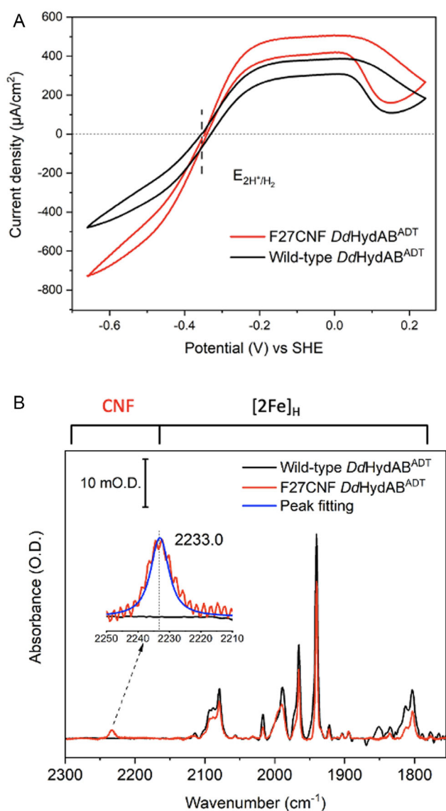
Figure 2. A) Cyclic voltammograms of WT DdHydAB ADT and F27CNF DdHydAB ADT , adsorbed onto a pyrolytic graphite electrode. Conditions: buffer mix pH 6, 2000 rpm, 1000 \text{ mL min}^{-1} \text{H}_2 , and scan rate 20 \text{ mV s}^{-1} . B) Transmission-mode IR spectra WT DdHydAB ADT (1 mM) and F27CNF DdHydAB ADT (1.5 mM). Conditions: 100 mM Tris-HCl buffer + 150 mM NaCl pH 8, 25 °C, 1 \text{ cm}^{-1} resolution, and 1024 co-averaged scans.
