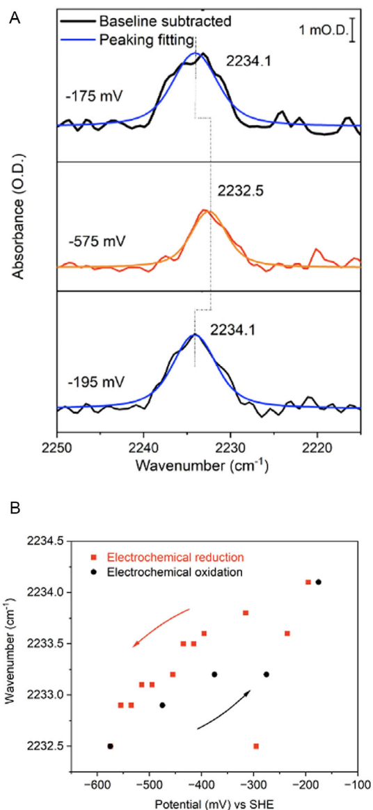
Figure 4. A) IR spectroelectrochemistry of F27CNF apo- DdHydAB . Spectra were recorded in a reflection-absorption cell. Conditions: 1.5 mM F27CNF apo- DdHydAB in 100 mM Tris-HCl + 150 mM NaCl pH 8 buffer containing redox mediators (see Supporting Information, Experimental Section), with peak fitting according to a Voigt profile; 1 cm -1 resolution, and 1024 co-averaged scans. B) NC stretching band of CNF versus applied potential. The red dots represent titration in a reductive direction, and the black dots represent return titration series in an oxidative direction.
