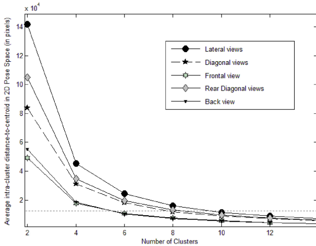
Fig. 16 Class Definition for MoBo dataset: For each training view, the 2D pose space is clustered and for each number of clusters, the intra-cluster distances to centroid are computed. By selecting a thresholding value of this average intra-cluster distance, the views are quantized into a number of classes that reflect the variability in appearance for that view. For the selected threshold (dashed line), frontal views of walking have a coarser quantization (6 classes) compared to the diagonal (8 classes) and lateral views (10 classes).
