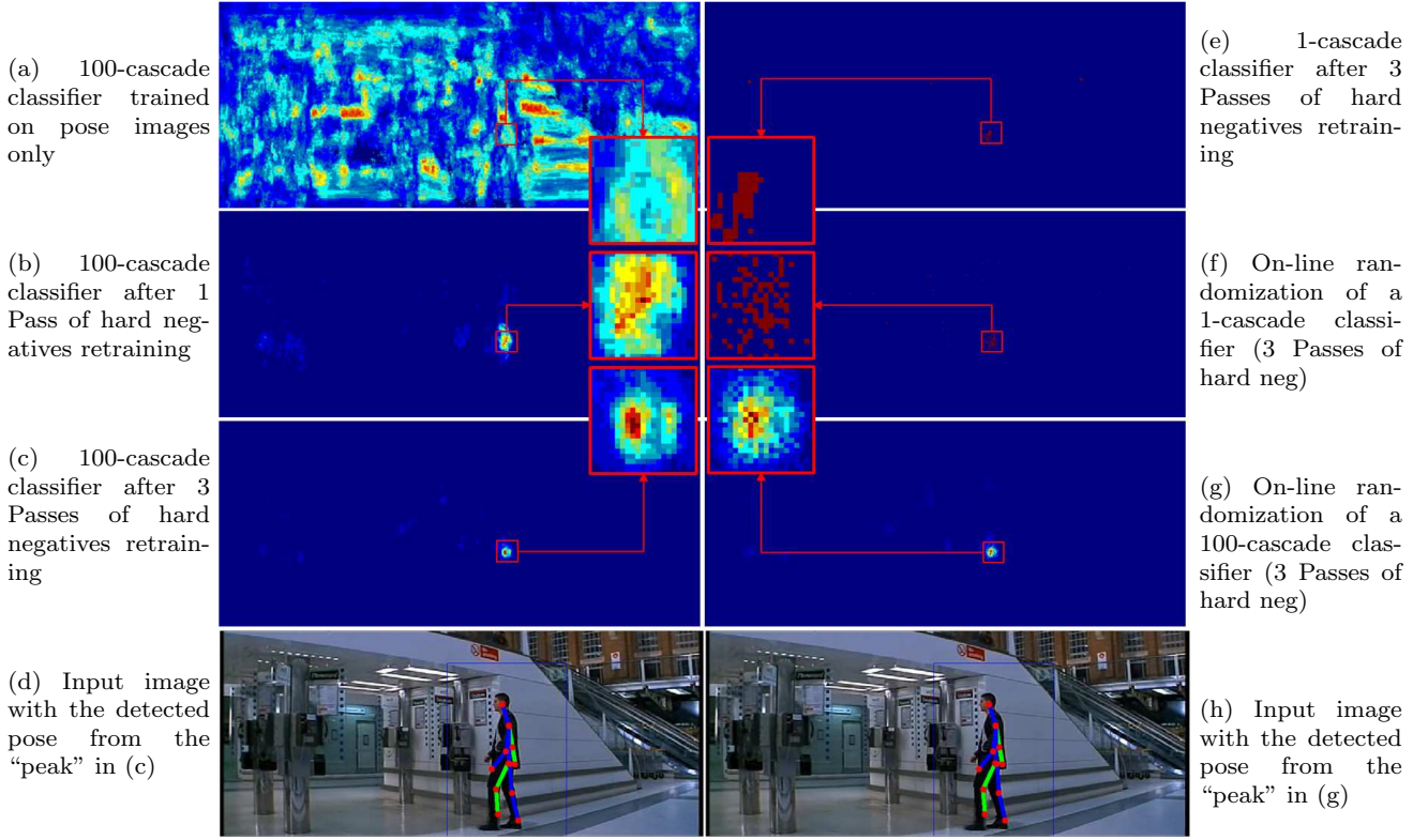
Fig. 8 Cascade classifier response for a dense scan. Left side, from top to down: saliency map \mathcal{M} after 0 (a), 1 (b) and 3 (c) passes of hard negatives retraining (i.e. adding hard negative examples in the cascade learning process). For visualization purpose we represent \mathcal{M} for ground truth scale (i.e. s = 0.6 ) and show a zoom around the ground truth location. (d) input image with the pose corresponding to the peak in (c). Right side, from top to down: saliency map \mathcal{M} obtained with a 1-cascade (e), 1 cascade randomized on-line (f), a 100-cascade ensemble randomized on-line (g). In (h) we show the pose corresponding to the peak in (g).
