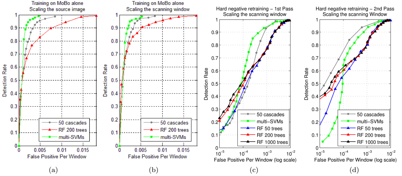
Fig. 22 Detection results on the combined localization dataset using different classifiers trained on Mobo images only (a and b), trained with a first pass of hard negatives from INRIA (c) and with a second pass (d). For the 1 st case, we present results for 2 different types of multi-scales scanning scheme: scaling the input image and keeping the size of the scanning windows fixed (a) and scaling the scanning window and keeping the size of the input image fixed (b), while the other 2 graphs (c and d) are obtained with the second scanning scheme. Note that a log scale is used for c and d to aid visualization.
