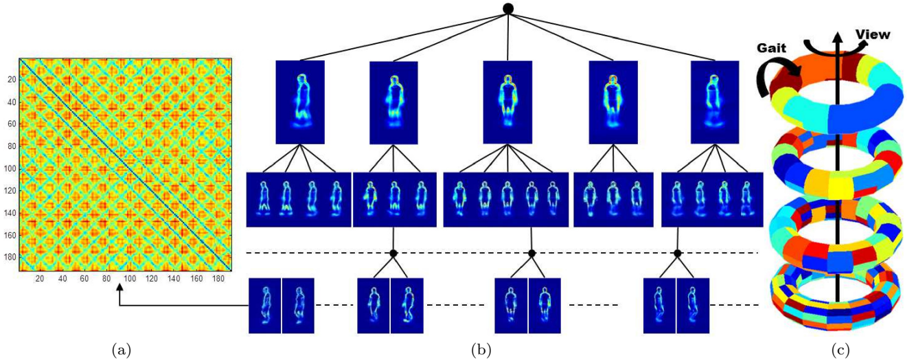
Fig. 4 Bottom-up hierarchical tree construction: the structure \mathcal{S} is built using a bottom-up approach by recursively clustering and merging the classes at each level. We present an example of tree construction from 192 classes (see class definition in Sect. 4.1.2) on a torus manifold where the dimensions represent gait cycle and camera viewpoint. The matrix presented here (a) is built from the initial 192 classes and used to merge the classes at the very lowest level of the tree. The similarity matrix is then recomputed at each level of the tree with the resulting new classes. The resulting hierarchical tree-like structure \mathcal{S} is shown in (b) while the merging process on the torus manifold is depicted in (c). We can observe (b) how the first initial node acts as a viewpoint classifier.
