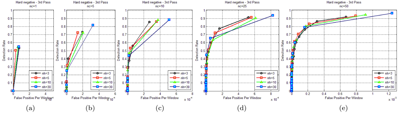
Fig. 24 Detection results for different configurations of the cascades classifiers with a 3^{rd} pass of hard negative retraining: we present the results with respectively 1 (a), 5 (b), 10 (c), 25 (d) and 50 cascades (e). For each case we vary the number n_h of HOG blocks we sample from at each branch of the tree. The corresponding classification times are shown in Fig. 26.
