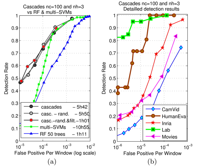
Fig. 29 Best Cascade Classifier - Results: detection rate of the selected cascade classifier (100 cascades filtered with the first 5 cascades) compared to other classifiers for a 4-pixels search stride (a) and corresponding detailed detection rates over the 5 different types of images in our localization dataset (b).
