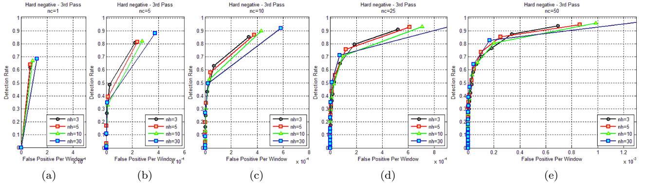
Fig. 25 Detection results for different configurations of the cascades classifiers with a 3^{rd} pass of hard negative retraining and on-line randomization: we present the results with respectively 1 (a), 5 (b), 10 (c), 25 (d) and 50 cascades (e). For each case we vary the number n_h of HOG blocks we sample from at each branch of the tree.
