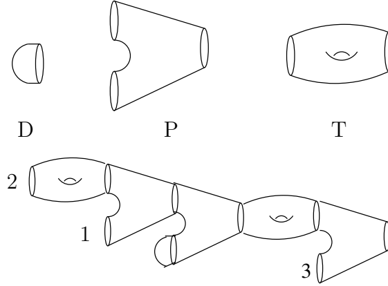
Figure 3.1: Basic surfaces
