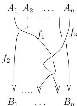
Figure 1.7: Arrow in \mathfrak{B}\mathcal{f}\mathcal{A}
