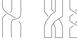
Figure 1.3: Braid and ribbon
