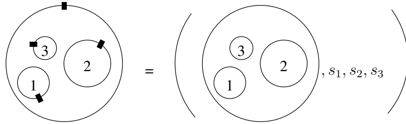
Figure 1.4: Element of f\mathcal{D}_2(3) = \mathcal{D}_2(3) \times (S^1)^3
