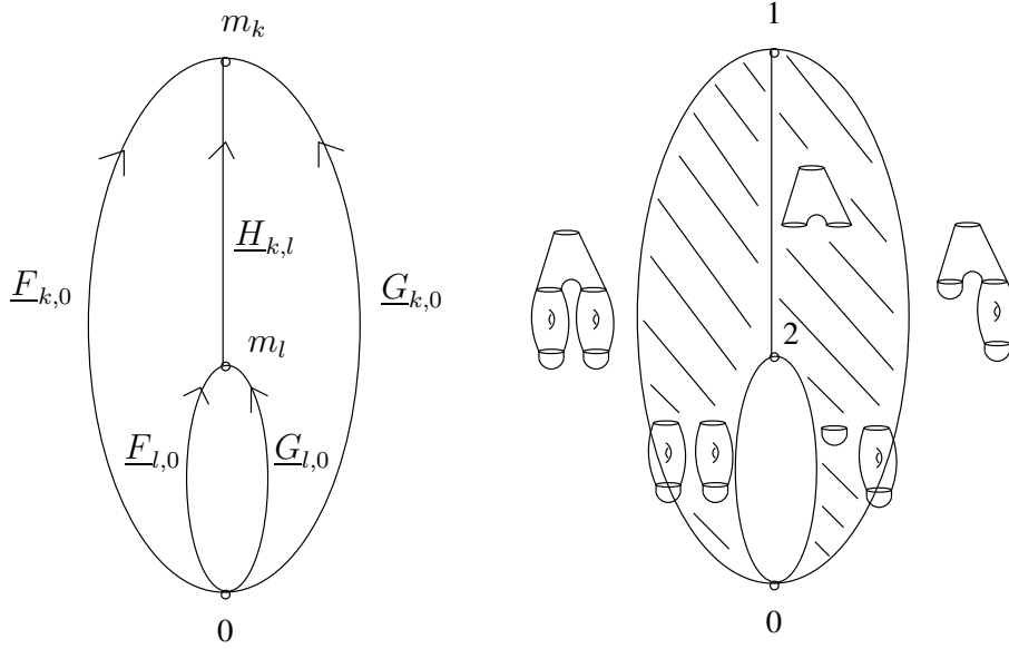
Figure 3.4: Homotopy H_{k,l}
