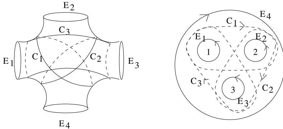
Figure 2.1: Lantern relation
