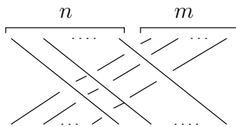
Figure 1.6: Braiding b_{n,m} of \mathfrak{B}
