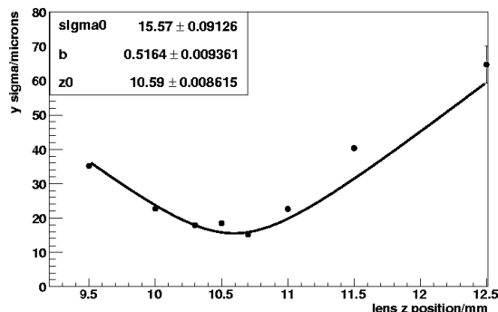
Figure 4: Scan of the laser-waist position by stepping the final focus lens along the laser-beam direction.
