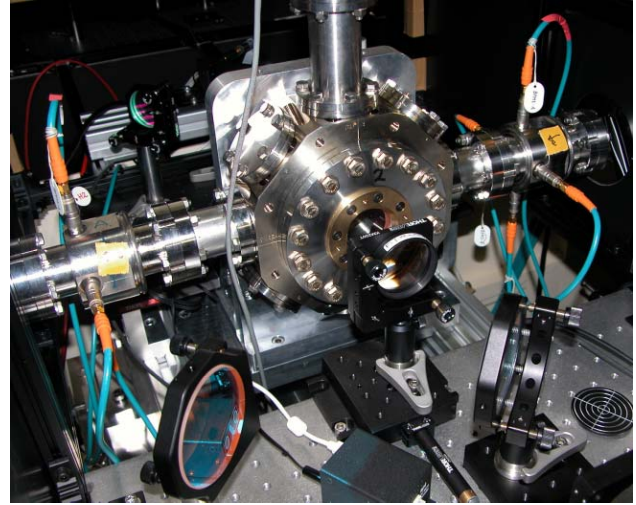
Figure 2: Photograph of the LW vacuum chamber in-situ. Note the two strip-line BPMs, the insertion device for the knife edge (top) and the re-collimation optics.
