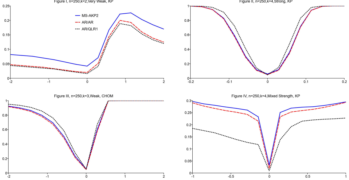
Figure 1: Power of various subvector tests in different cases. Covariance structure: Kronecker product (KP); CHOM. Identification strength (\pi_W, \pi_Y) : Very Weak (2, 2); Weak (4, 4); Strong (40, 40); Mixed strength: (2, 40).
