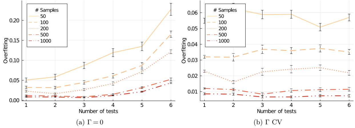
Figure EC8 Overfitting (relative difference between in-sample and out-of-sample AUC) as the number of tests K increases, for the non-robust (left) and robust (right) policy, on synthetic data without any missing entries, for varying sample size N . Results are averaged over 50 random training sets.
