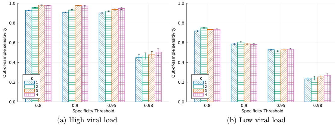
Figure EC7 Best achievable sensitivity for a K -test combination of antigen tests, for different target specificity levels, for high- and low- viral load patients respectively.
