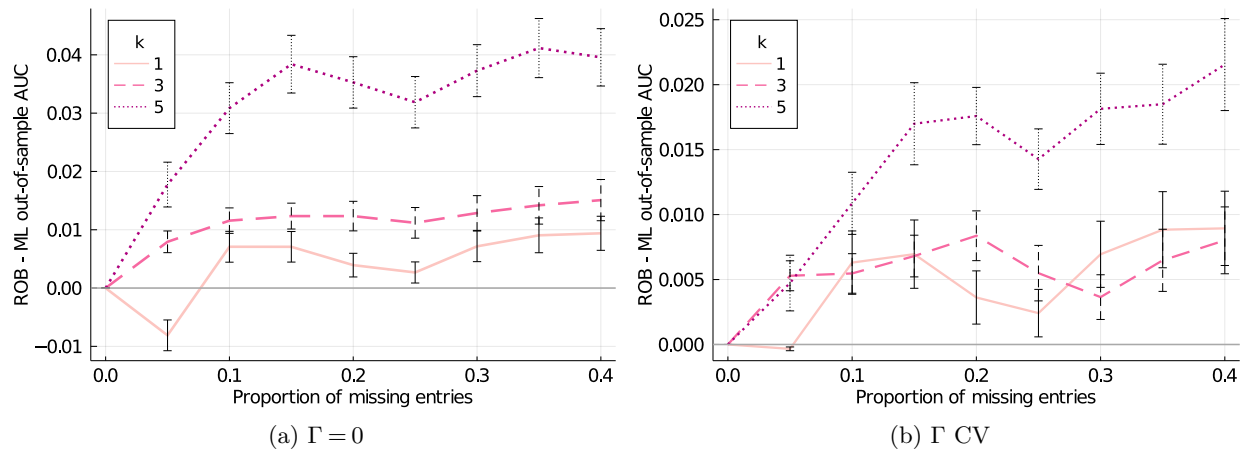
Figure EC10 Absolute difference in out-of-sample AUC between robust (ROB) and maximum likelihood (ML) imputation as the proportion of missing entries increases, for the non-robust (left) and robust (right) policy, on synthetic data with N^+ + N^- = 200 . Results are averaged over 50 random training sets.
