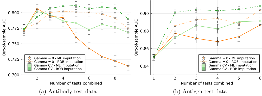
Figure 4 Out-of-sample accuracy (AUC) as a function of the imputation method for missing data.
