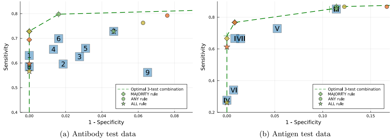
Figure EC3 Performance of the majority (diamond), any (circle) and all (star) rules on a subset of 3 tests selected that achieve highest individual AUC (orange), are cherry-picked to lie on the frontier (yellow), or achieve the highest AUC when combined (green).
