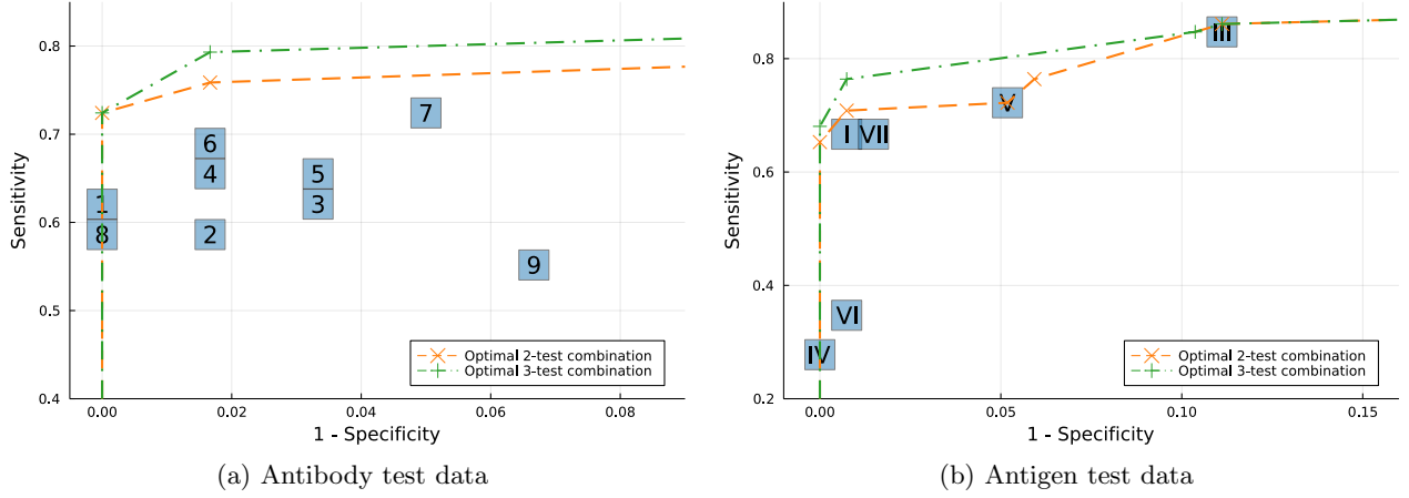
Figure 2 The trade-off between specificity and sensitivity (ROC curve) for all the individual tests and the optimal combinations of 2 (orange line) and 3 tests (green line).
