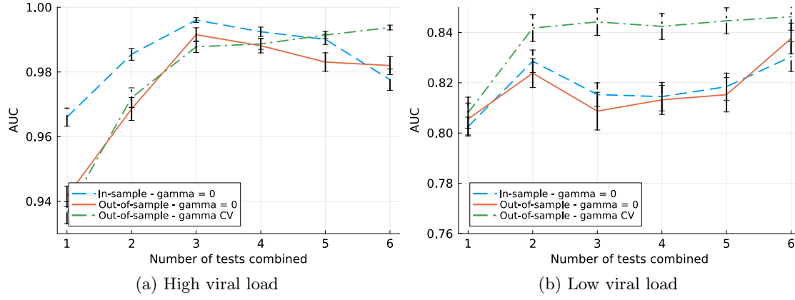
Figure EC6 Diagnostic accuracy (AUC) of the best K -test combination of antigen test, as K increases, for high- and low- viral load patients respectively.
