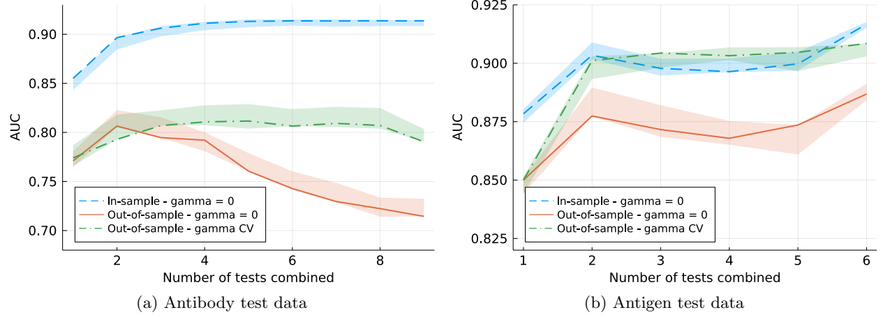
Figure EC1 Robustness of the AUC of the best combination of K tests to the training/validation proportion, as the number of tests K increases, for the non-robust combination policy (in-sample in dash blue, out-of-sample in solid orange) and the robust policies with cross-validated \gamma (dash-dot green).
