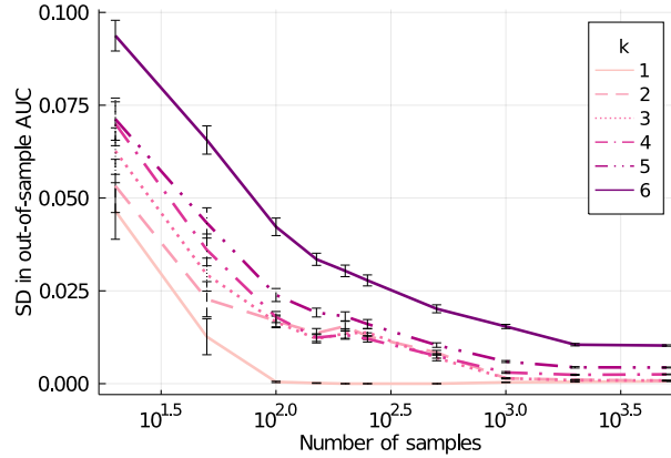
Figure EC9 Standard deviation (SD) in out-of-sample AUC between models with \Gamma \in \{0, \dots, 10\} as the number of samples increases, for different values of K . Results are averaged over 50 random training sets.
