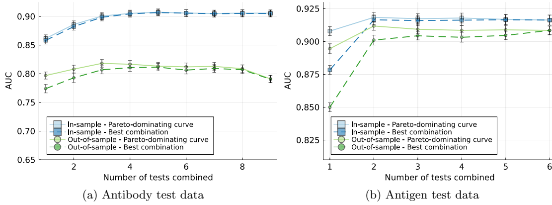
Figure EC2 Comparison of the diagnosis accuracy (AUC) of the best combination of K tests and the entire Pareto-dominating curve as a function of the number of tests K combined.
