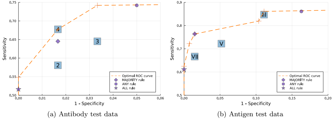
Figure 1 The trade-off between specificity and sensitivity (ROC curve) for 3 individual tests and all their potential combinations.
