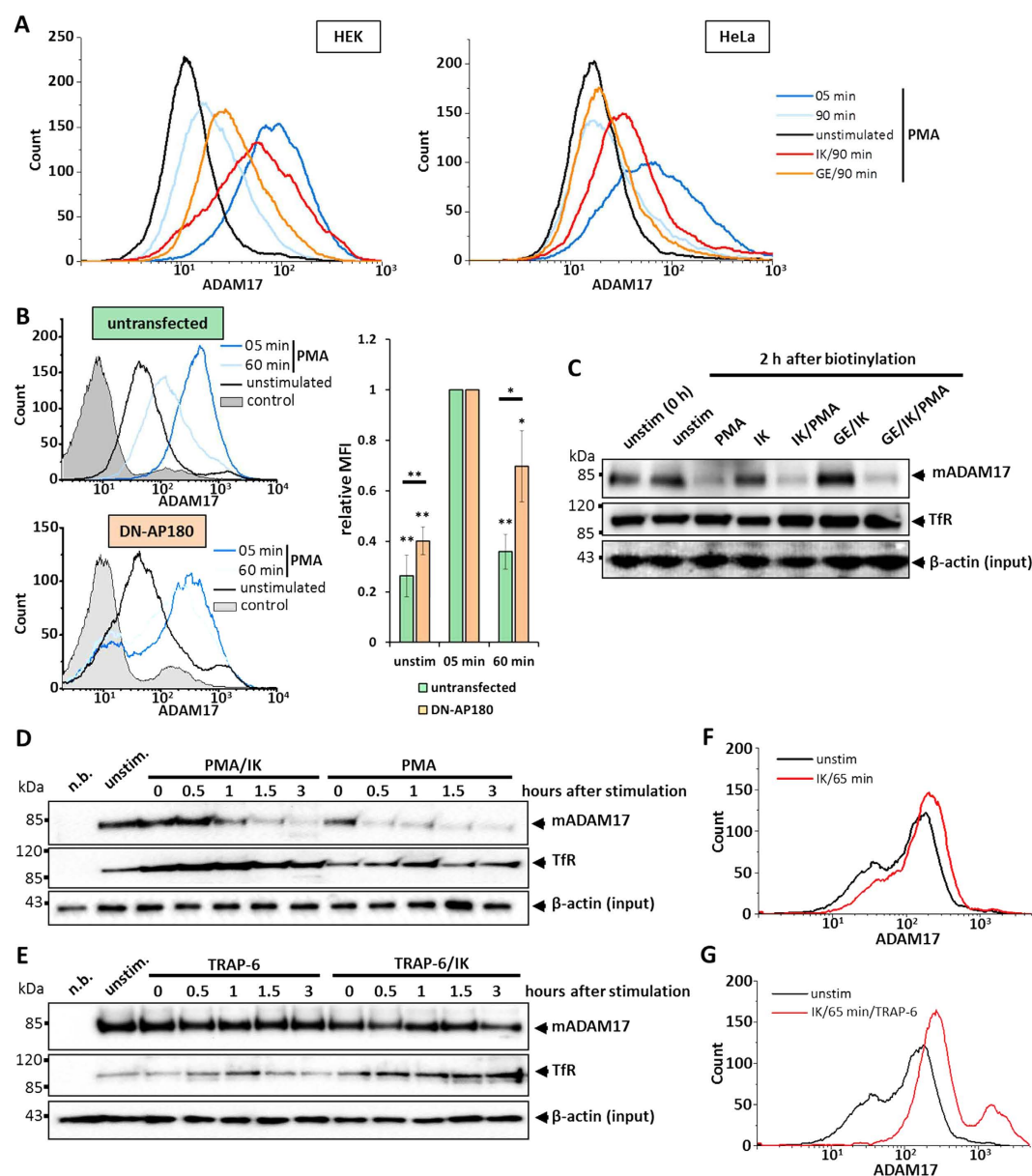
Figure 4. Inhibition of ADAM17 internalisation. (A–G) As inhibitor against the clathrin-dependent internalisation 5 \mu M ikarugamycin (IK) were used. To inhibit caveolin-dependent internalisation cells were treated with 200 \mu M genistein (GE). Each depicted flow cytometry graph is one representative experiment of a set of n = 3 . (A) Flow-cytometry analysis of HEK293 and HeLa cells, which were left unstimulated, were stimulated with 100 nM PMA or were stimulated with 100 nM PMA and treated either with genistein or with ikarugamycin 1 hour before stimulation. (B) HEK293 cells were left untransfected or were transfected with DN-AP180_BFP2. Afterwards, cells were stimulated with PMA for 5 minutes or 60 minutes, or left unstimulated and harvested for flow cytometry analysis. Each depicted flow cytometry graph is one representative experiment of a set of n = 4 . Right panel: Comparison of relative MFI (median fluorescence intensity) between untransfected and with DN-AP180 transfected cells. The MFIs were normalised to the respective 5 minutes stimulated sample. (C) Pulse chase experiments: HEK293 cells were incubated with inhibitors like described before. After 1 hour surface proteins were biotinylated and cells were immediately harvested (unstim (0 h)), or were stimulated with 100 nM PMA or left unstimulated in addition to the indicated treatment with inhibitors for 2 hours. The lysates, which were used for the Streptavidin-Sepharose precipitation were immunoblotted as additional input control. (D,E) Western blots of cell-surface fractions of HEK293 cells, which were either left unstimulated, stimulated with 100 nM PMA (D) or stimulated with 30 \mu M TRAP-6 (E). An additional set of cells were treated with ikarugamycin and were stimulated like described before 1 hour after treatment with the inhibitor. Cell-surface proteins were biotinylated at given time points after stimulation. The lysates, which were used for the Streptavidin-Sepharose precipitation were immunoblotted as additional input control. (F) Flow-cytometry analysis of HEK293 cells, which were left unstimulated and were treated with ikarugamycin for indicated times. (G) Flow-cytometry analysis of HEK293 cells, which were treated with ikarugamycin for 60-minute prior stimulation. Cells were analysed 5 minutes after stimulation with 30 \mu M TRAP-6.
