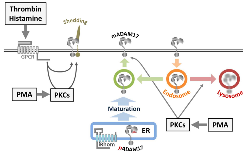
Figure 6. Model of the ADAM17 life cycle. ADAM17 exists as immature proform (pADAM17) and as mature protease (mADAM17) in cells. After ADAM17 is translated into the ER, it travels iRhom-dependent to the Golgi apparatus, where the maturation takes place. This process seems to be a tightly regulate bottleneck in the life cycle of ADAM17 dividing a big pool of immature from a smaller pool of mature molecules. Most of the mature ADAM17 seems to be intracellularly located whilst only a small amount is actually at the cell surface, where shedding can take place. Stimulation with physiological stimulators of ADAM17-mediated shedding such as Thrombin or Histamine does not alter the amount of cell surface ADAM17 or the overall amount of mature ADAM17 in the cell. Most recently it was shown, that most of the mature ADAM17 at the cell surface is internalised and recycled. The non-physiological PKC-activator PMA does not only activate ADAM17-mediated shedding but does also drastically dysregulate the localisation of mature ADAM17. PMA leads to a fast increase in surface expression followed by internalisation and lysosomal degradation of ADAM17. The activation of this path eventually empties the pool of mature ADAM17 within a few hours without affecting the pool of immature ADAM17.
