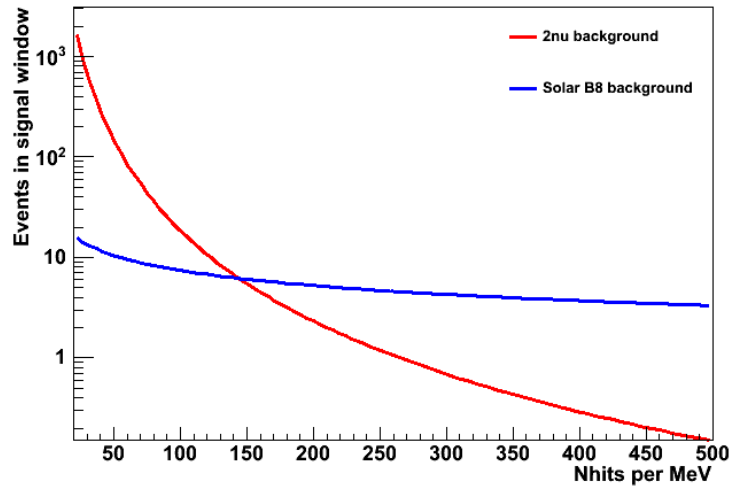
Figure A.1: Relative rate of events from the ^{130}\text{Te} 2\nu background and solar ^8\text{B} backgrounds reconstructing in the energy window at different assumed light levels, given in nhits per MeV.
