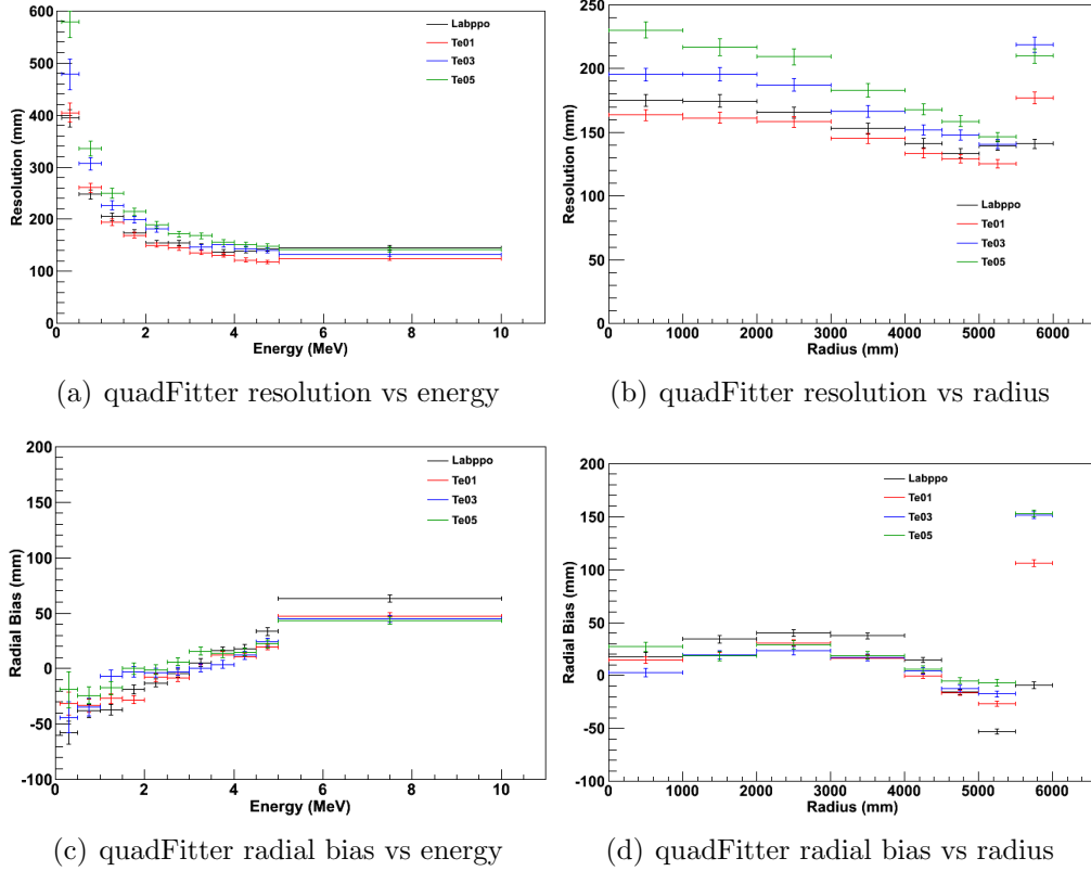
Figure 5.9: The resolution and radial bias of the quadFitter at different energies and radii, generated by simulating electron events for a detector filled with unloaded scintillator and 0.1, 0.3 and 0.5% Type-B Te-loaded scintillator. The energy events are simulated for events filling the detector for 11 different energy bins while the radial events are simulated at 3 MeV in 8 different radial bins.
