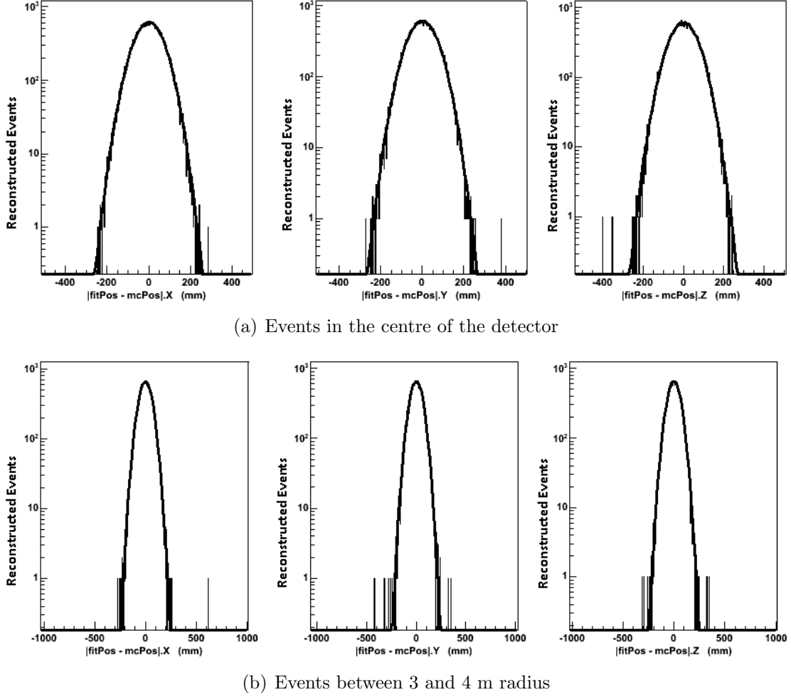
Figure 5.21: The difference between fitted and Monte-Carlo positions for the x, y, z components and the distance between the fitted and Monte-Carlo positions generated for 50,000 events fit using the likelihood fitter in a) the centre of the detector and b) between 3 and 4 m radius.
