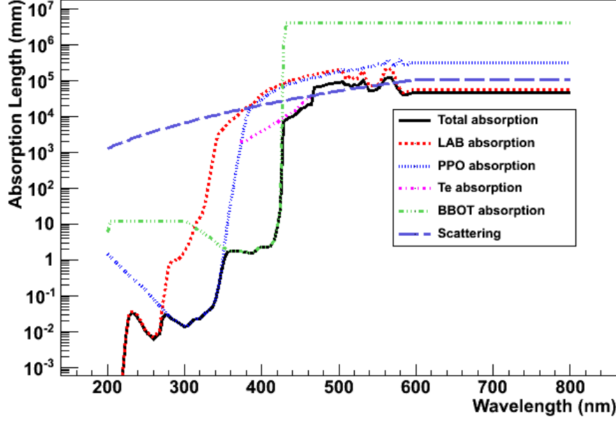
(a) Total absorption for Type B Te-loaded scintillator (at 0.1% loading) with BBOT as a secondary WLS)
