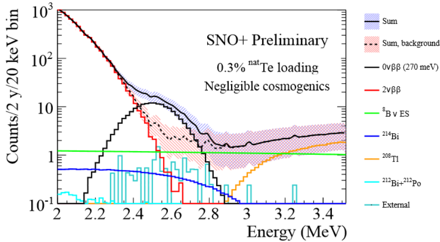
Figure 1.5: Expected signal and backgrounds for 0\nu\beta\beta in SNO+ assuming 0.3% loading of tellurium, after two years of data taking[45]. Error bands represent statistical errors (Poisson) at 68% CL.
