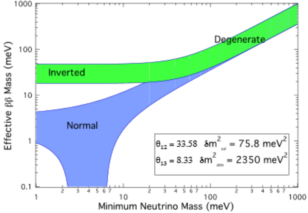
Figure 1.2: Effective Majorana mass as a function of the lightest neutrino mass for the normal and inverted mass hierarchys. Effective Majorana mass is defined as a sum of the three neutrino masses, m_{\beta\beta} = |\sum_{i=1}^3 m_i U_{ei}^2| . This figure is taken from[25].
