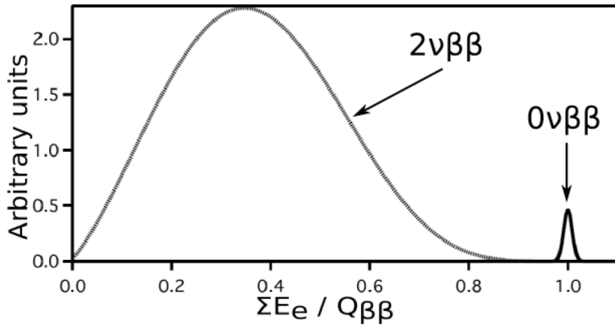
Figure 1.4: Generic energy spectrum showing the energy spectrum for 2\nu\beta\beta as well as the 0\nu\beta\beta peak[36].
