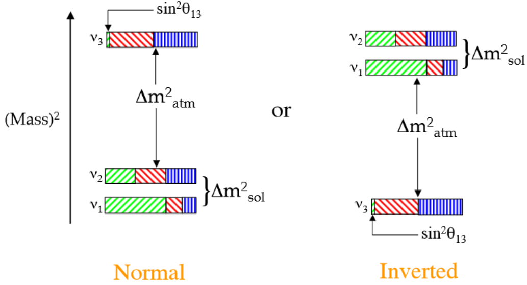
Figure 1.1: Possible neutrino mass orderings for a) the normal hierarchy and b) the inverted hierarchy. The electron, muon and tau fraction of each mass state is shown in the colours green, red and blue. This figure is taken from[24].
