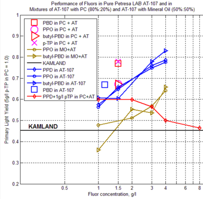
Figure 4.1: Measured light yield of the scintillator with various fluor concentrations based on measurements at Queens[74]. The light yields used in this study were the blue circles which give the change in light yield for LAB (AT-107) with different PPO concentrations.
