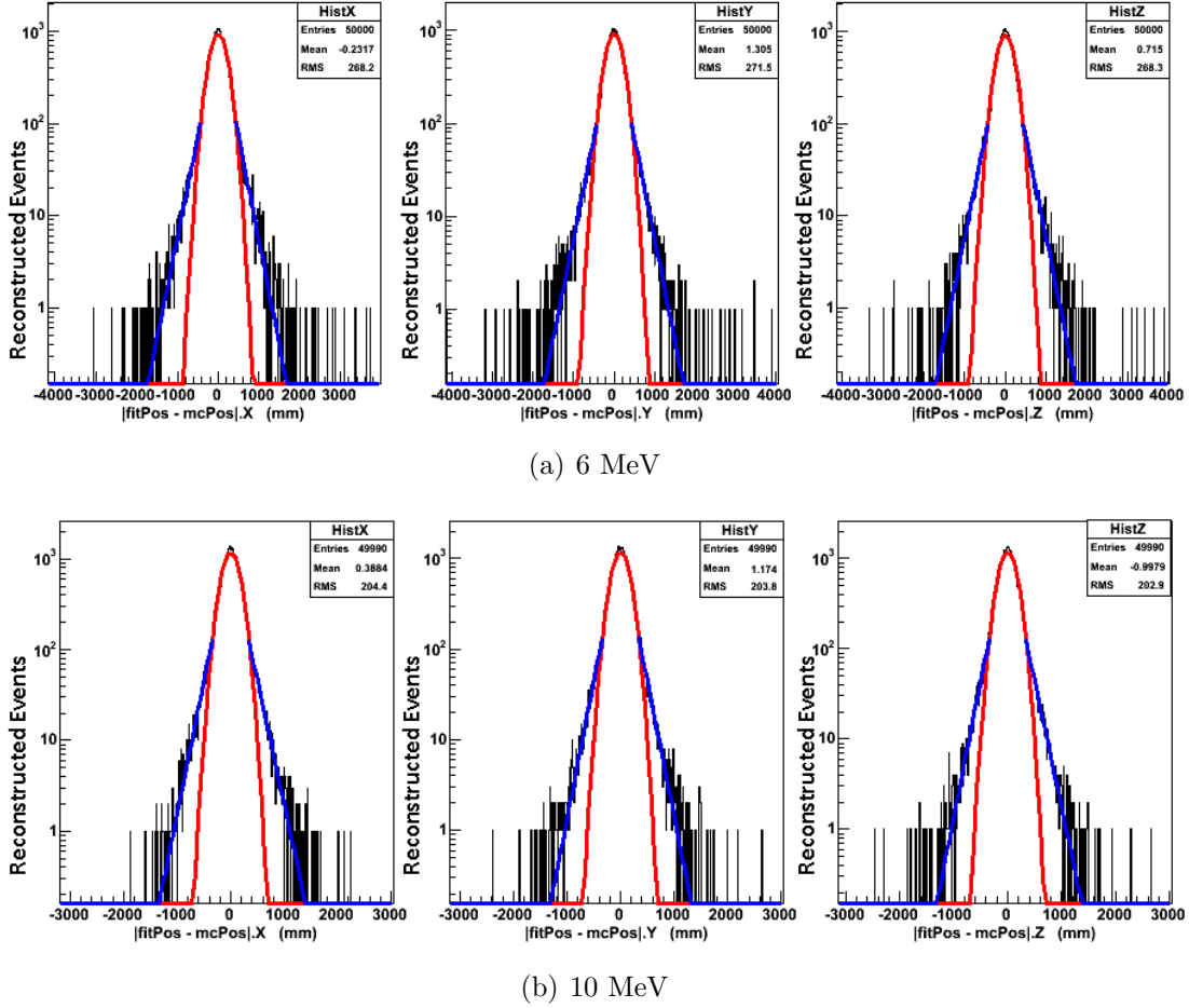
Figure 7.2: The difference between fitted and Monte-Carlo positions for the x, y, z components and the distance between the fitted and Monte-Carlo positions generated for 50,000 events at the centre of the detector fit using the waterFitter at a) 6 MeV and b) 10 MeV.
