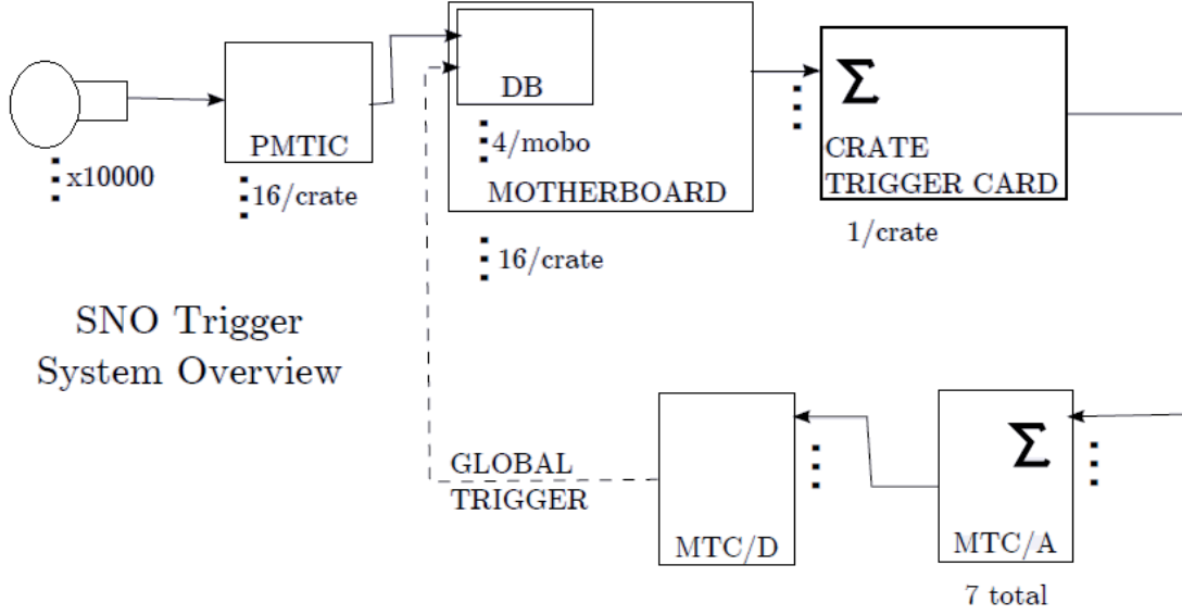
Figure 2.2: Diagram showing the SNO+ trigger system, adapted from[57]. The output of the PMT is read out by the PMT Interface card (PMTIC) and passed to the daughterboard (DB) which calculates timing and charge which is then read out by the front end card (FEC). The crate trigger card (CTC) sums the triggers for a particular crate and passes this to the analogue master trigger (MTCA) which combines this information for all crates. The digital master trigger card (MTCD) compares this to the trigger thresholds to decide whether a global trigger is issued.
