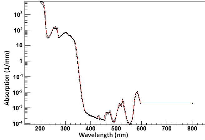
Figure 3.4: Effect of changing the bin size from 10 nm (black) to 4 nm (red) on the total absorption for Nd-loaded scintillator.
