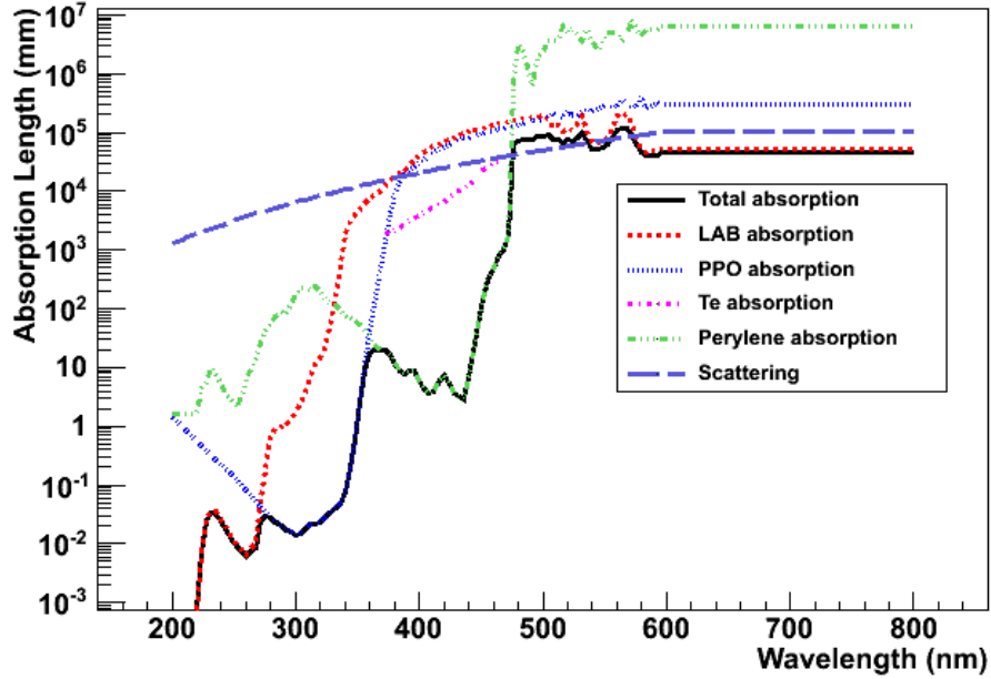
(b) Total absorption for Type B Te-loaded scintillator (at 0.1% loading) with perylene as a secondary WLS
