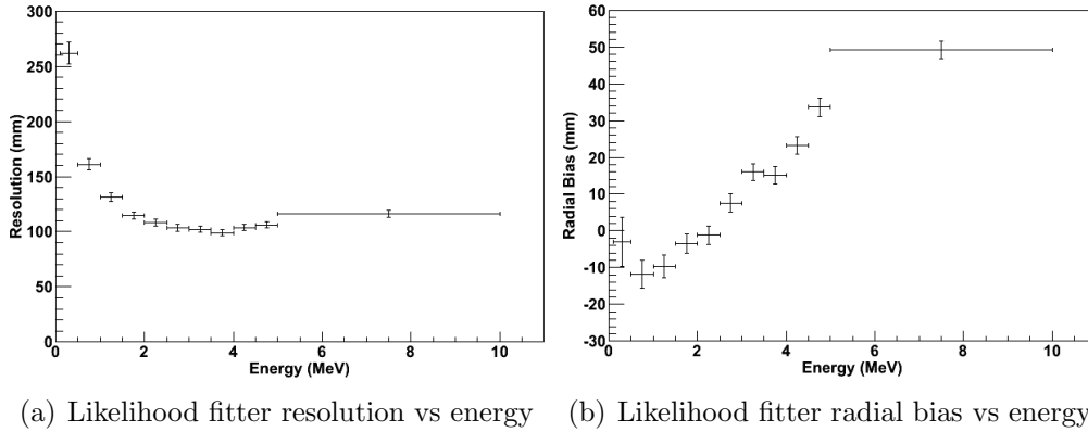
Figure 5.16: The resolution and radial bias of the likelihood fitter for electron events generated in unloaded scintillator at 0.1 to 10 MeV, spread evenly through the detector with a fiducial volume of 5.5 m.
