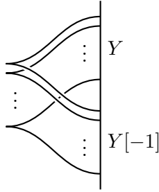
Figure 3.1: The tangle \beta_Y .
