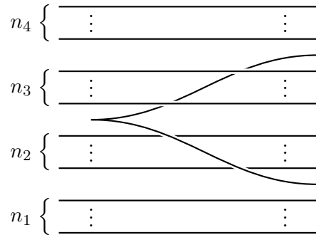
Figure 3.2: A tangle with a single left cusp and n_2 + n_3 crossings.
