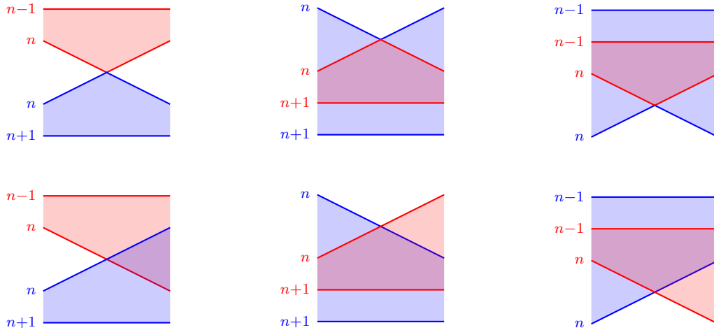
Figure 3.3: Switches (top row) and departures (bottom row). Returns are departures reflected on the vertical axis.
