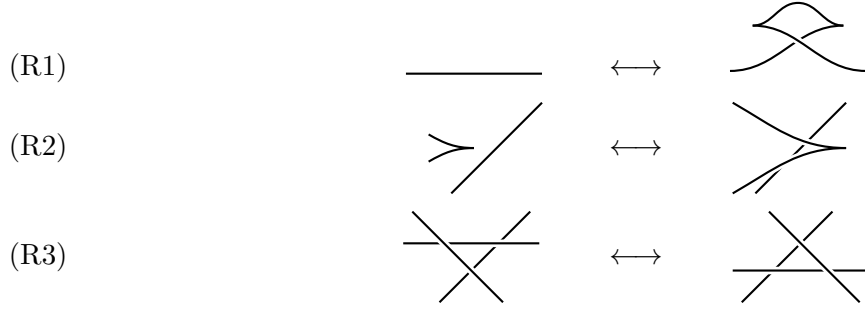
Figure 3.4: Legendrian Reidemeister moves
