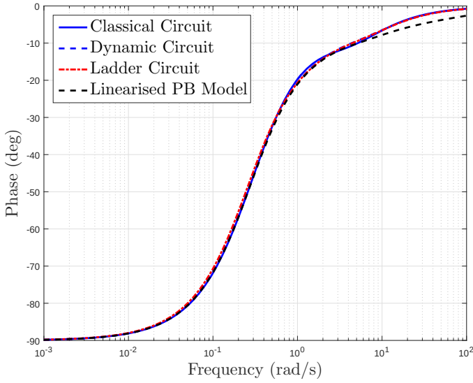
(b) Phase of G(s) .
