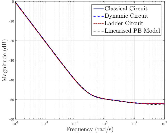
(a) Magnitude of G(s) .
