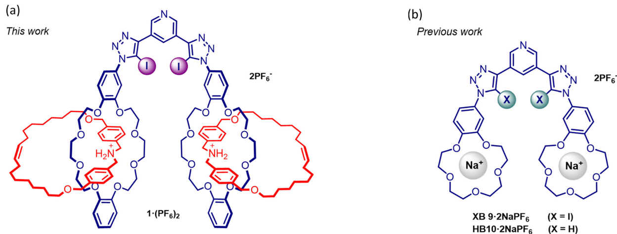
Fig. 1 Chemical structures of (a) ammonium-dibenzo[24]crown-8 [2]catenane functionalised XB receptor, 1 -(PF 6 ) 2 and (b) XB and HB heteroditopic benzo-15-crown appended analogous receptors containing sodium ion complexed benzo[15]crown-5, XB9-2NaPF 6 and HB10-2NaPF 6 , respectively.
