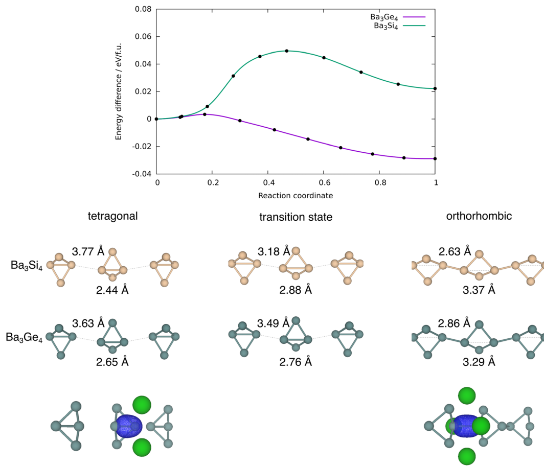
Fig. 3 Potential energy curve (optB86b- vdW ) for the concerted phase transition from the tetragonal to the orthorhombic phase in Ba 3 Ge 4 and Ba 3 Si 4 . Maximally localised Wannier functions corresponding to the intra- and inter-molecular bonds of the tetragonal and orthorhombic phases, respectively, are also shown.
