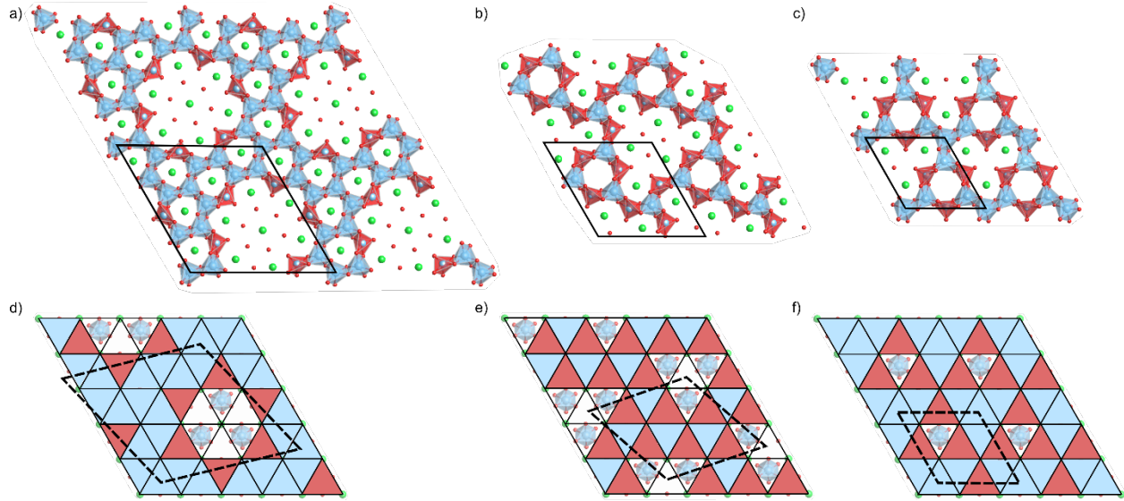
FIG. 5. (a) Diagram of RT13b, (b) RT7b, and (c) (2 \times 2)a where \text{TiO}_5 octahedra are red, \text{TiO}_6 octahedra blue, and Sr atoms are green. (d) Grid imposed on bulk \text{SrTiO}_3 (111) to codify RT13b, (e) RT7b, and (f) (2 \times 2)a .
