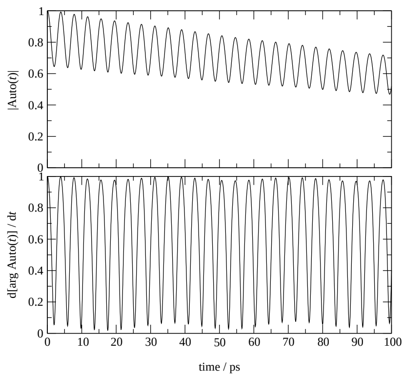
Figure 7.9: Autocorrelation function and the time derivative of phase of autocorrelation function evaluated at 119.5 \text{ cm}^{-1} below threshold for the hydrogenic system shown in Fig. 7.6.
