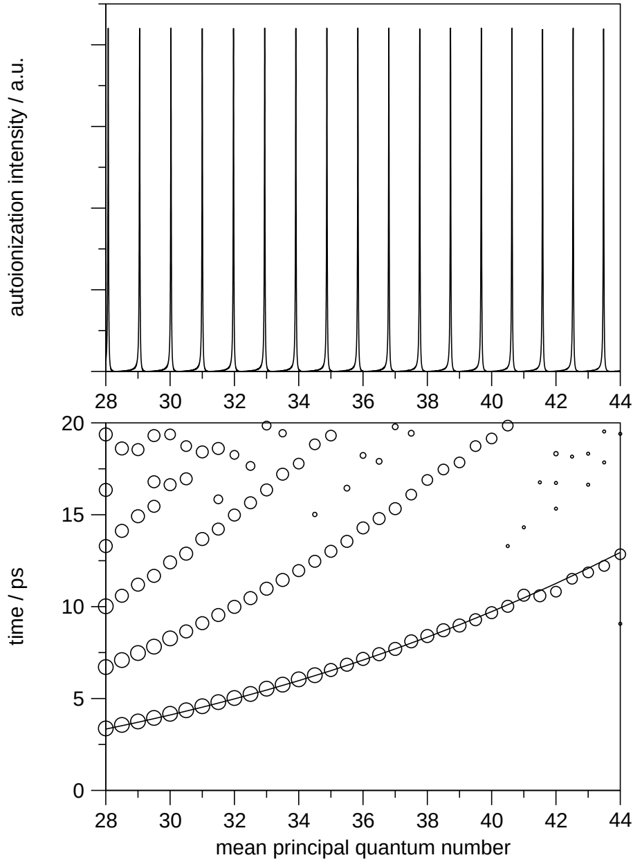
Figure 7.6: Above: Hydrogenic spectrum for a four-channel system where \Delta\mu = 0 plotted against principal quantum number. Below: ( \circ ) Plot of times of peaks of autocorrelation functions plotted against mean principal quantum number. The size of the circle is proportional to the height of the peak. (Solid line) Kepler recurrence time.
