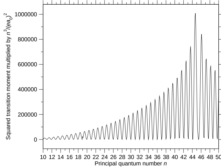
Figure 2.6: Plot of the 45.4f \rightarrow ng transition moment squared and scaled by \Delta n^3 against n . The zero at n = 45.4 is where \Delta n = 0 ; the transition moment reaches a maximum there.
