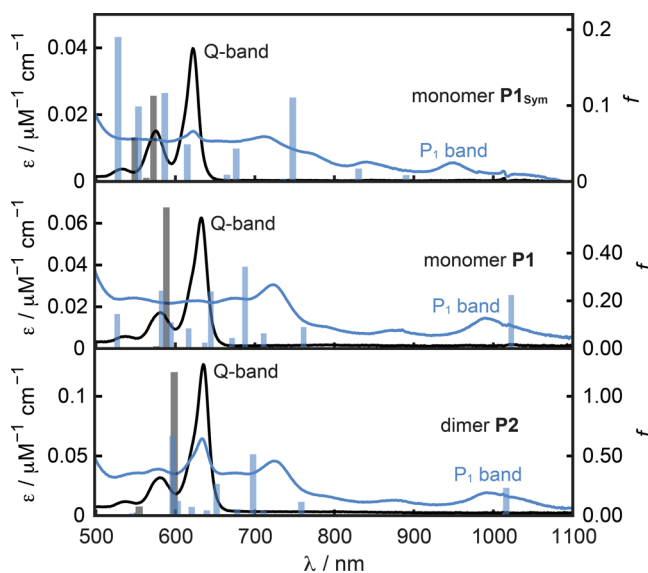
Figure 2. Steady-state UV–vis–NIR absorption spectra of neutral (black) and oxidized (blue) P1 sym , P1 , and P2 in CHCl 3 (298 K). The absorption spectra of the radical cations P1 sym •+ , P1 •+ , and P2 •+ were obtained by oxidation with one equivalent of BAHA (see SI Figure S27 for the full oxidation titrations). The vertical bars indicate the TD-DFT (LC- \omega PBE/6-31G*; \omega = 0.1 ) calculated wavelengths and oscillator strengths, f , for the electronic transitions of the neutral and oxidized compounds in the absence of vibronic coupling.
