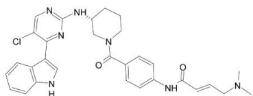
THZ531 (CDK12/13 selective)
