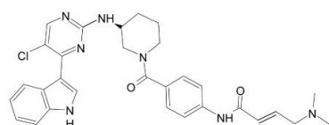
THZ532 (control isomer 50-100 fold weaker against CDK12/13)
