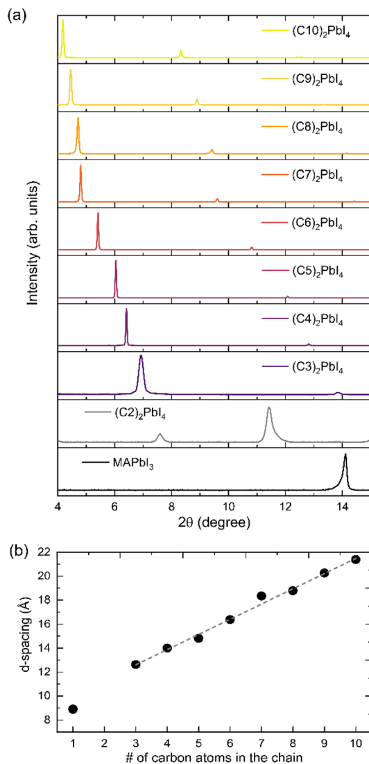
Fig. 1 Structural analysis of the perovskite films. (a) XRD patterns of 2D perovskite and MAPbI 3 with different A-site cations in the range of 2\theta from 4^\circ to 15^\circ . A wider region is shown in Fig. S5 in the ESI.† (b) Extracted relationship between the number of the carbon atoms in the spacer cation and the resulting d -spacing of the perovskite film; note that the C1 sample corresponds to the 3D perovskite MAPbI 3 .
