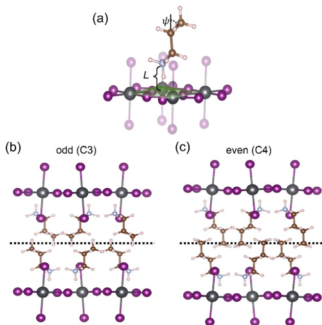
Fig. 5 DFT-derived structures of 2D perovskites. (a) Illustration of the vertical distance L of the \text{N-PbI}_x plane and the angle \psi between the horizontal plane and the tail of the ligands. Examples for packing of the organic ligands within the inorganic lattice for (b) odd and (c) even numbers of carbon atoms in the spacer cation.
