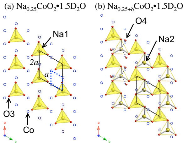
FIG. 3: (Color) Projections of the Na- \text{D}_2\text{O} layer down the c -axis. The \text{NaO}_6 triangular prisms centered on Na are highlighted. The 2a \times 2a \times c unit cell is shown in solid lines and the a \times a \times c cell as dashed lines. The doubling of the unit cell is evident from the position of the Na sites. D-atoms are omitted for clarity. (a) The idealized x = \frac{1}{3} structure. (b) A model for the x = \frac{1}{2} structure with the Na2 site filled. The coordination to the O4 site is shown.
