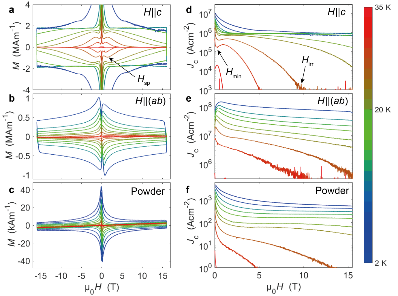
FIG. 3. The isothermal magnetization loops, M(H) , for the single crystal in two orientations with (a) H||c and (b) H||(ab) and (c) the powder sample of CaKFe_4As_4 . The critical current density, J_c , calculated from M(H) using the Bean model 20 , plotted as a function of magnetic field at constant temperatures for the single crystal (d) when H||c and (e) H||(ab) and (f) the powder sample, respectively. The arrows indicate the positions of H_{sp} in (a) and H_{irr} and H_{min} in (d).
