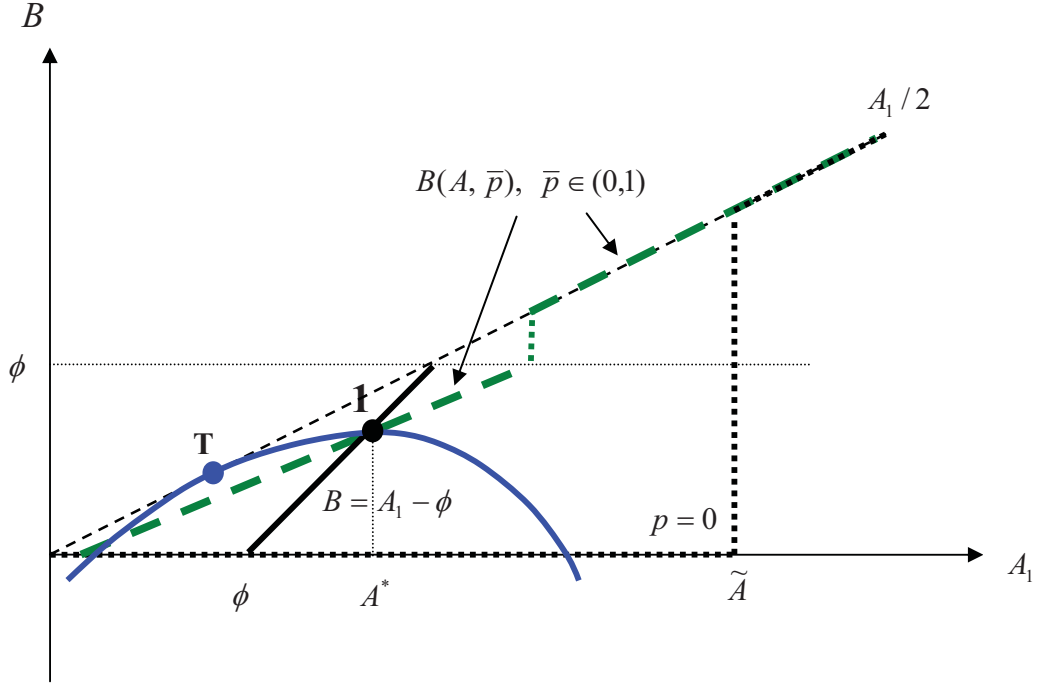
Figure 3. Pooling equilibrium
