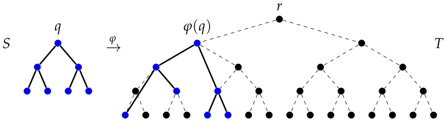
Fig. 1 A subdivision of S inside T . Edges of T are dashed for better visibility
