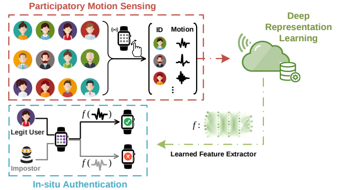
Figure 1: DeepAuth learns a deep feature extractor from crowd-sourced data, and protects legitimate users from unknown imposters on their smartwatches.
