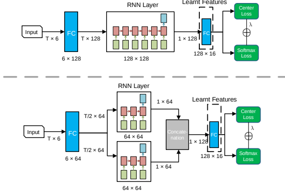
Figure 2: Deep neural network architecture with standard RNN layer (top) and the proposed sub-RNN layer (bottom).
