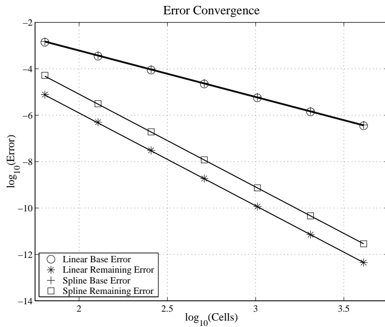
Figure 7: Error convergence for quasi-1D shock-free transonic flow.
