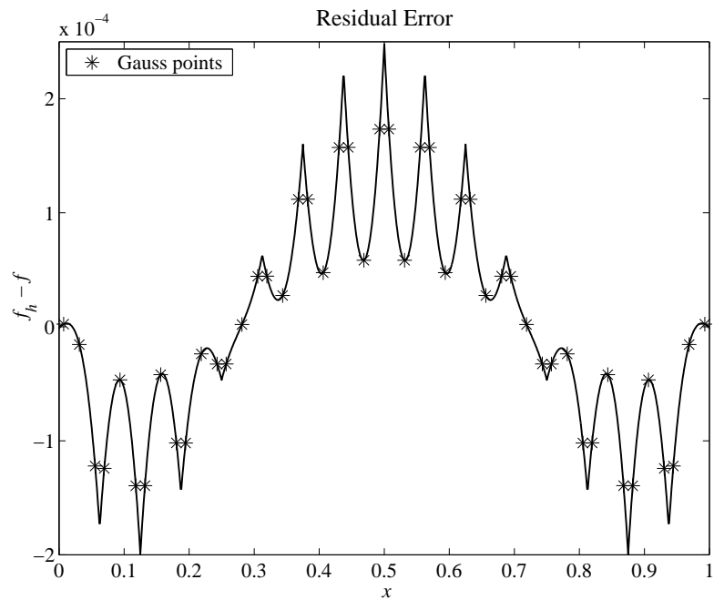
Figure 1: Residual error for a 1D Poisson problem.
