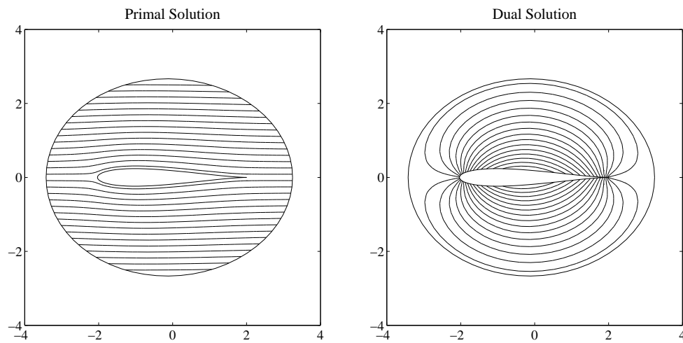
Figure 3: The primal and dual solutions for a 2D Laplace problem around a Joukowski airfoil with a cusped trailing edge.
