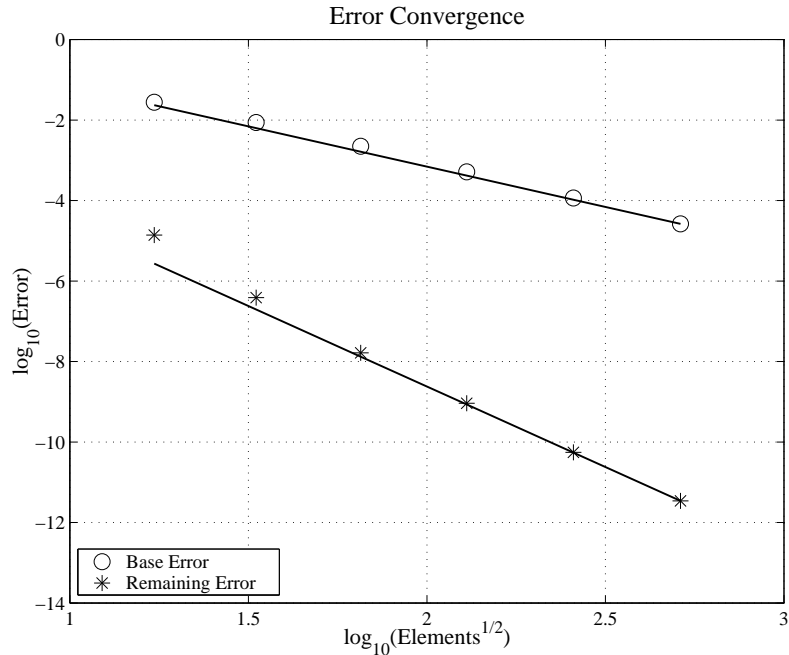
Figure 9: Error convergence of a boundary functional for a 2D nonlinear thermal diffusion problem.
