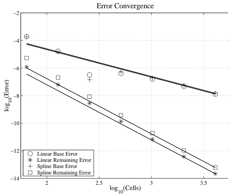
Figure 6: Error convergence for quasi-1D subsonic flow.
