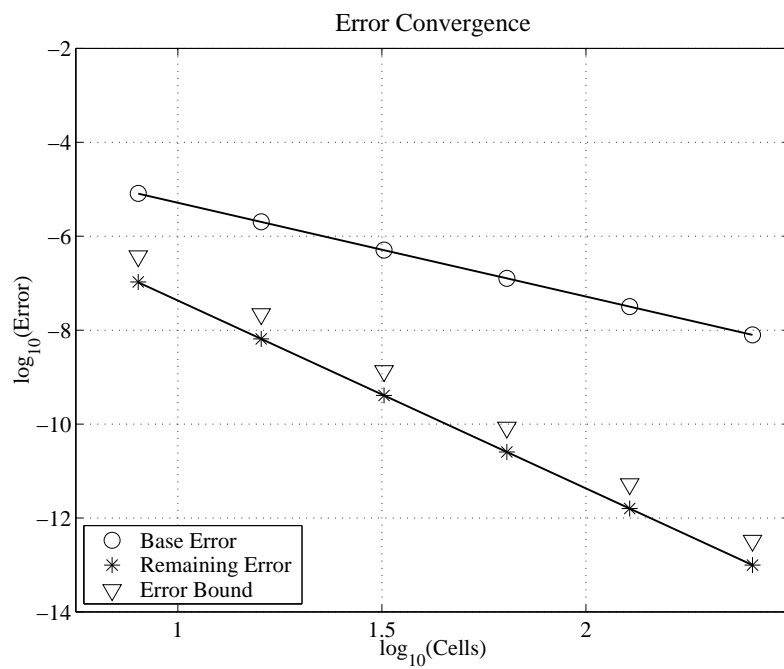
Figure 2: Functional error convergence for a 1D Poisson problem.
