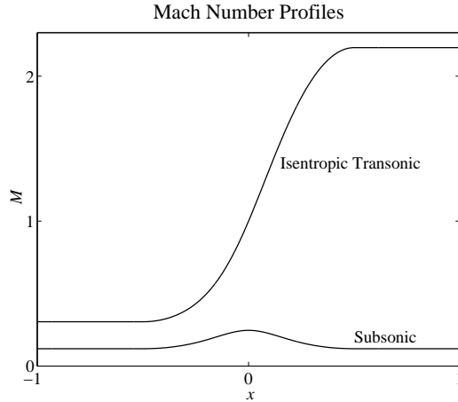
Figure 5: Mach number profiles for quasi-1D Euler equation test cases.
