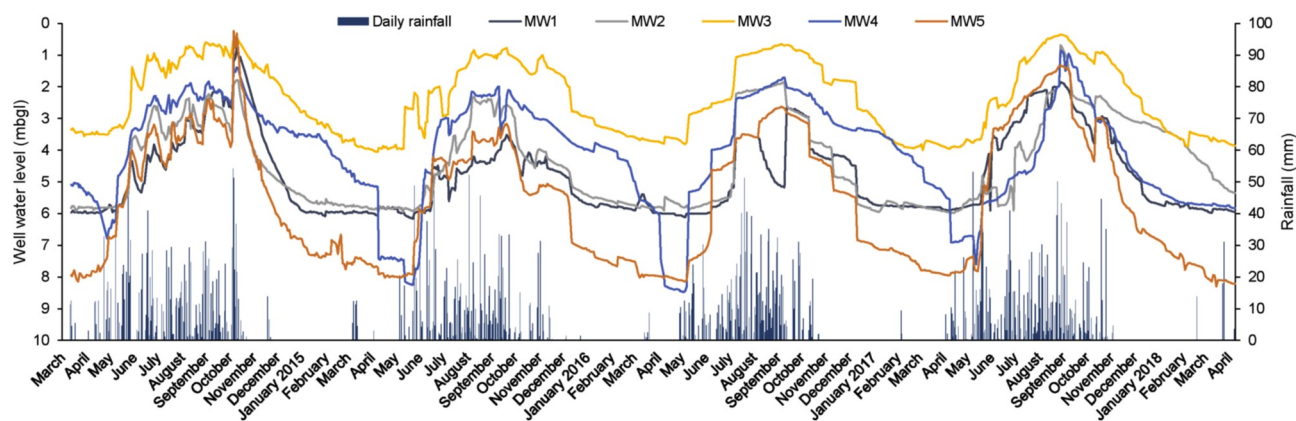
Fig. 3. Daily community observed rainfall and groundwater level data for 2014–18 (well depths are: MW1 6.0 m; MW2 6.9 m; MW3 4.2 m; MW4 9.2 m; MW5 8.4 m).
