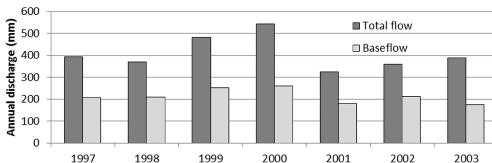
Fig. 4. Annual river discharge and baseflow for the Kilti catchment (1997–2003).
