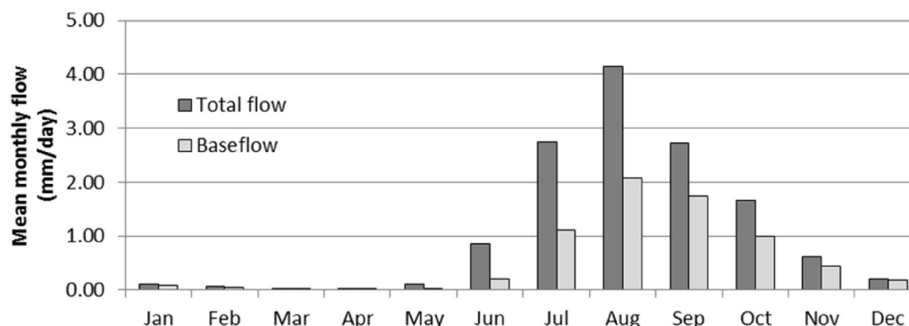
Fig. 5. Mean monthly river discharge and baseflow for the Kilti catchment (1997–2003).
