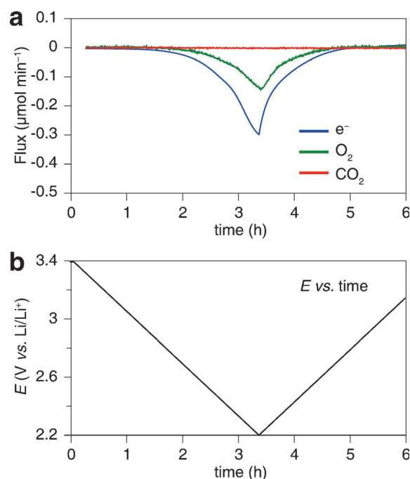
Figure 5. In situ DEMS of a GDL on discharge in phenol–LiTFSI–TEGDME showing 2.04 \text{ e}^- per \text{O}_2 consumed, consistent with \text{Li}_2\text{O}_2 formation. a) Discharge current (blue), \text{O}_2 consumption (green) and \text{CO}_2 evolution (red) in 30 mM phenol/1 M LiTFSI in TEGDME. b) Voltage profile of the DEMS cell. Cyclic voltammetry was applied at a scan rate of 0.1 \text{ mVs}^{-1} .
