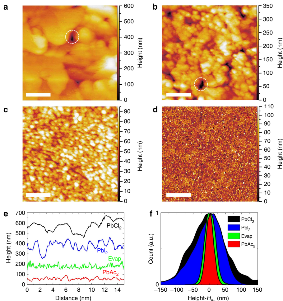
Figure 5 | AFM images of perovskite films. The films were deposited on a FTO/c-TiO 2 substrate derived from the three different lead sources, \text{PbCl}_2 (a), \text{PbI}_2 (b), \text{PbAc}_2 (c) and a vapour-deposited film based on \text{PbCl}_2 (d). The scale bars are 4 \mu\text{m} . Examples of pinholes in \text{PbCl}_2 - and \text{PbI}_2 -derived films are circled, which are notably absent in the film from \text{PbAc}_2 . Line segments from each scan (e) and the height distribution (f) around the average height, H_{Av} , show the exceptional smoothness of the \text{PbAc}_2 -derived films.
