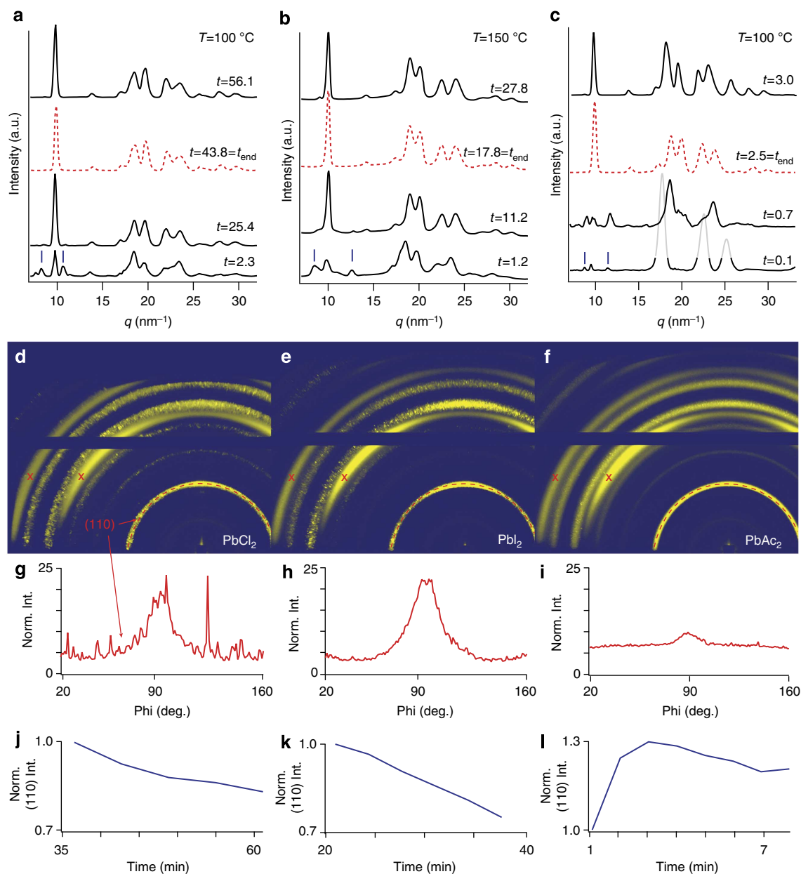
Figure 2 | In situ WAXS data for all three routes. Azimuthally integrated 1D plots at several key time points ( t , in minutes) of annealing for films made from (a) PbCl 2 , (b) PbI 2 and (c) PbAc 2 routes. Red dashed traces indicate the point of complete perovskite transformation, blue stick markers on the bottom-most traces note the peaks used to track the 'precursor' structure; the three grey peaks in c are from the TiO 2 substrate and have been greyed out for clarity. (d-f) 2D WAXS images corresponding to t_{\text{end}} of the respective samples in a-c. Two rings marked with a red 'x' are from the TiO 2 substrate, horizontal line is the detector seam; red dashed line is the (110) peak for the tetragonal perovskite. (g-i) Azimuthal line scans for (110) peak at 10 nm -1 ( q vector) radially integrated between 9.9-10.1 nm -1 and normalized such that the entire integrated area = 1,000. (j-l) Peak intensity of the (110) peak normalized by the intensity at t_{\text{end}} (defined in text). Plots begin ~1 time point before t_{\text{end}} and extend to the end of the experiment.
