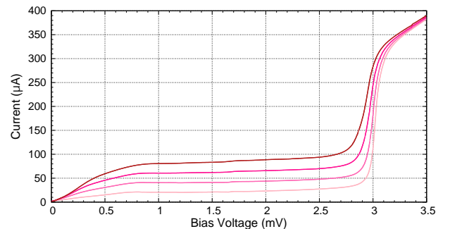
Fig. 1. Reduction of the gap voltage when the mixer, stabilised at a constant block temperature of 4 K, is injected with strong LO power.
