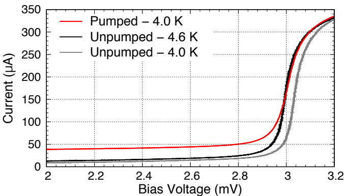
Fig. 2. Plot illustrates how we infer the effective temperature of the tunnel junction by matching the gap voltage of pumped and unpumped IV curves at different block temperature. The temperature shown in the legend indicates the mixer block temperature when the IV curve was taken.
