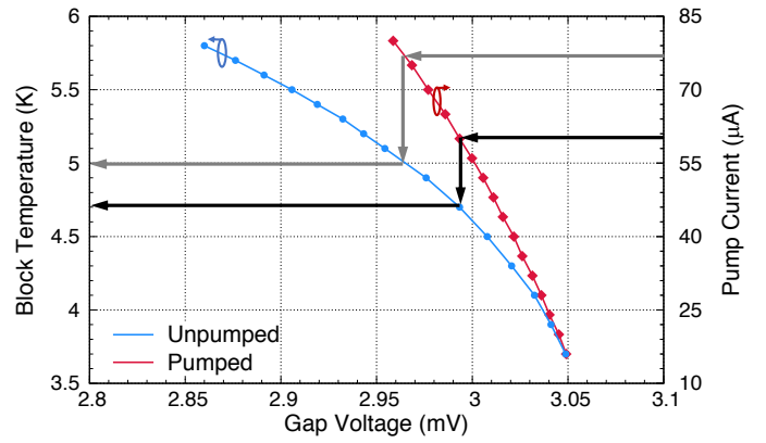
Fig. 3. Relation between the pump current and the effective tunnel junction temperature. The pumped IV curve was measured at a fixed temperature of 3.3 K.
