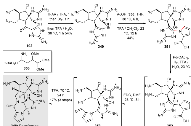
Scheme 43: Enantioselective synthesis of (–)-palau'amine 348 (Baran et al. , 2011) 51
