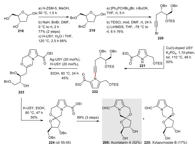
Scheme 30: Zeolite catalyzed synthesis of (+)-acortatarin A 205 (Pale et al. , 2017) 86
