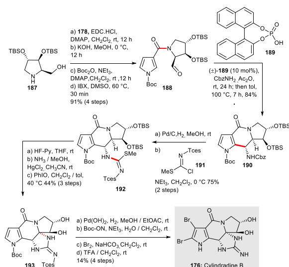
Scheme 25: Synthesis of (+)-cylindradine B 176 (Nagasawa et al. , 2017) 81
