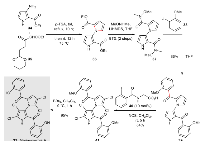
Scheme 5: Synthesis of marinopyrrole A 33 (Gulder et al. , 2016) 35
