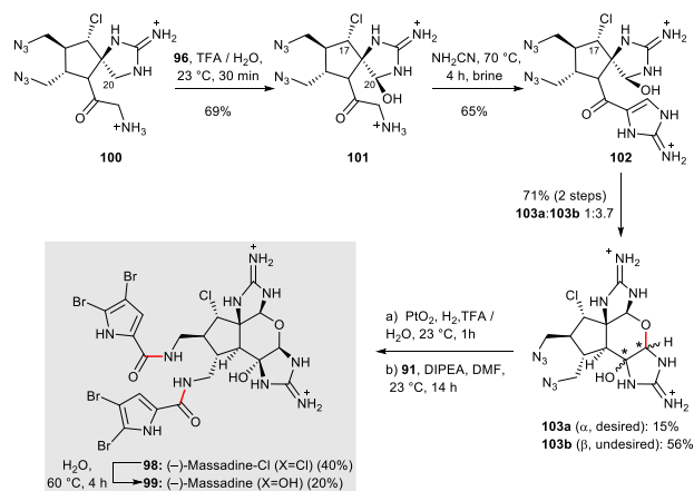
Scheme 13: Enantioselective synthesis of (-)-massadine 99 (Baran et al. , 2011) 51
