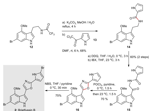
Scheme 2: Synthesis of brietfussin B 2 (Sperry et al. , 2018; Khan and Chen, 2015) 18,19
