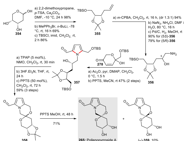
Scheme 44: Synthesis of (+)-pollenopyrroside A 265 (Brimble et al. , 2016) 108
