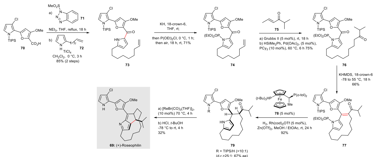
Scheme 9: Asymmetric synthesis of (+)-roseophilin 69 (Harran et al. , 2013) 43
