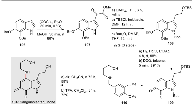
Scheme 14: Synthesis of sanguinolentaquinone 104 (Spiteller et al. , 2018) 54
