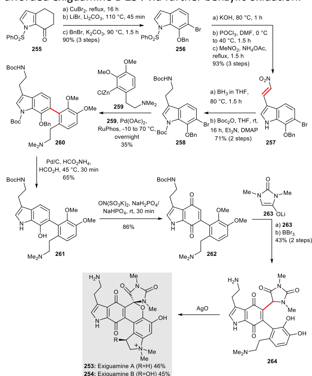
Scheme 33: Syntheses of exiguamines A 253 and B 254 (Trauner et al. , 2012) 92
