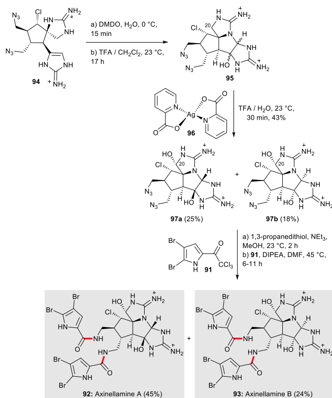
Scheme 12: Enantioselective synthesis of (-)-axinellamine A 92 and (-)-axinellamine B 93 (Baran et al. , 2011) 51
