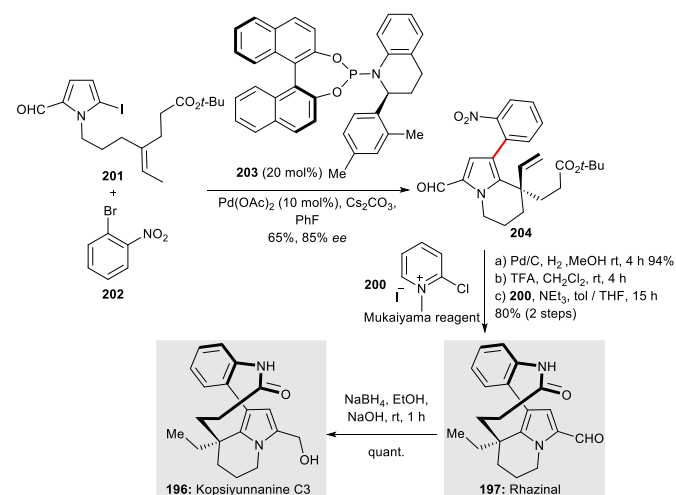
Scheme 26: Synthesis of (+)-rhazinal 197 and (+)-kopsiyunnanine C3 196 (Gu et al. , 2016) 83
