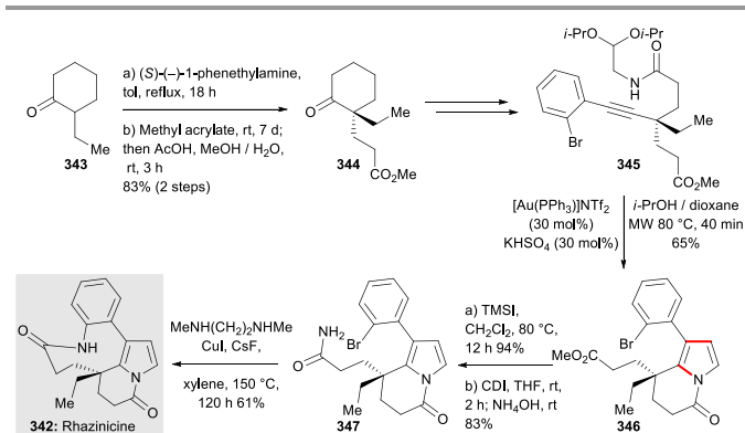
Scheme 42: Synthesis of (–)-rhazinicine 342 (Tokuyama et al. , 2013) 106
