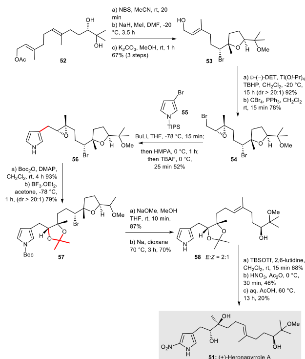
Scheme 7: Synthesis of (+)-heronapyrrole A 51 (Morimoto et al. , 2015) 38
