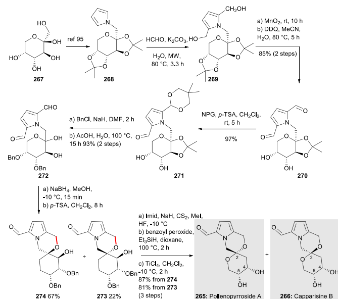
Scheme 34: Syntheses of (+)-pollenopyrroside A 265 and (+)-capparisine B 266 (Zhao et al. , 2015) 94
