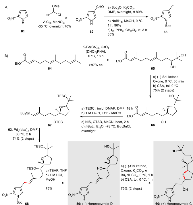
Scheme 8: Synthesis of (+)-heronapyrrole C 60 and (–)-heronapyrrole D 59 (Brimble et al. , 2016) 39
