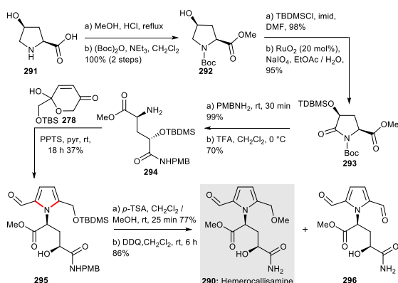
Scheme 37: Synthesis of (–)-hemerocallisamine 290 (Brimble et al. , 2017) 98
