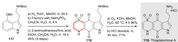
Scheme 16: Synthesis of thiaplakortone A 116 (Quinn et al. , 2013) 56
