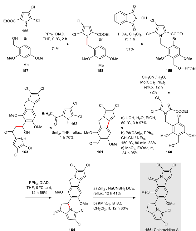
Scheme 22: Synthesis of chlorozidine A 155 (Mhaske et al. , 2017) 67
