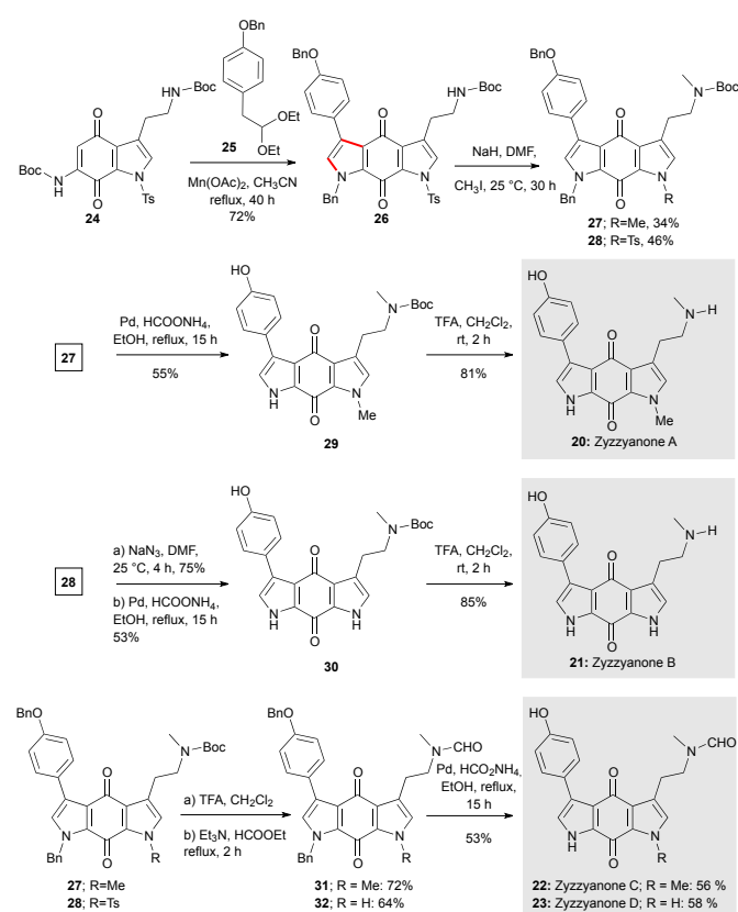
Scheme 4: Synthesis of zyzzyanone (A-D) 20-23 (Velu et al., 2013) 29
