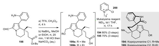
Scheme 27: Synthesis of (+)-kopsiyunnanine C1 194 and (+)-kopsiyunnanine C2 195 (Gu et al. , 2016) 83
