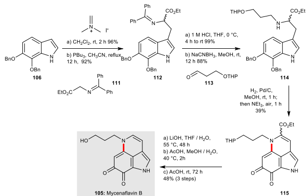
Scheme 15: Synthesis of mycenaflavin B 105 (Spiteller et al. , 2018) 54
