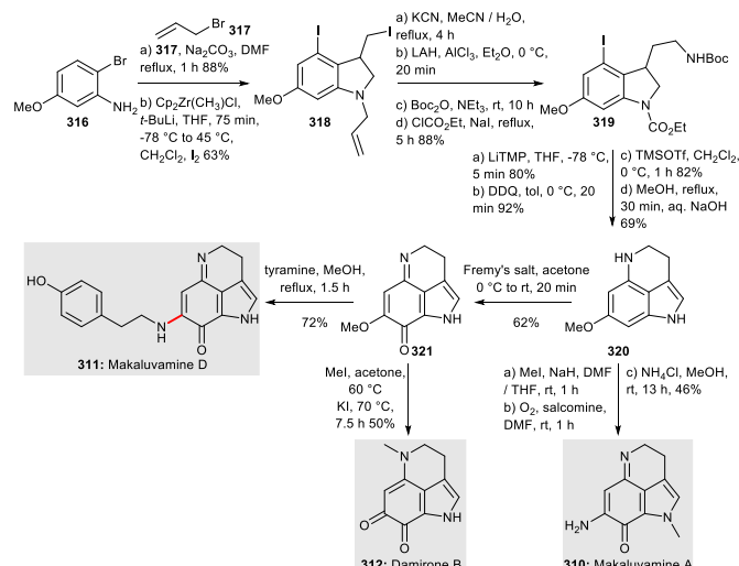
Scheme 39: Syntheses of makaluvamine A 310 , makaluvamine D 311 and damirone B 312 (Tokuyama et al. , 2012) 102
