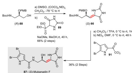
Scheme 11: Enantioselective synthesis of (S)-mukanadin F 87 (Barker et al. , 2018) 47
