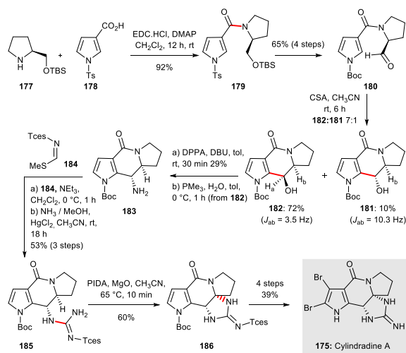
Scheme 24: Enantioselective synthesis of (+)-cylindradine A 175 (Nagasawa et al. , 2014) 78
