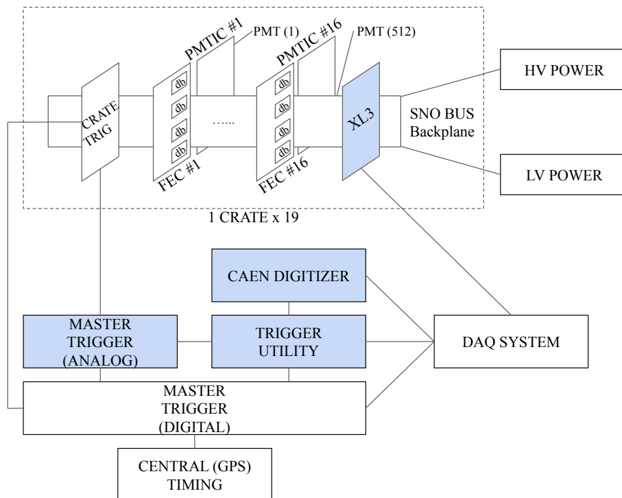
Figure 7. A schematic of the SNO+ electronics. Adapted from [73], with the updates with respect to SNO highlighted.
