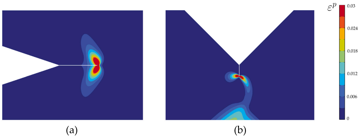
Fig. 7. Contours of the effective plastic strain \epsilon^p for (a) DCB and (b) notched cantilever beam specimens with a hardening exponent of N = 0.1 , at J = 0.15 \text{ kJ/m}^2 , \sigma_Y = 900 \text{ MPa} , and (a, W - a) = 0.01 \text{ mm} .
