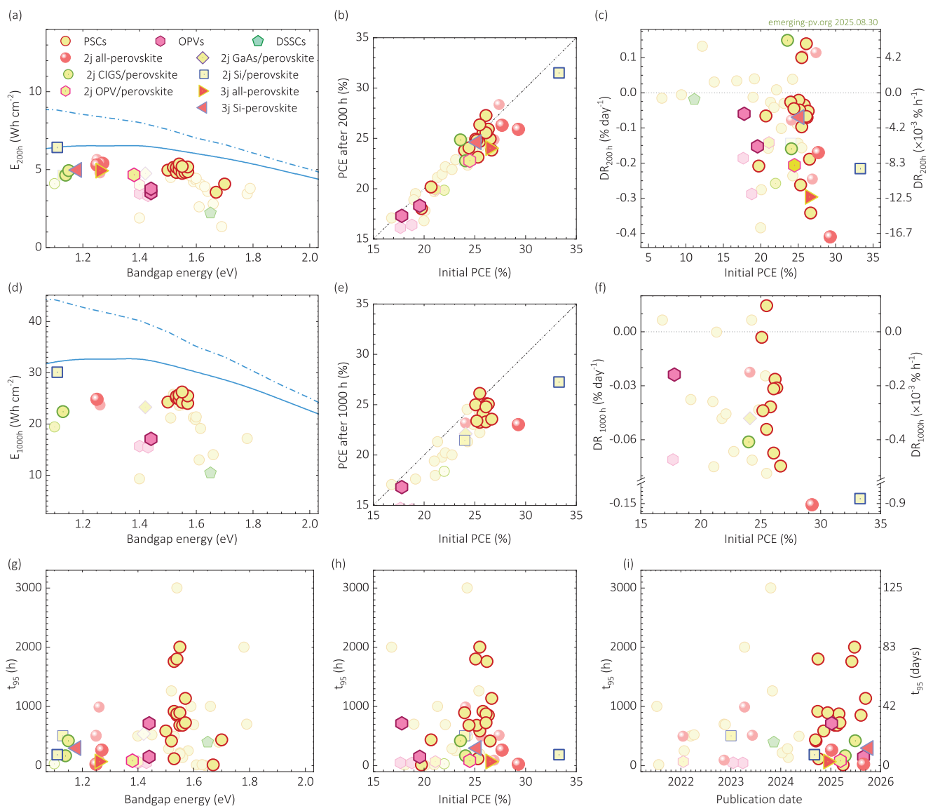
FIGURE 7 | Operational stability under 100 \text{ mW cm}^{-2} illumination at MPP conditions during 200 h (a-c) and 1000 h (d-f) of testing. Analysis parameters include: (a,d) stability test energy yield (STEY, Equation 9, Table 2) as a function of bandgap energy, (b, e) final as a function of initial power conversion efficiency, and (c, f) degradation rate (Equation 10 in Table 2) as a function of initial efficiency. The characteristic t_{95} times are also plotted as a function of bandgap energy (g), initial efficiency (h), and publication date (i). Experimental data are summarized in Section 7.4. The solid and dot-dashed blue lines in the STEY plots (a, d) represent the detailed balance theoretical limits for single-junction and double-junction devices, respectively. In (b, e), the diagonal dot-dot-dashed lines indicate where the final and initial efficiencies are equal. In (c, f), positive values above the horizontal dotted line denote devices where the PCE increased relative to the initial value.
