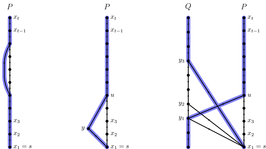
Fig. 2 Contradiction to minimality in the proof of Claim 4.2
