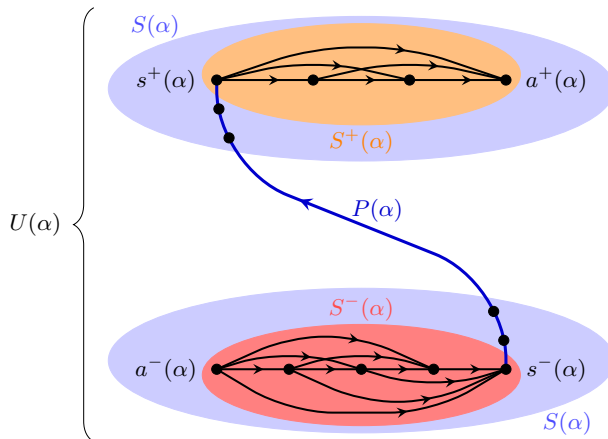
Fig. 1 The sets U(\alpha) , S^+(\alpha) , S^-(\alpha) , vertices s^+(\alpha) , s^-(\alpha) and path P(\alpha)
