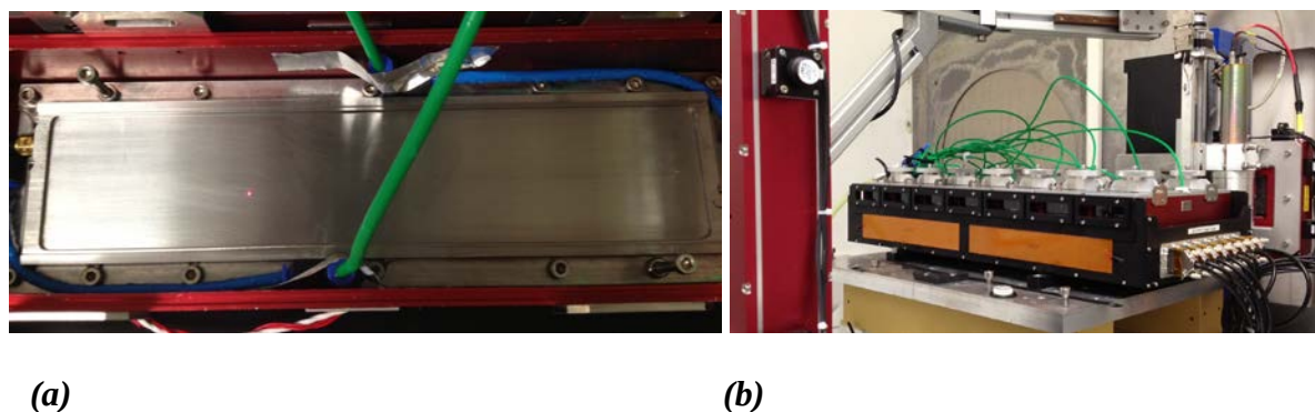
Figure 1: Images showing the experimental set up for the NR measurements at 25°C and 10°C, (a) view of stainless steel troughs, (b) arrangement of 7 steel trough on sample changer.
