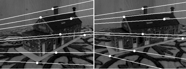
Figure 7: Corresponding epipolar lines and points using the computed fundamental matrix.
