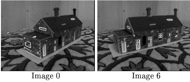
Figure 3: Automatic extraction of parallelogram line cycles. The 3 and 4 cycles are shown before parallelogram completion. There are 15 groupings in image 0, and 26 in image 6.
