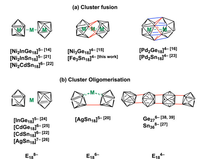
Fig. 1 Cluster fusion vs. cluster oligomerisation of E 9 polyhedra, E = Ge, Sn. 14–16,19–29
