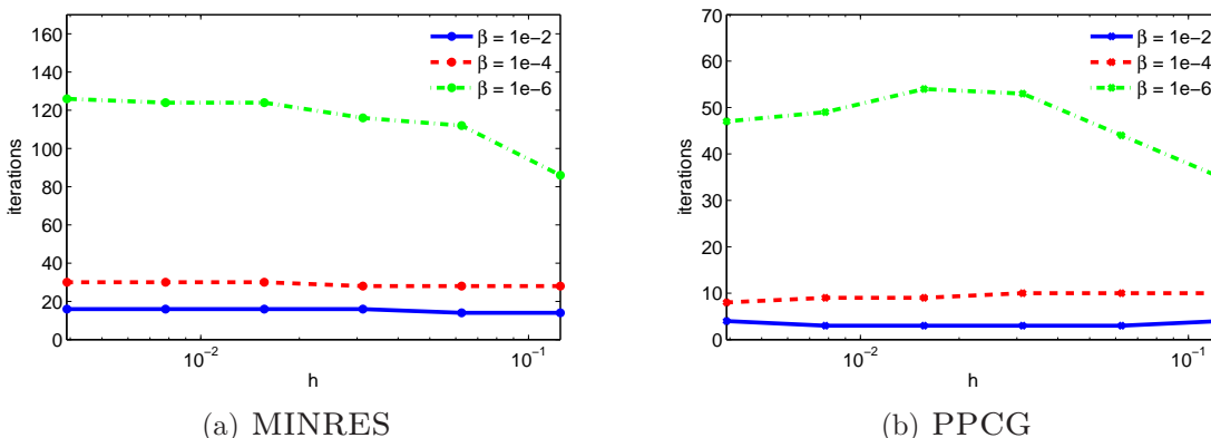
Figure 2: Number of iterations for MINRES with \mathcal{P}_{D_3} and PPCG with \mathcal{P}_{C_2} to converge for \beta = 10^{-2} , 10^{-4} and 10^{-6}
