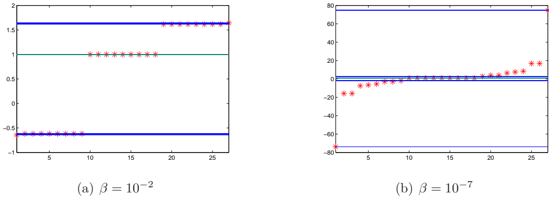
Figure 1: Eigenvalues of \mathcal{P}_{D1}^{-1}\mathcal{A} and eigenvalue bounds predicted by Proposition 2 (lines are the predicted, *s are the eigenvalues)
