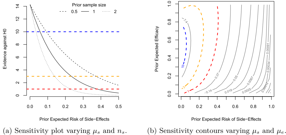
Figure 3: Sensitivity analysis of \text{BF}_{10} for the aspirin trial.
