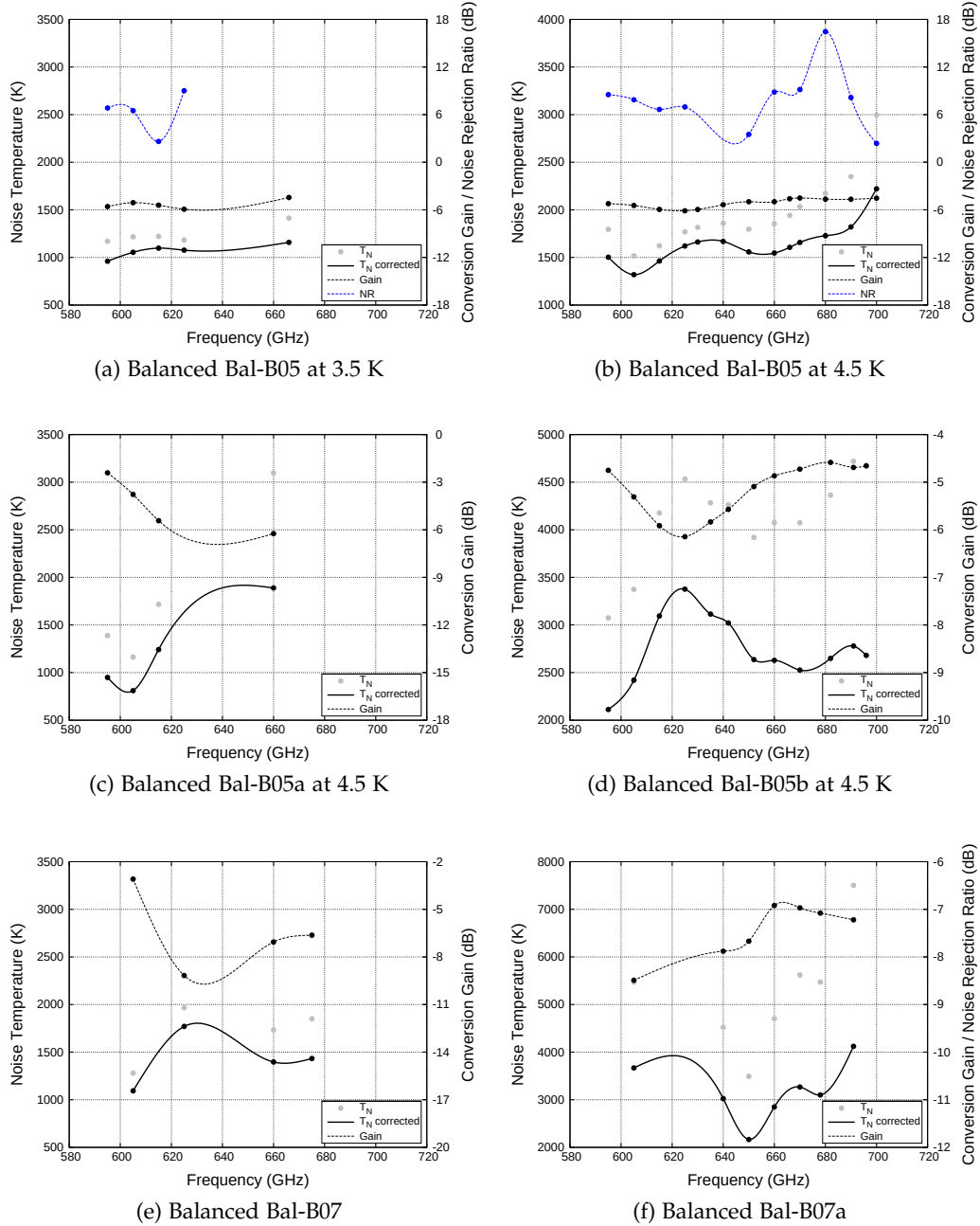
Figure B.1: Measured noise temperature and DSB conversion gain of Balanced Bal-B05 and Bal-B07 across the operating RF bandwidth. The grey points corresponding to the uncorrected values.
