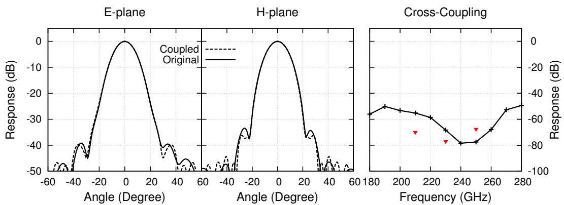
Figure 2.17: The HFSS predicted far-field patterns of the radiating horn in the two-horn array, compared with the same patterns of a single horn. The panel on the right shows the comparison of HFSS predicted cross-coupling with the measured data. The red triangle indicates the measured response, while the black thick line represents the result predicted by HFSS.
