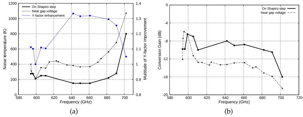
Figure 8.5: (a) Y-factor and noise temperature improvement when biasing at the S_1 compared to the conventional bias point near the V_{gap} . (b) Same as left panel, but plotting for the conversion gain improvement.
