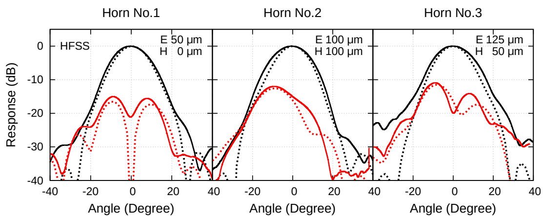
Figure 2.16: Measurements of co- and cross-polarization for all three first generation prototype horns, comparing with HFSS simulation. The lateral misalignment used in the HFSS model are labelled on the top right of the panels, with E and H indicating the plane where the misalignment shifted, and the number indicating the amount of shifting. The solid curves are the measured data while the dotted curves are the computed patterns. The black curves represent the co-polarization patterns, while the red curves correspond to the cross-polarization patterns.
