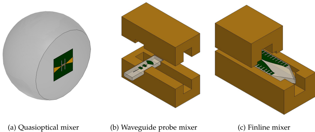
Figure 1.4: Examples of various types of mixers, utilising different coupling mechanisms to the mixer. They were drawn only for illustration, hence are not drawn to scale.
