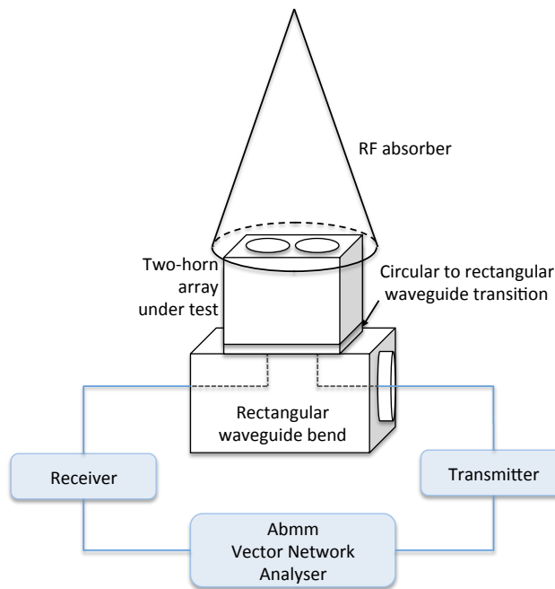
(a) Cross-coupling measurement setup
