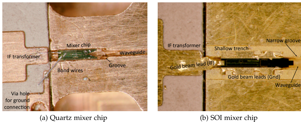
Figure 5.5: A photo showing the mixer chip sitting in the groove inside the waveguide. Two bond wires were used to connect the mixer chip bonding pads to the IF transformer board.
