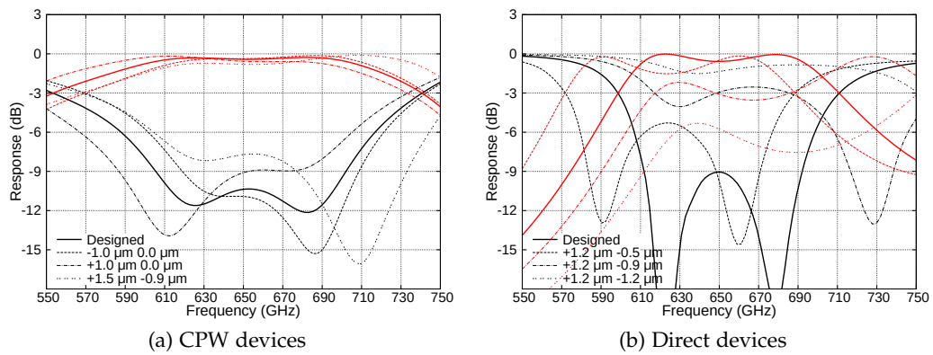
Figure 5.14: HFSS simulating the effects of junction misalignment to the power coupling. The value in the legend corresponding to the magnitude of offset along (horizontal) and orthogonal (vertical) to the finline axis. The couplings to the junction are plotted with red lines, while the black lines representing the return loss.
