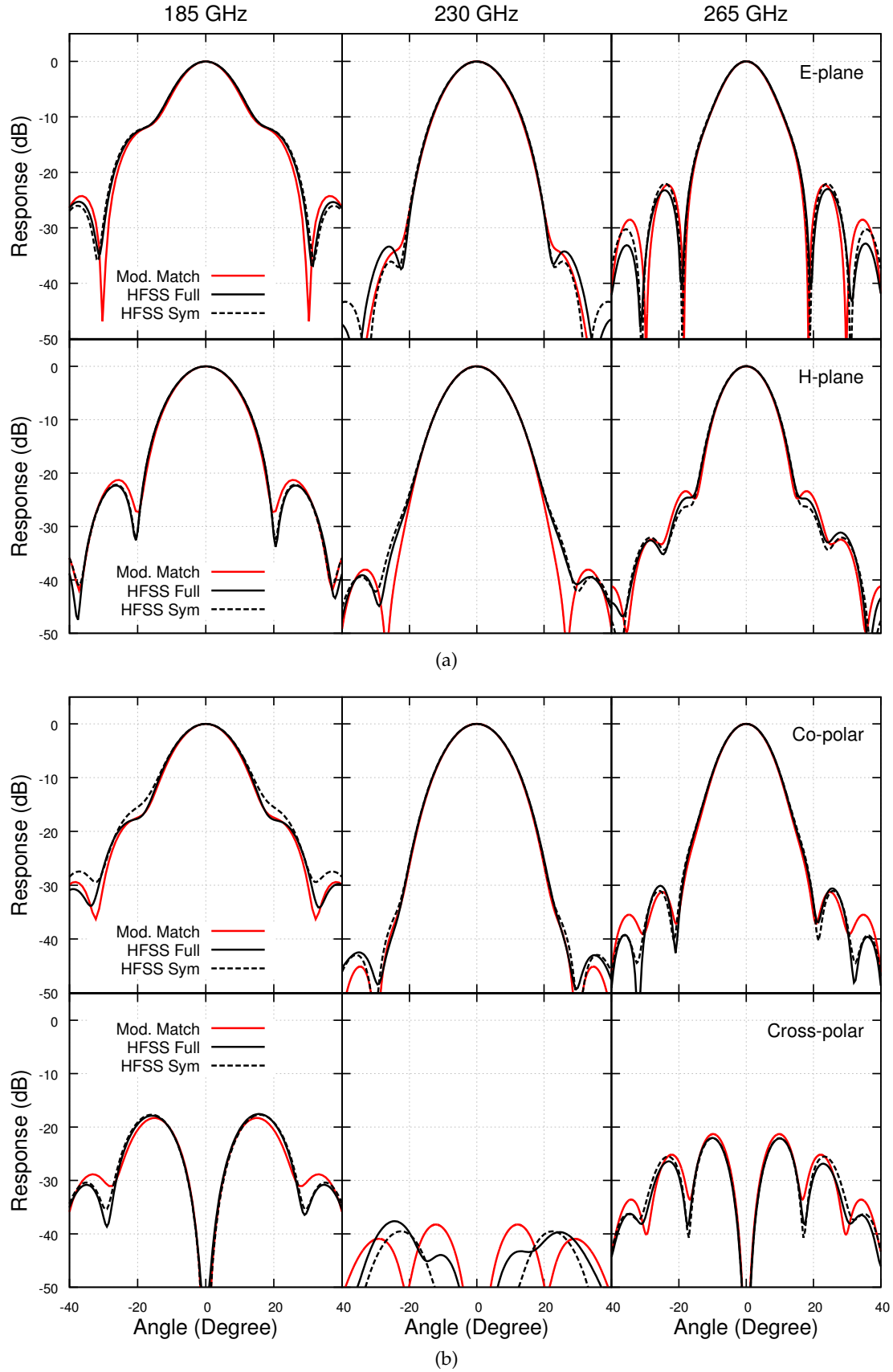
Figure 2.14: Far-field patterns of a 3-section smooth-walled horn across the 230 GHz design wavebands, generated by HornSynth , a full-horn HFSS model and a simplified quarter-wedged horn HFSS model.
