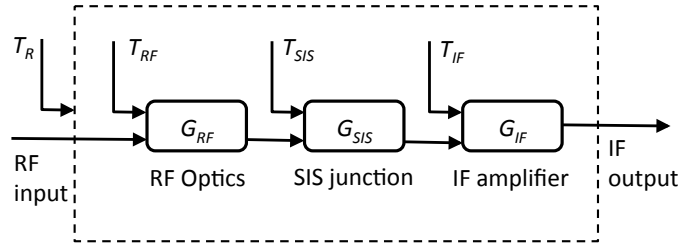
Figure 3.6: Diagram showing the various components making up to the final SIS receiver that contribute to the overall noise temperature.
