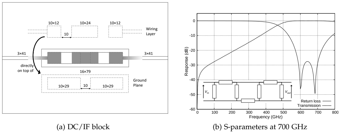
Figure 6.4: (a) Layout of the broadside coupler as DC/IF block. Panel (b) shows the equivalent circuit, and the transmission and the return loss simulated using HFSS.
