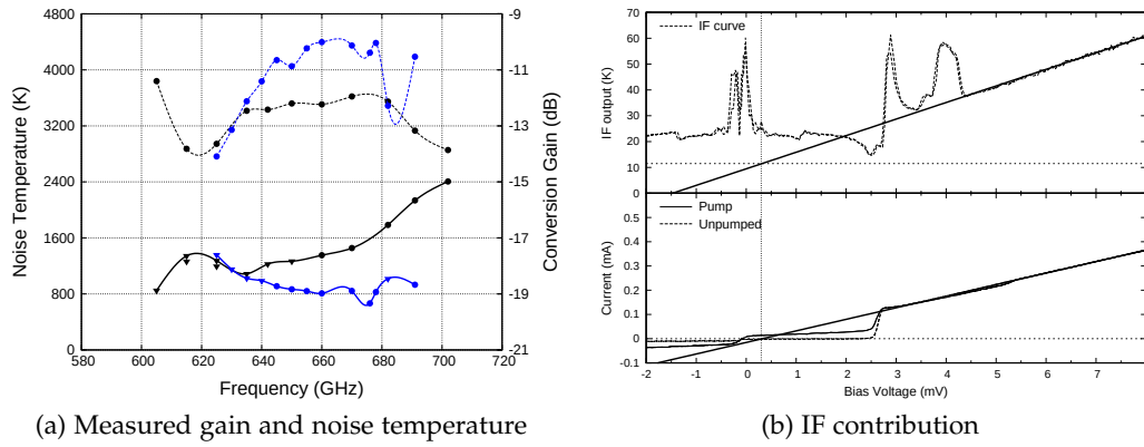
Figure 6.23: (a) DSB gain (dashed line) and noise temperature (solid line) of Bal-B04a (black curves) and Bal-B04b (blue curves) measured independently. (b) IF noise contribution estimated experimentally showing high IF noise at \sim 12.5 K.
