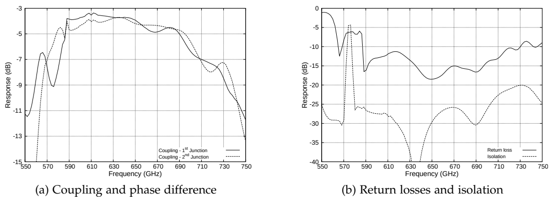
Figure 7.6: Ansoft Designer simulation of the full sideband separating mixer chip by importing various S-parameters from HFSS.
