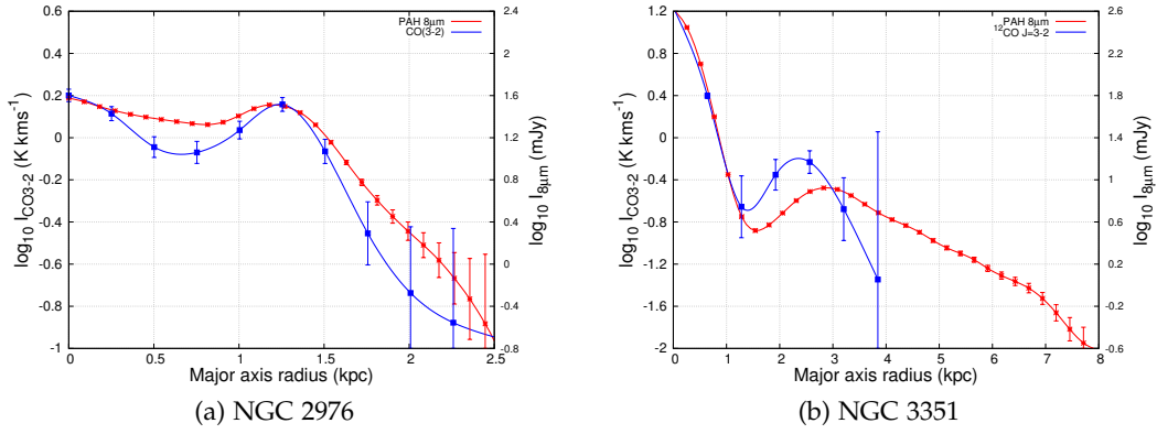
Figure 10.8: Comparison of ^{12}\text{CO } J=3 \rightarrow 2 radial profile with that of Spitzer IRAC 8\mu\text{m} for both NGC 2976 and NGC 3351. ^{12}\text{CO } J=3 \rightarrow 2 intensity is in \text{K km s}^{-1} (blue, left axis) and PAH 8\mu\text{m} is in mJy (red, right axis). All data were convolved with kernels that match the PSF of ^{12}\text{CO } J=3 \rightarrow 2 data.
