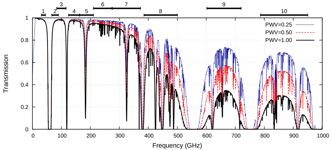
Figure 1.2: Atmospheric transmission window at Llano de Chajnantor, Chile, at the altitude of 5040 m. Downloaded from http://almascience.eso.org .
