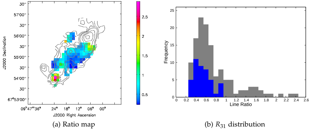
Figure 10.4: Panel (a) shows the R_{31} ratio map for NGC 2976 constructed using the ^{12}\text{CO } J=1 \rightarrow 0 map from BIMA SONG. The grey contour line is the ^{12}\text{CO } J=3 \rightarrow 2 contour map to show the position of the ratio map relative to the galaxy. Panel (b) shows the distribution of the value of R_{31} across the galaxy. The grey histogram shows the pixel count when including all the pixels within the ratio map, whereas in the blue histogram we discard pixels within the ratio map with SNR less than 2.
