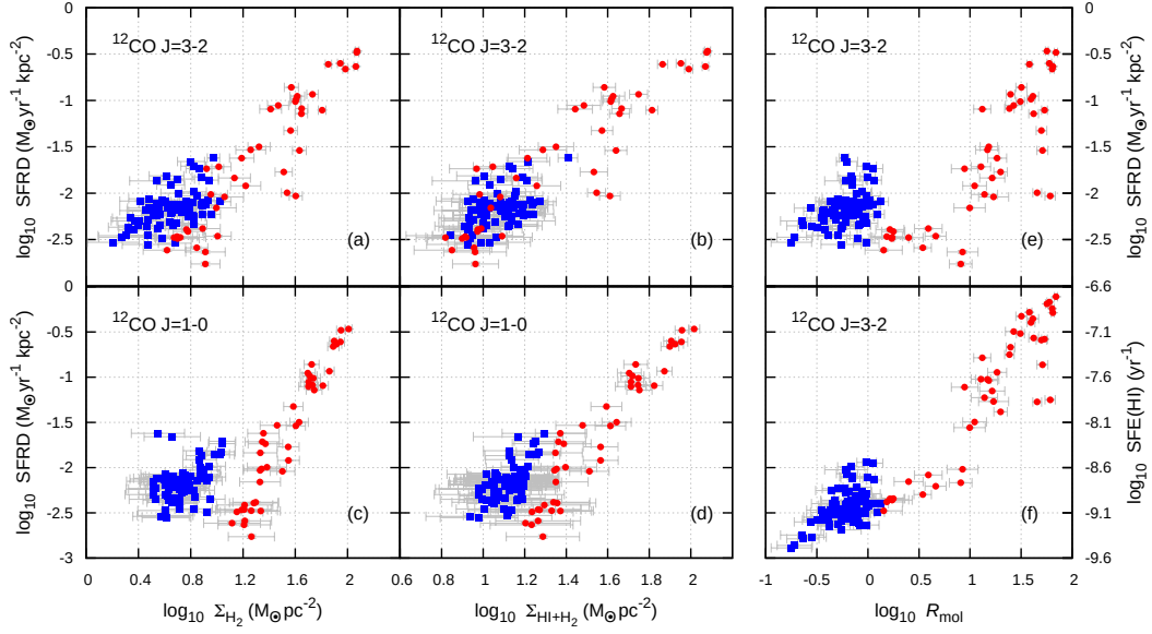
Figure 10.7: \Sigma_{SFR} as a function of different gas phase: (left) H_2 only, (centre) H\text{I}+H_2 and (right) H_2 -to- H\text{I} ratio. Each point in these diagrams represents a single pixel corresponding to the pixel size of our ^{12}\text{CO } J=3 \rightarrow 2 map. Pixels from NGC 2976 are plotted with blue square, while regions from NGC 3351 in red circle.
