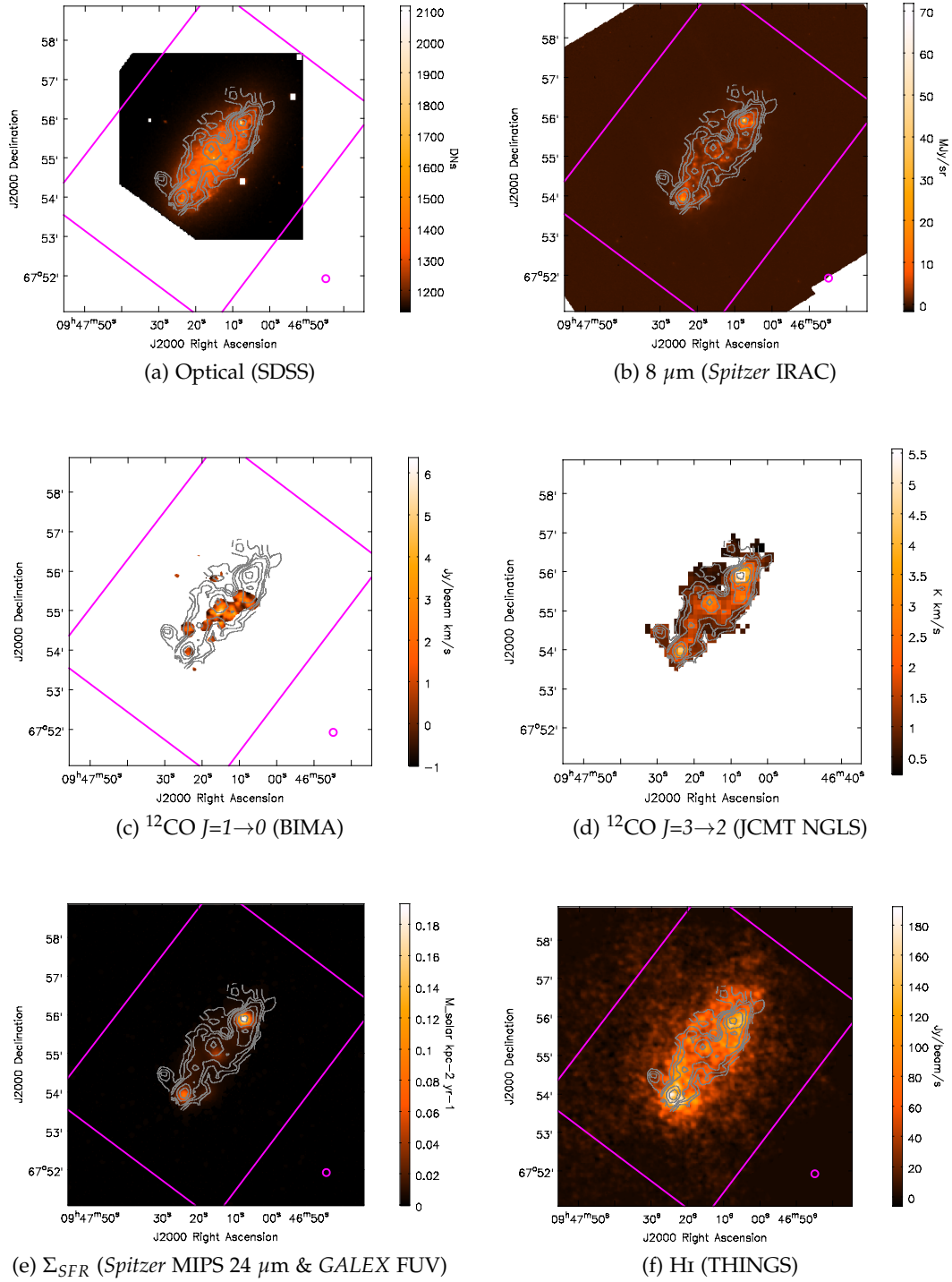
Figure 10.1: Contours of the ^{12}\text{CO } J=3\rightarrow2 data of NGC 2976 overlaid on the corresponding ancillary images from the archives. The contour levels are 0.36 ( 3\sigma ), 0.72, 1.08, 2.0, 3.0 and 5.0 \text{K km s}^{-1} (temperature in T_{\text{mb}} ). In all panels, a magenta box is drawn to show the region mapped by HARP-B, and a magenta circle to indicate the 14.5'' angular resolution of the ^{12}\text{CO } J=3\rightarrow2 data. All images are oriented North up and East to the left, with the inclination angle of 54^\circ . The image representing \Sigma_{\text{SFR}} had been convolved to the HARP-B beam size.
