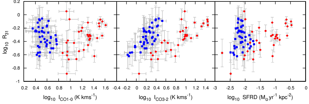
Figure 10.6: Correlation of R_{31} with ^{12}\text{CO } J=1\rightarrow0 , ^{12}\text{CO } J=3\rightarrow2 and SFR surface density respectively. The blue square represent pixel points from NGC 2976, whereas the red dots represent pixel points from NGC 3351.
