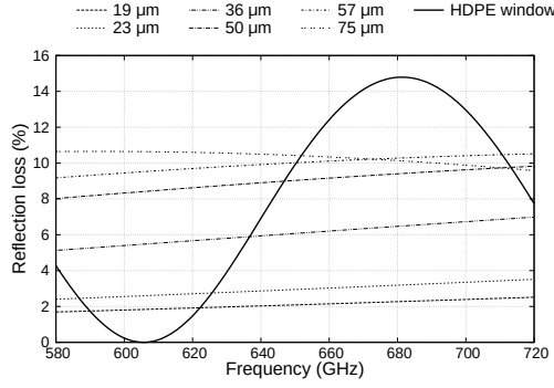
Figure 3.8: Reflection loss of beam splitter with various thickness and a 660 \mu\text{m} thick HDPE Dewar window without corrugation.
