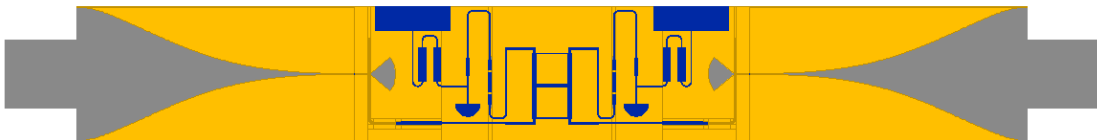
Figure D.5: The layout of the balanced SIS mixer chip.
