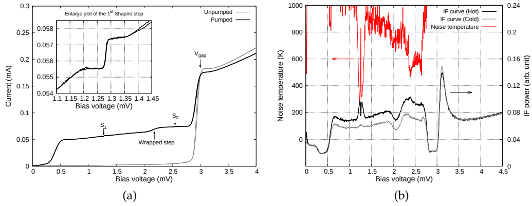
Figure 8.4: (a) IV curve showing the step wrapping, the Shapiro steps and the photon steps at 634 GHz. (b) Calculated noise temperature using the hot and cold load IF curves.
