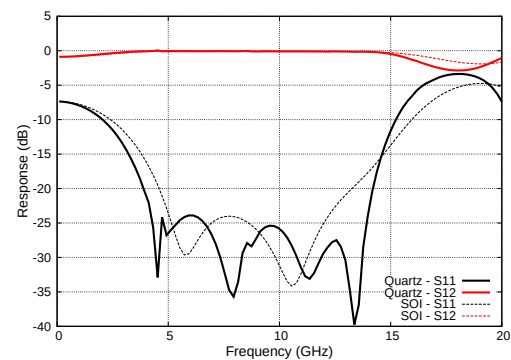
(b) Insertion and return loss
