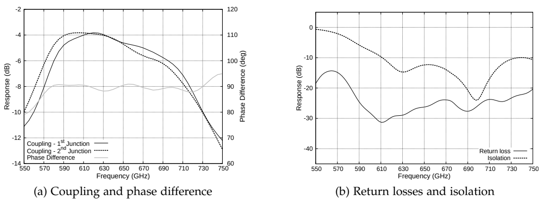
Figure 6.6: HFSS simulation of a subsection of the mixer chip including the RF quadrature hybrid, the DC/IF blocks and the tuner circuits.
