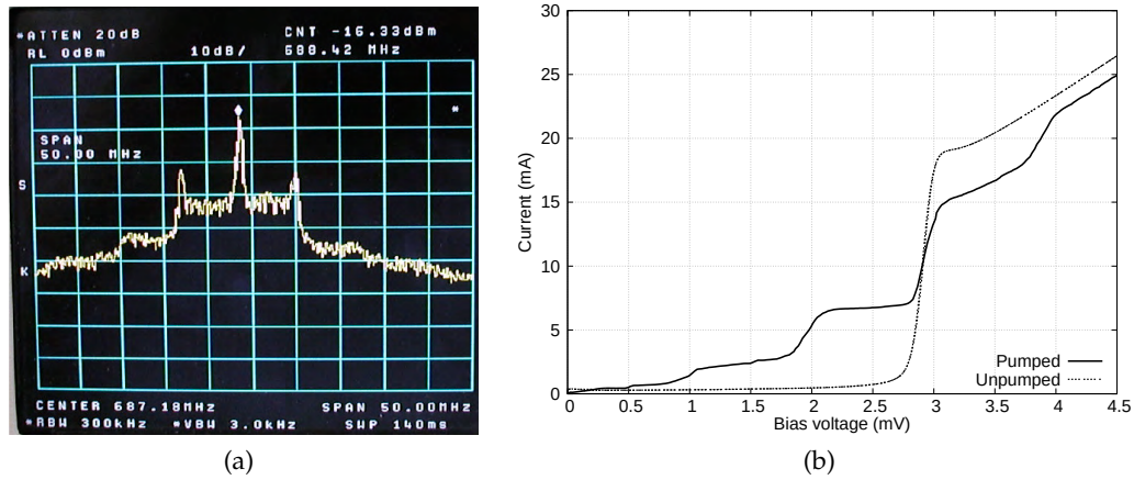
Figure 9.3: (a) Beat note from a narrow line fibre laser and a narrow line diode laser. The factory specification of line width is about 10 kHz, however the spectrum of the down-converted signal shows additional noise from the laser power supply. (b) The pumped and unpumped IV curve of a 230 GHz SIS mixer illuminated with a photonic LO source.
