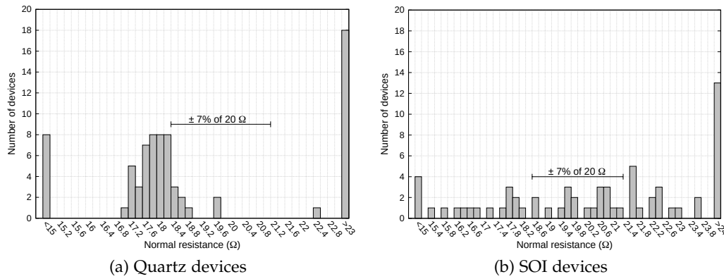
Figure 5.3: Normal resistance of all the quartz and SOI mixer that have a live junction.
