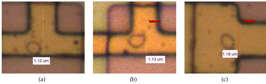
Figure 5.13: Microscope photos showing the junction was not aligned to the microstrip as designed.
