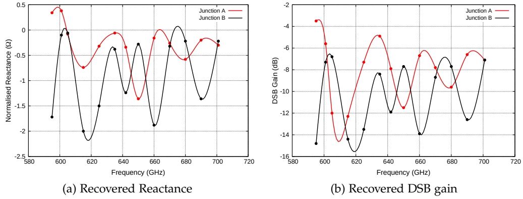
Figure 6.22: Embedding impedance and DSB gain recovered from SuperMix model.
