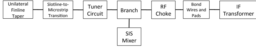
(a) Block diagram of SuperMix model
