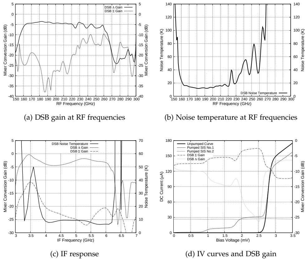
Figure D.4: SuperMix simulations showing the predicted behaviour of the complete balanced SIS mixer chip design. The simulation was carried out with the following settings: bias voltage at 2.4 mV, IF frequency at 5 GHz, and RF frequency at 220 GHz.
