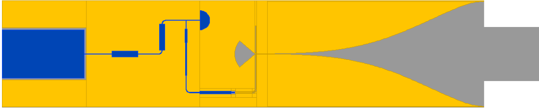
Figure D.3: The layout of the single-port SIS mixer chip.
