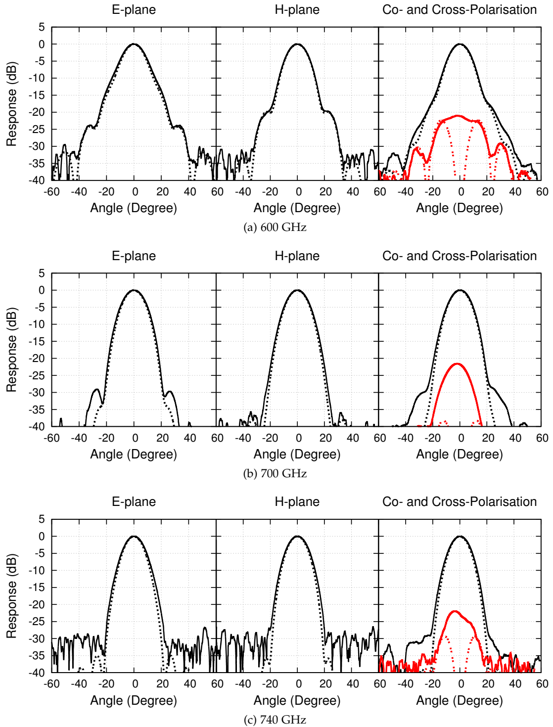
Figure 2.12: Beam pattern measurements of horn No. 3 from the second generation smooth-walled horn in the 700 GHz frequency band. The solid lines are the measured beam patterns, while the dash lines are the calculated patterns using modal matching. In the right column, the red colour lines represent the cross-polar patterns, and the black lines are the co-polar patterns.
