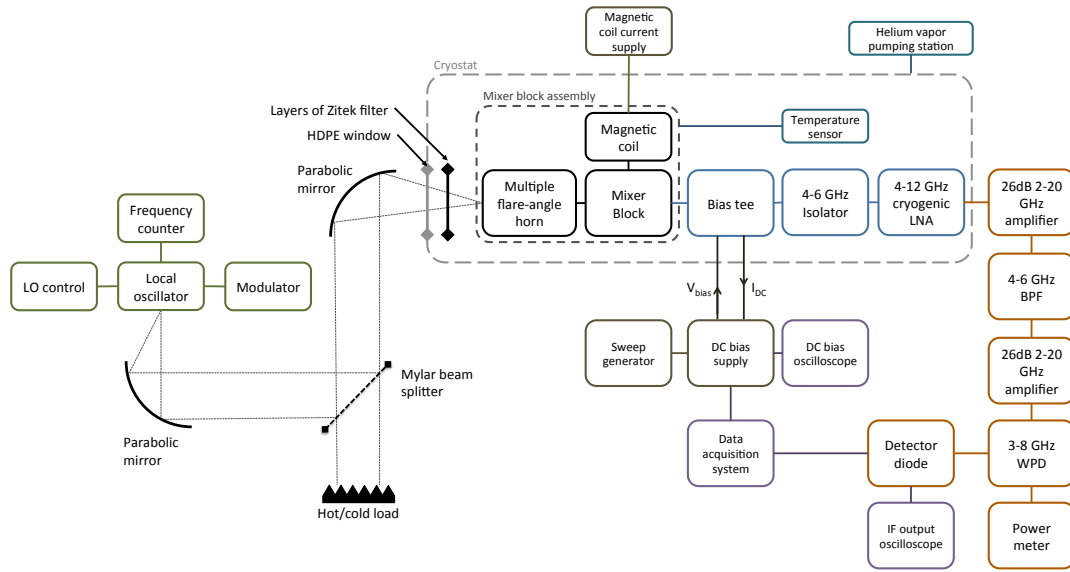
(a) Block diagram of the test system
