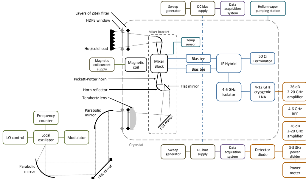
Figure 6.14: Block diagram of the balanced mixer test setup.
