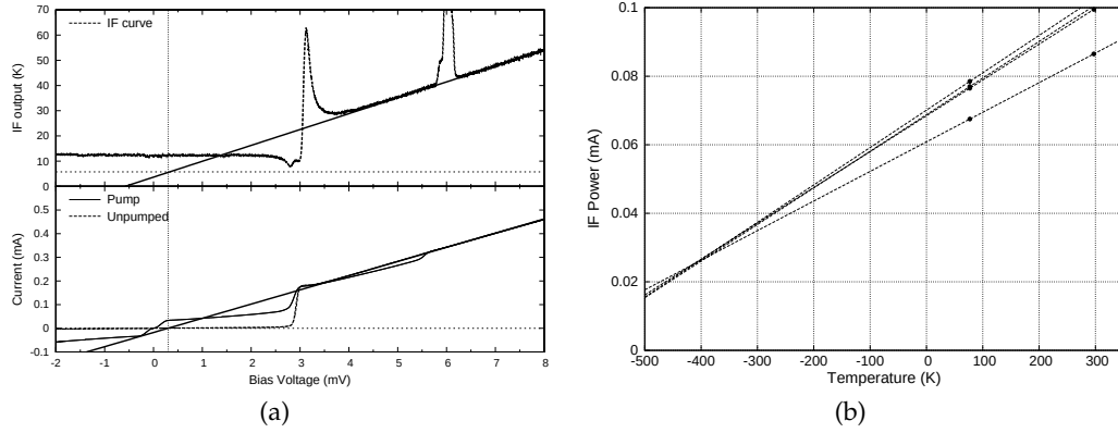
Figure 5.15: RF and IF noise contribution estimated from the unpumped IV and IF curve of FSOI A-D2N1.
