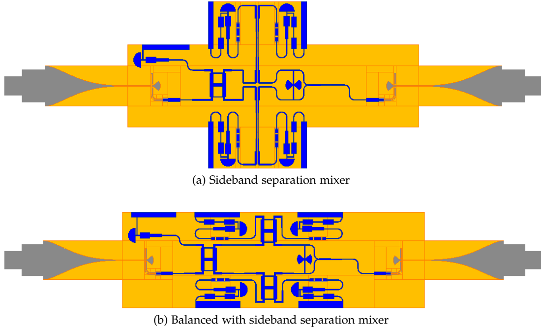
Figure 7.3: AutoCAD layout of the complete sideband separating and balanced-2SB SIS mixer chip. These drawings were drafted without the dielectric layers for clarity.
