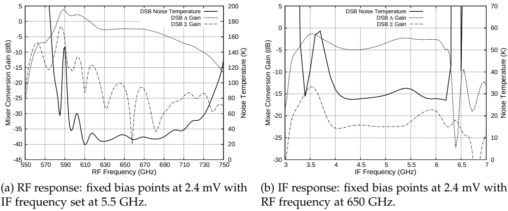
Figure 6.9: SuperMix simulations showing the predicted behaviour of the final design of the balanced mixer chip.
