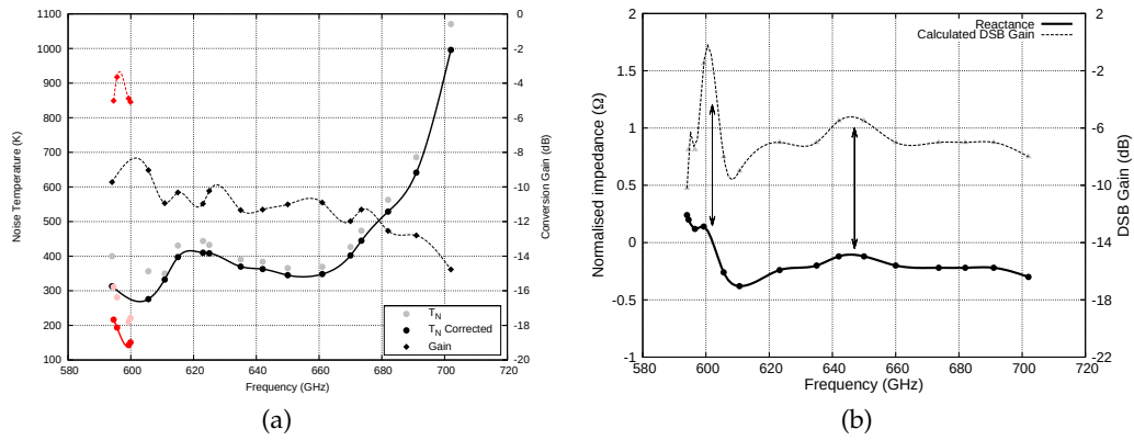
Figure 5.8: (a) Frequency response of the tested F74 C-D7N6 quartz mixer. The two tuning dips are clearly observed around 600 GHz and 650 GHz. The red curves indicate measurement done at bias voltage close to the actual first photon step. (b) Embedding impedance and DSB gain recovered using SuperMix across the operating RF bandwidth.
