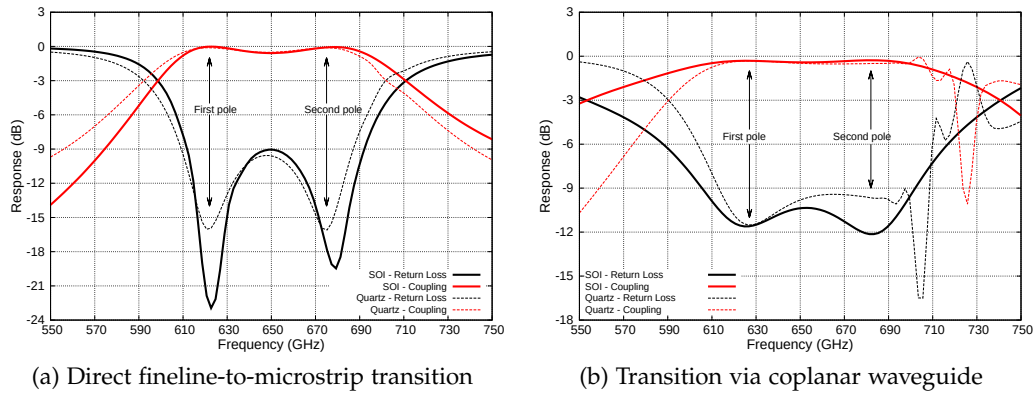
Figure 4.8: HFSS simulation showing that the tuner design exhibiting broad bandwidth of 100 GHz centred at 650 GHz.
