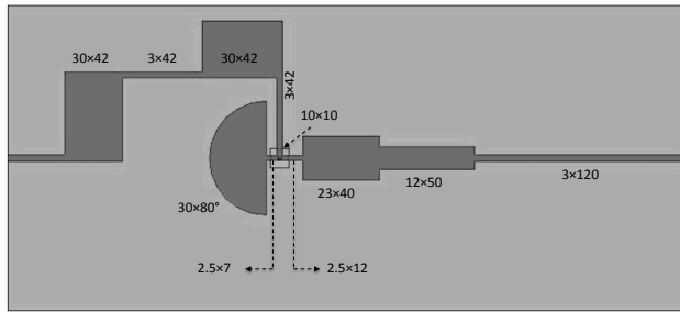
Figure 4.6: (a) Electrical diagram representing the RF tuning circuit of the finline mixer. (b) Layout of the RF tuning circuit with an RF choke to prevent RF leakage to the IF port. The dimensions for various structures are similar to the previous figures. (c) Return losses and coupling efficiency of the tuning circuit across the designed RF band.
