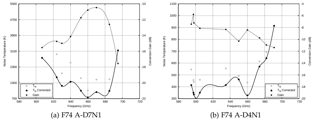
Figure A.2: Measured noise temperature and DSB conversion gain of F74 A-D7N1 and F74 A-D4N1 across the operating RF bandwidth. The grey points corresponding to the uncorrected noise measurement.
