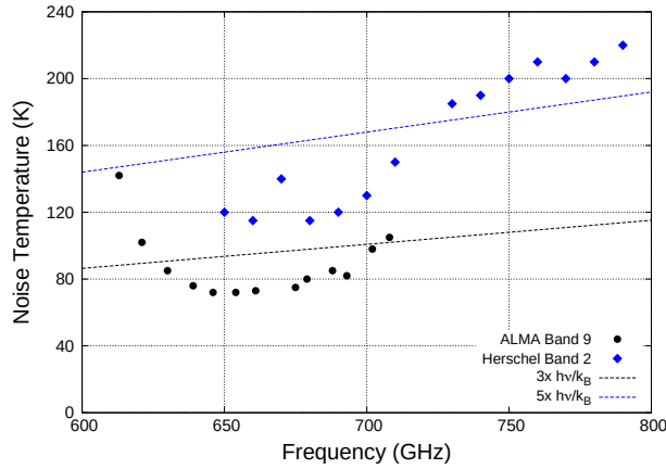
(a) ALMA &amp; Herschel noise temperature performance
