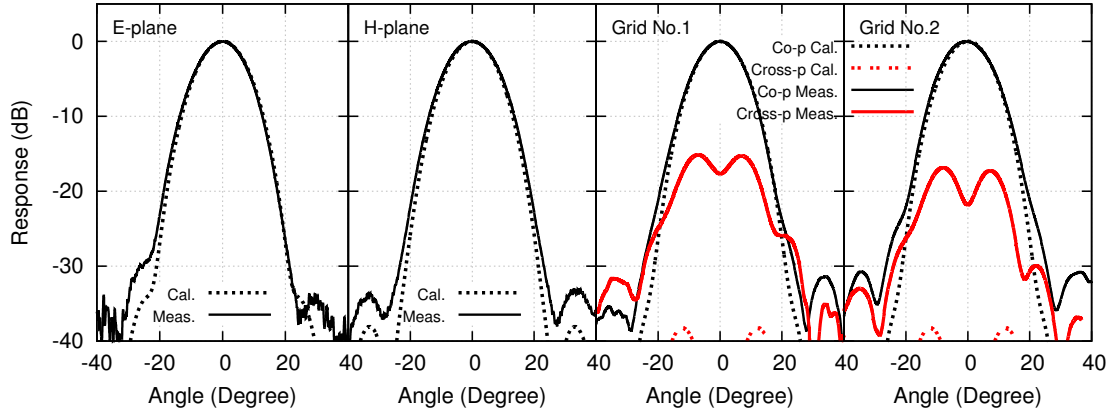
Figure 2.7: Beam pattern measurements of the first generation smooth-walled horn No. 1 at the central frequency 700 GHz. The measured beam patterns match very well with theory, given the tight tolerances required at this wavelength. Grid No. 1 and grid No. 2 represent two different polarizers used during the measurements for comparison purpose. The beam patterns measured at various other frequencies across the wavebands are presented in Appendix C.
