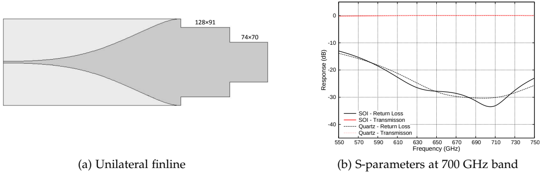
Figure 4.2: (a) Layout of the unilateral finline taper with a 2-step notch to match the impedance of the unloaded waveguide to the 15 \mu\text{m} SOI substrate. The quoted dimensions of the matching notches are in width \times length, in \mu\text{m} . (b) Return loss and coupling efficiency across the designated RF bands for both the quartz and the SOI substrates.
