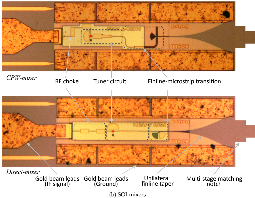
Figure 4.1: Overview of the unilateral finline mixer designs, with two different types of finline-to-microstrip transition and two different types of substrate, showing the different components of the complete mixer chip. The red dot near the half-moon stub indicates the location of the SIS tunnel junction.
