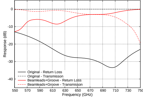
Figure 6.18: Changes in the power coupling behaviour of the finline taper and the matching notches due to the existence of the waveguide groove.
