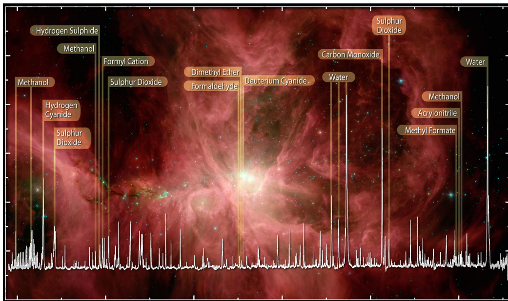
Figure 1.1: Example of image taken in sub-mm region, and the wealth of spectral lines available in this region (480 GHz–2 THz). This European Space Agency (ESA) public released image was downloaded from http://herschel.cf.ac.uk (hosted by Cardiff University), in courtesy of UK Herschel team.
