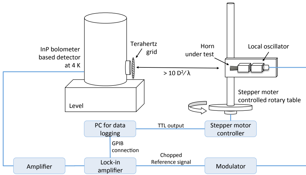
Figure 2.6: Schematic diagram showing the setup of the far-field beam pattern test range.
