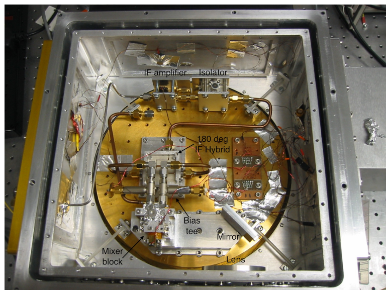
(b) Working area of the Dewar
