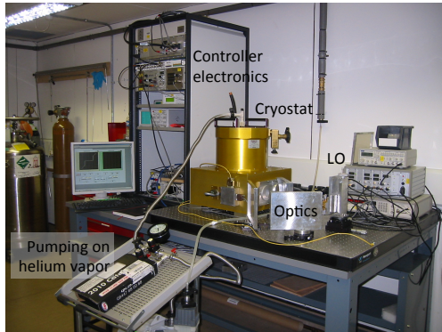
(b) Actual experimental setup without the liquid nitrogen bucket
