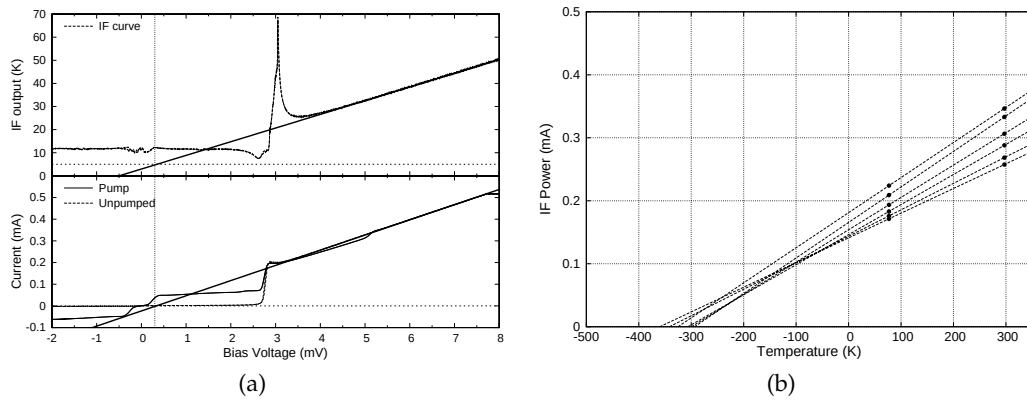
Figure 5.11: RF and IF noise contribution estimated from the unpumped IV and IF curve.
