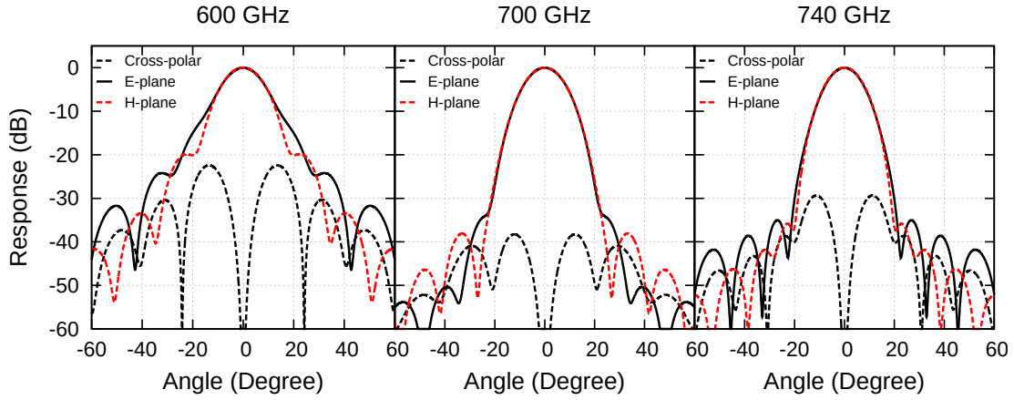
Figure 2.3: Theoretical E-, H-plane and cross-polarization beam pattern calculated using modal matching.
