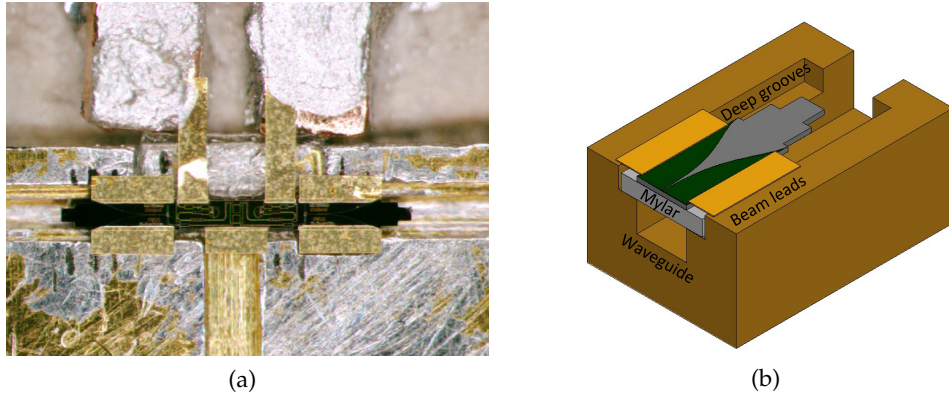
Figure 6.16: (a) Photo showing a balanced SOI device mounted on the quartz mixer block. (b) Diagram illustrate the position of the mixer chip relative to the waveguide groove.
