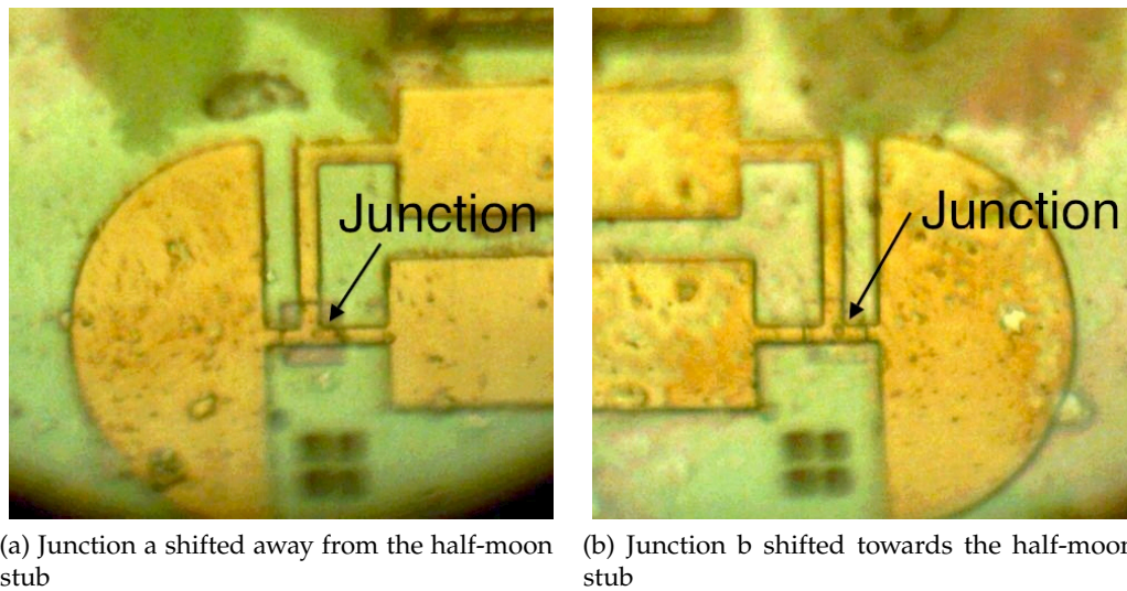
Figure 6.12: Photograph showing both junction of the same device shifted rightwards.
