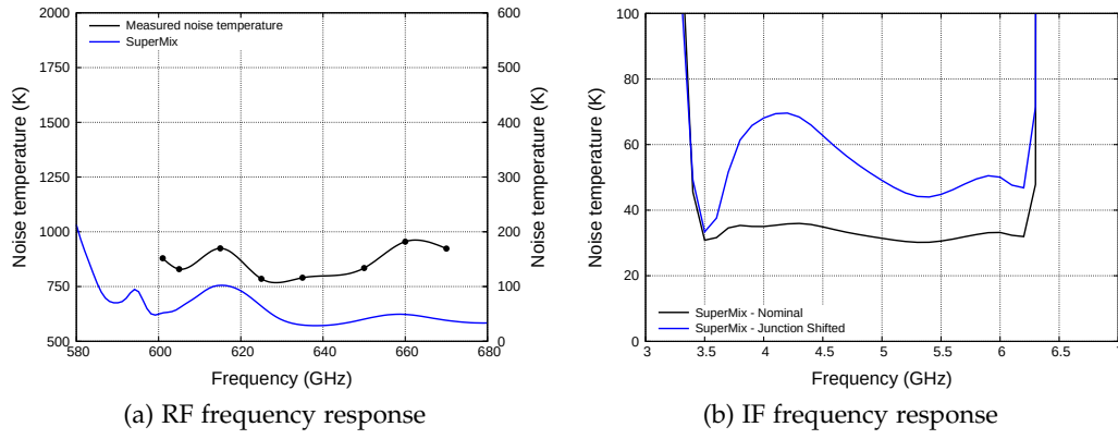
Figure 6.21: SuperMix model prediction of (a) RF response in comparison with the measured data, and (b) a two fold increase in noise temperature across the IF band due to the junction shifting and size difference.
