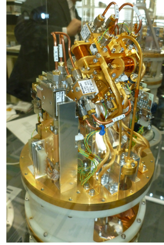
(b) ALMA Band 8 cartridge
