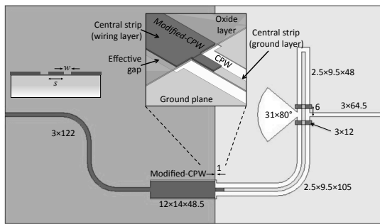
(a) Slotline to microstrip transition
