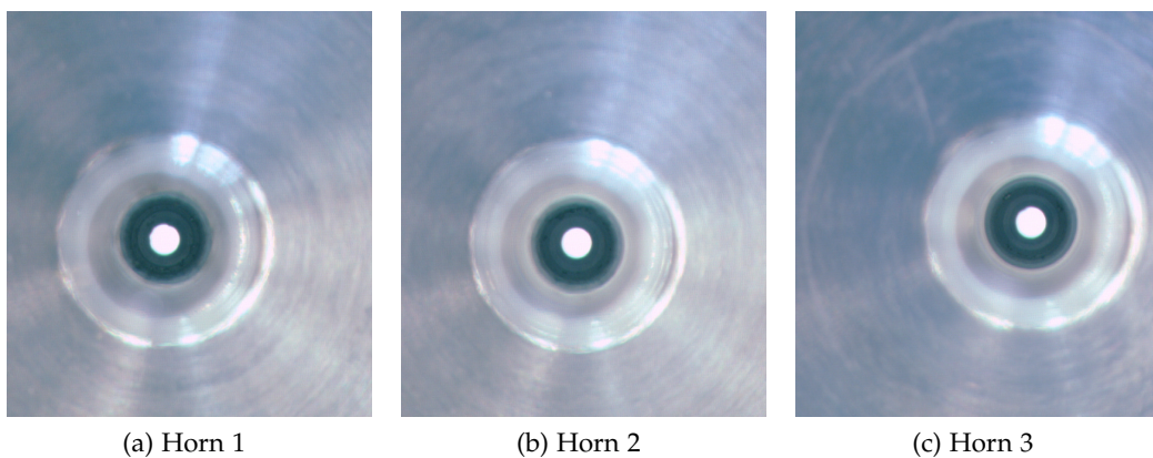
Figure 2.11: Microscope photos showing the lateral misalignment of the horns from second fabrication run.
