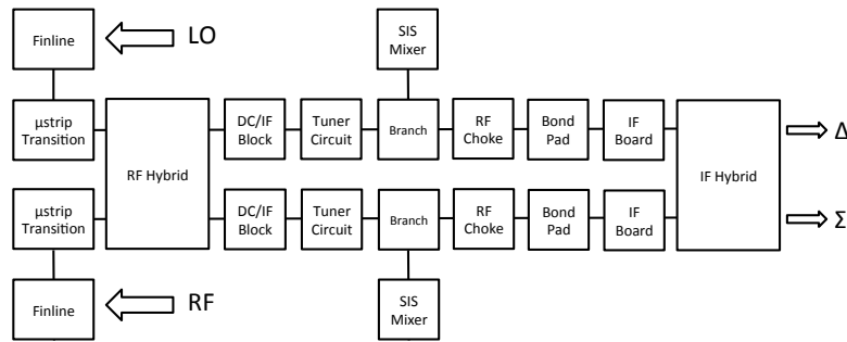
Figure 6.8: Block diagram shows the various components included in the SuperMix simulation.
