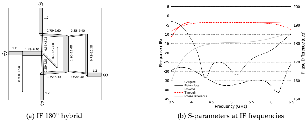
Figure 6.5: (a) Image (courtesy of P. Grimes) shows the layout of the 180^\circ IF hybrid, where Port 2 & 3 are the input port, while port 1 is the sum and port 4 is the difference port. (b) The S-parameters and the phase difference between the sum and difference port of the hybrid across the designed IF band.
