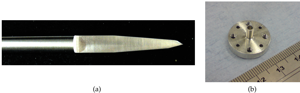
Figure 2.4: (a) The high speed steel machine tool used to fabricate the multiple flare-angle horns. (b) A prototype of 700 GHz smooth-walled horn made by direct milling into an aluminium block.
