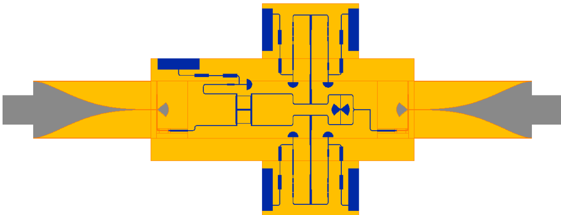
Figure D.7: The layout of the sideband separating SIS mixer chip.
