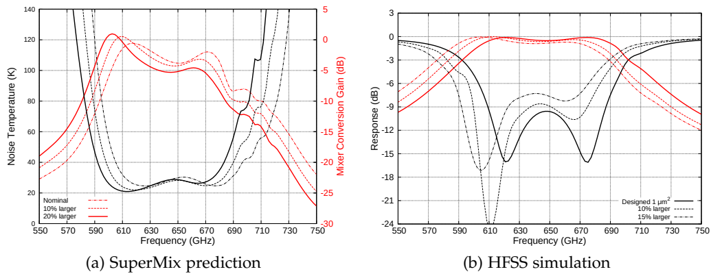
Figure 5.7: SuperMix and HFSS simulating the effect of a direct quartz mixer design with larger than designated junction size.
