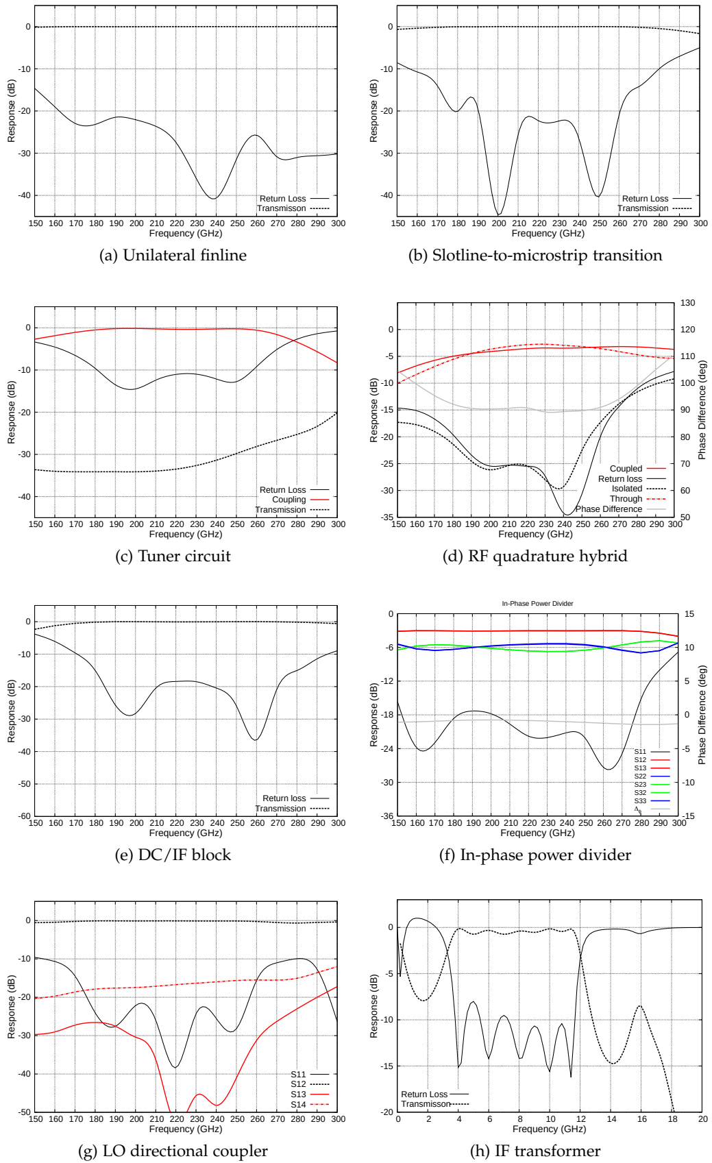
Figure D.1: Scattering parameters describing the performance of each circuit component simulated using HFSS. In general, all components show good performance from 180 GHz to 260 GHz.
