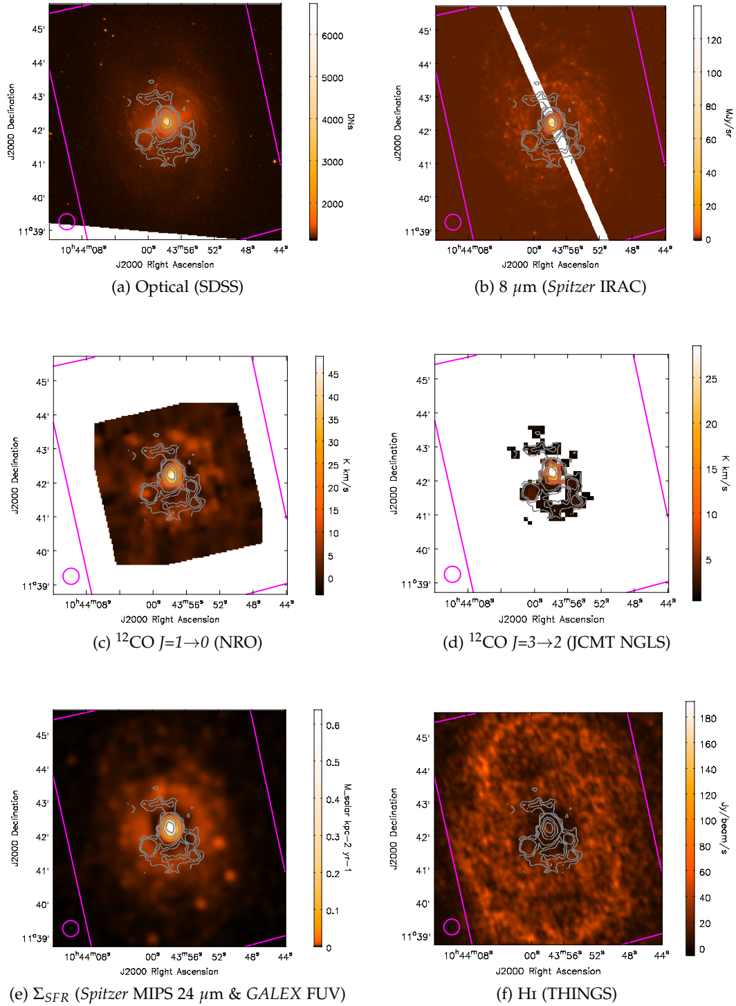
Figure 10.2: Contours of the ^{12}\text{CO}\ J=3\rightarrow2 data of NGC3351 overlaid on the corresponding ancillary images from the archives. The contour levels are 0.43 ( 3\sigma ), 0.86, 1.29, 5.0, 10.0, 20.0 and 30.0 K km s ^{-1} (temperature in T_{\text{mb}} ). In all panels, a magenta box is drawn to show the region mapped by HARP-B, and a magenta circle to indicate the 14.5'' angular resolution of the ^{12}\text{CO}\ J=3\rightarrow2 data. All images are oriented North up and East to the left. The 8\ \mu\text{m} image is affected by Muxbleed, hence the affected area is blanked out. The image representing \Sigma_{\text{SFR}} had been convolved to the HARP-B beam size.
