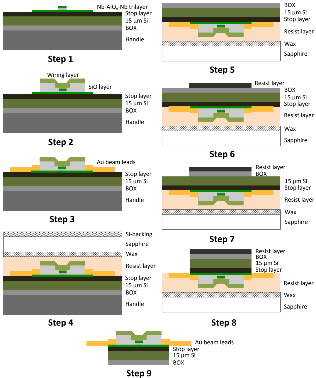
Figure 5.2: Drawing depicting the important stages involved in the fabrication of SIS mixers on a 15 μm thick SOI substrate.
