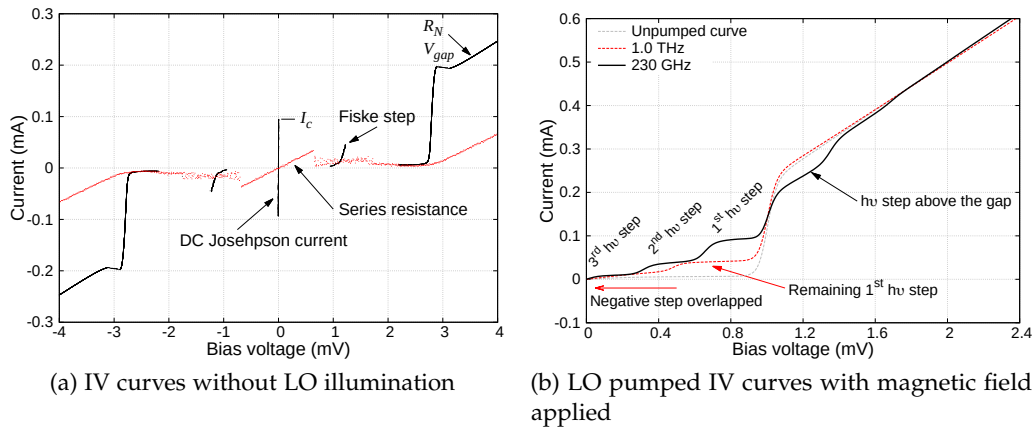
Figure 3.2: (a) Black curve: Typical current-voltage (IV) characteristic curve of an SIS junction measured in a current-biased mode showing various features. Red curve: IV curve of an SIS junction inflicted with a series resistance. (b) IV curves under illumination of 230 GHz and 1 THz LO signal showing the ordinary photon steps and the effect of negative step wrapping, respectively.
