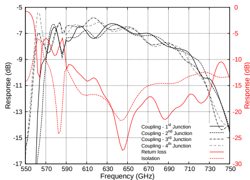
(a) The coupling and return loss from the LO port and its isolation from the RF port
