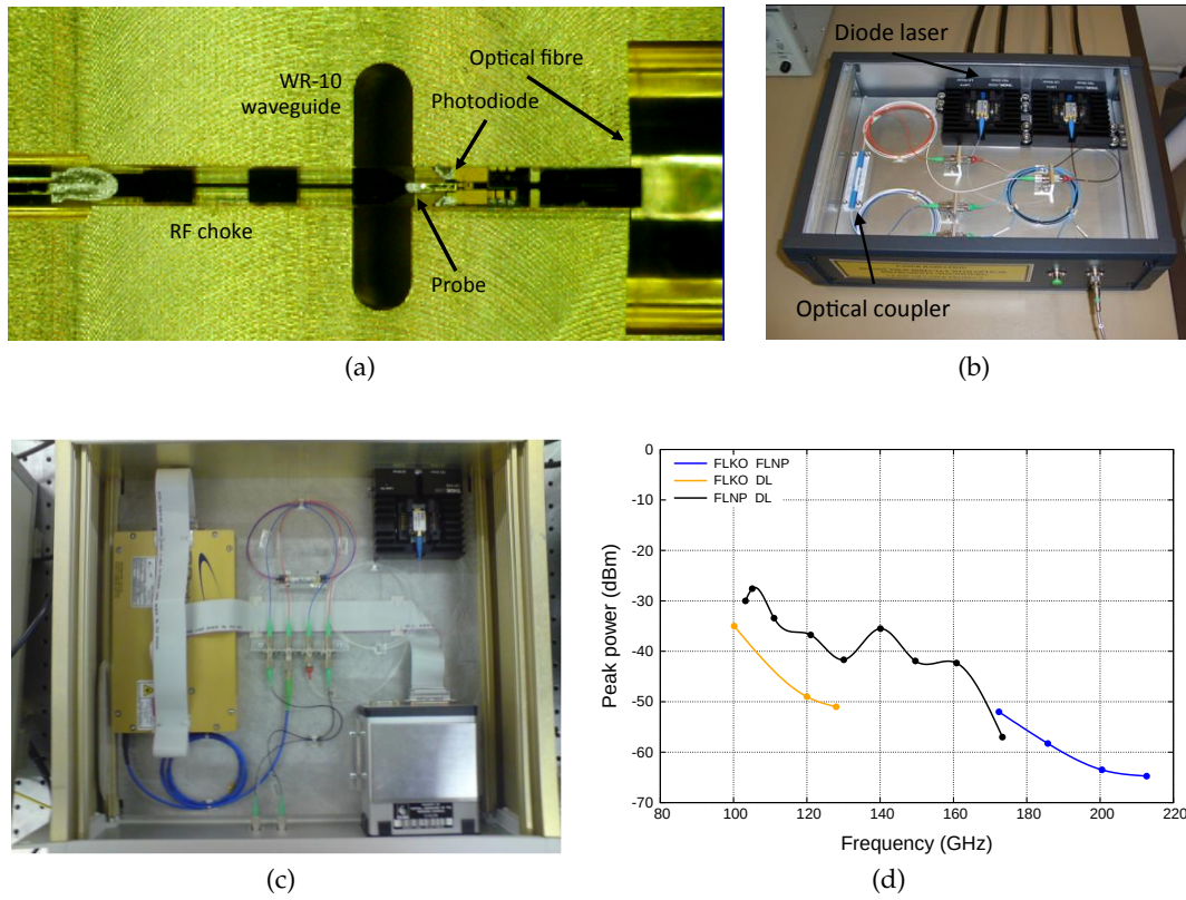
Figure 9.1: (a) Internal structure of a photomixer block. (b) System setup consisting two distributed feedback (DFB) diode lasers generating a GHz frequency source. (c) An NP Photonic fibre laser enclosed together with a DFB diode laser. (d) The output power of the photomixer plotted against the down-converted frequencies.
