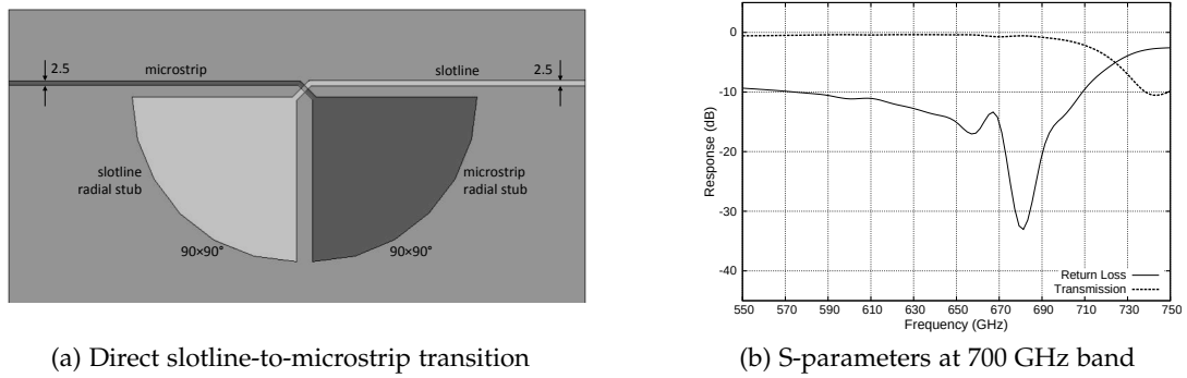
Figure 4.3: Layout of the direct slotline-to-microstrip transition. Figure (b) shows the return loss and coupling efficiency across the designated RF band for the SOI design. The dimensions for the radial stubs are in radius ( \mu\text{m} ) \times angle ( ^\circ ).
