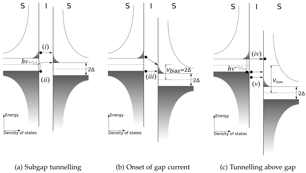
Figure 3.1: Energy level diagrams illustrating how the potential difference and the absorption of photon energy influencing the magnitude of tunnelling current at various biasing stages. (i) Leakage current. (ii) Photon-assisted tunnelling before V_{gap} . (iii) Sudden rise in current at V_{gap} . (iv) Current suppression above the gap due to photon-absorbed quasiparticle reduces the number of empty state at the counter-electrode. (v) Linear increase in tunnelling current.
