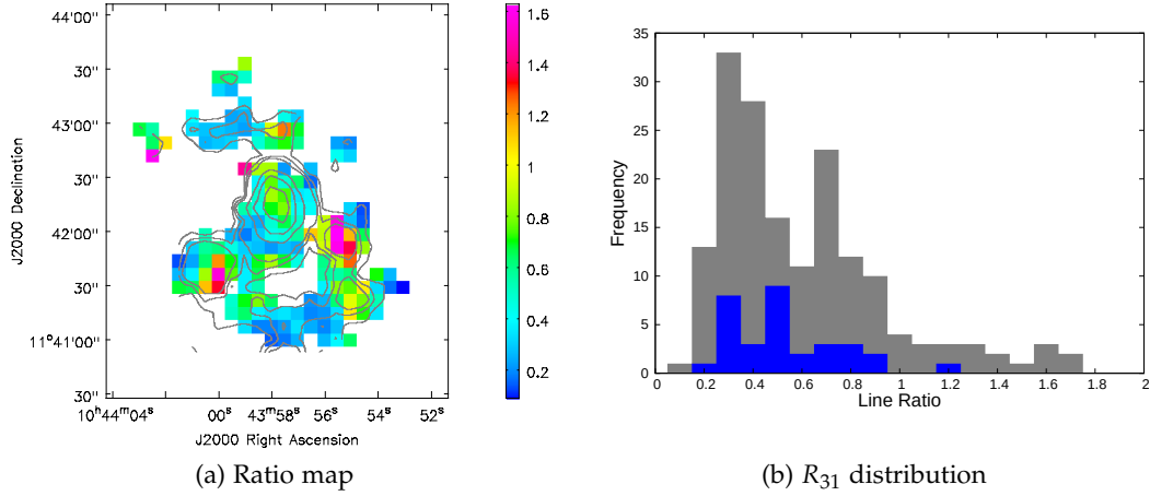
Figure 10.5: Same as Figure 10.4 but for NGC 3351. Ratio map and R_{31} distribution histogram constructed using the ^{12}\text{CO } J=1\rightarrow 0 map from the NRO Atlas.
