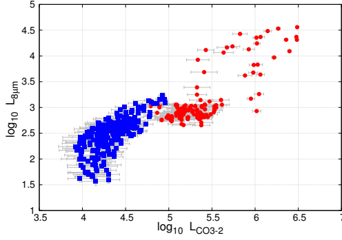
Figure 10.9: Pixel-by-pixel comparison of the ^{12}\text{CO } J=3 \rightarrow 2 luminosity with PAH 8 \mu\text{m} luminosity. Each red circle represent a pixel from NGC 3351, while each blue square corresponds to a single pixel in NGC 2976 map.
