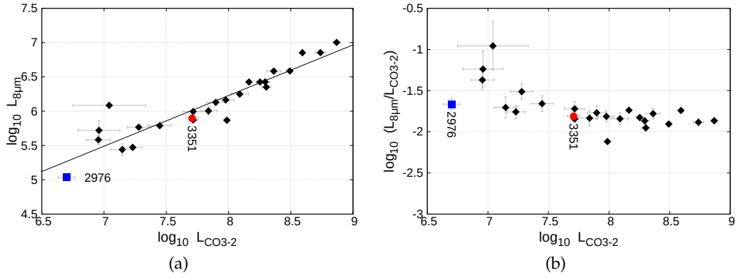
Figure 10.10: Correlation of total integrated PAH 8\mu m luminosity and the total integrated ^{12}CO J=3\rightarrow 2 luminosity of the 25 SINGS galaxies in the NGLS samples.
