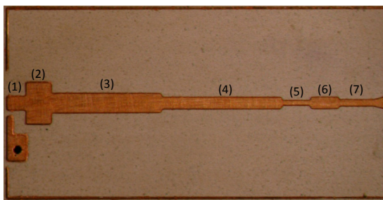
(a) Layout of the actual IF transformer board.
