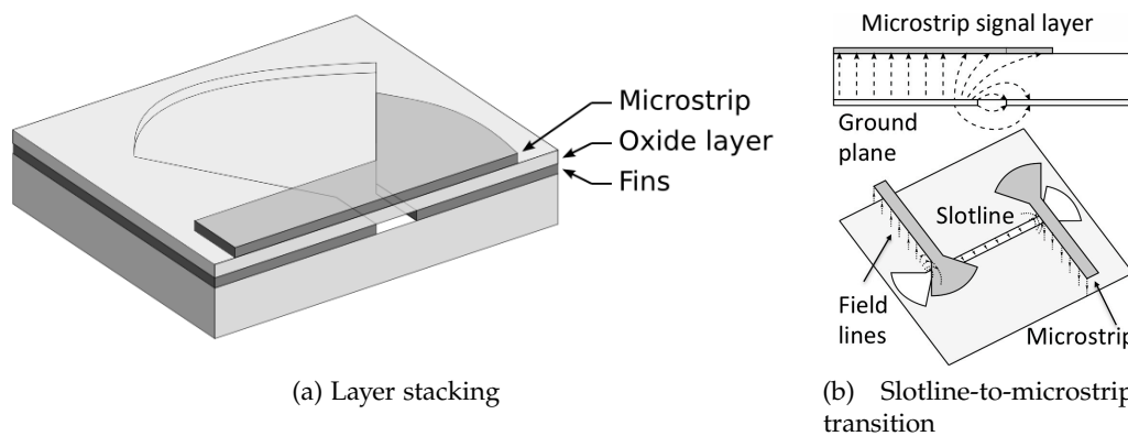
Figure 4.4: Figure (a) shows the layer structure of the transition from slotline to microstrip. Figure (b) shows how the field lines transit from the slotline to microstrip. Images courtesy of Yassin et al. (2008).
