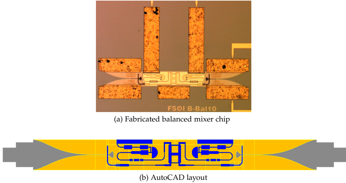
Figure 6.2: (a) Photo showing the complete balanced SIS mixer chip before the final SOI etching to define the chip size and the matching notches. (b) AutoCad drawing drafted without the dielectric layers and beam leads for clarity.
