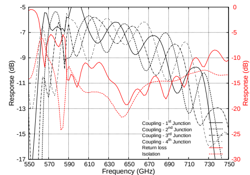
(b) The coupling and return loss from the RF port and its isolation from the LO port
