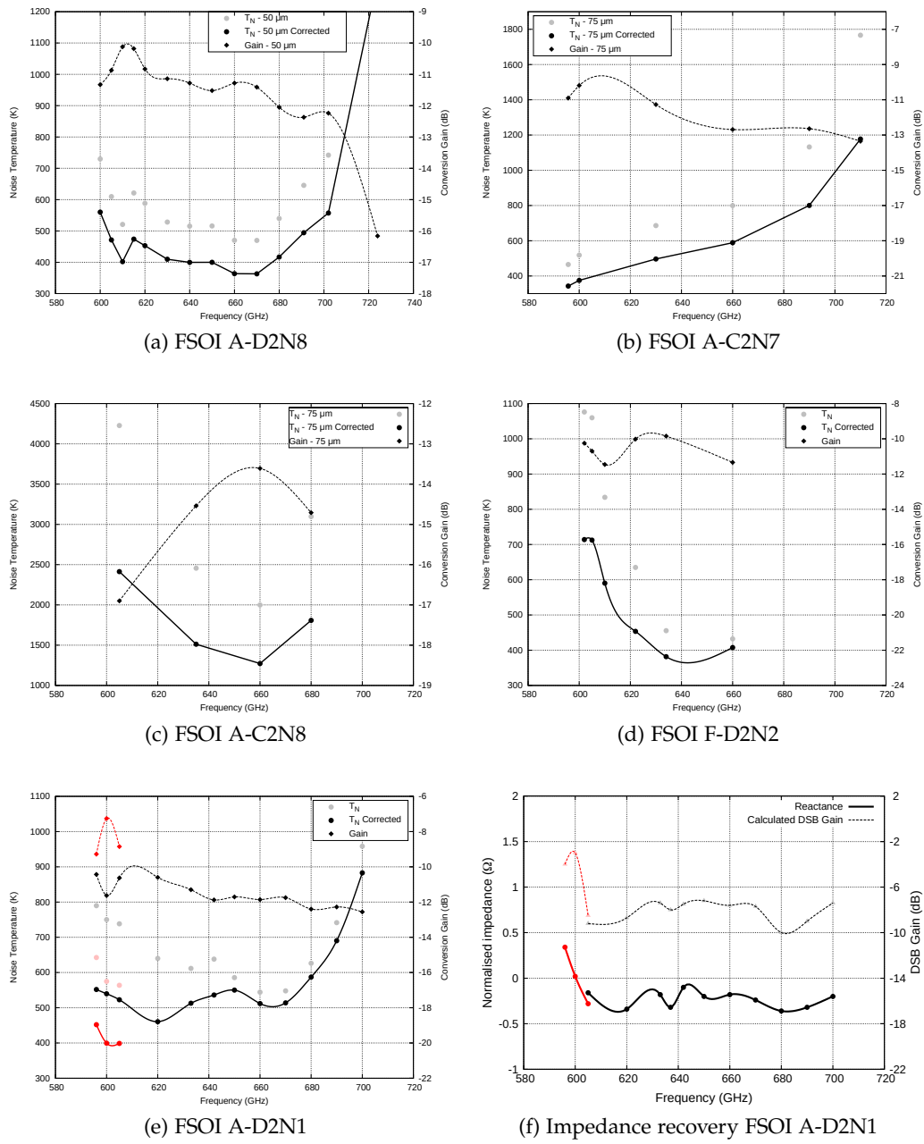
Figure 5.12: Frequency response of all SOI devices tested so far, in terms of measured conversion gain and noise temperature. The grey points are the uncorrected measurements. The red and pink points are those measured on the real first photon step i.e., between the dip shown in Figure 5.9 and the gap voltage.
