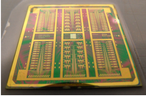
Figure 6.10: Photograph showing the layout of balanced and single-ended devices on the same SOI wafer, after the front side processing.
