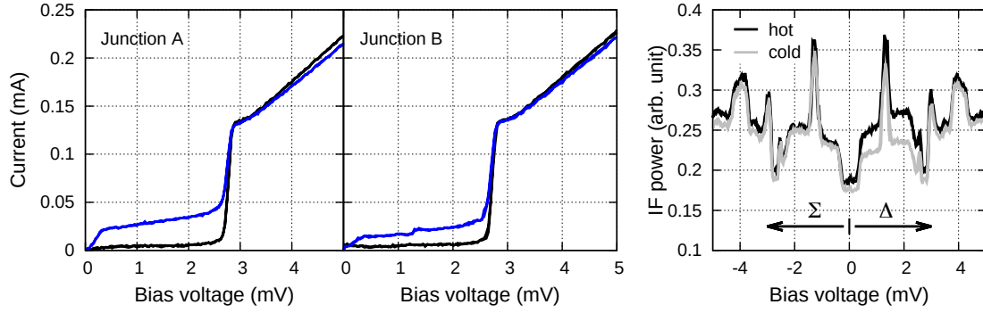
Figure 6.20: Example of IV and IF curves measured from FSOI Bal-B04.
