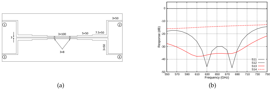
Figure 7.5: (a) Layout of the -15 dB LO directional coupler. Panel (b) shows the S-parameters of the structure across the designated bandwidth simulated using HFSS.
