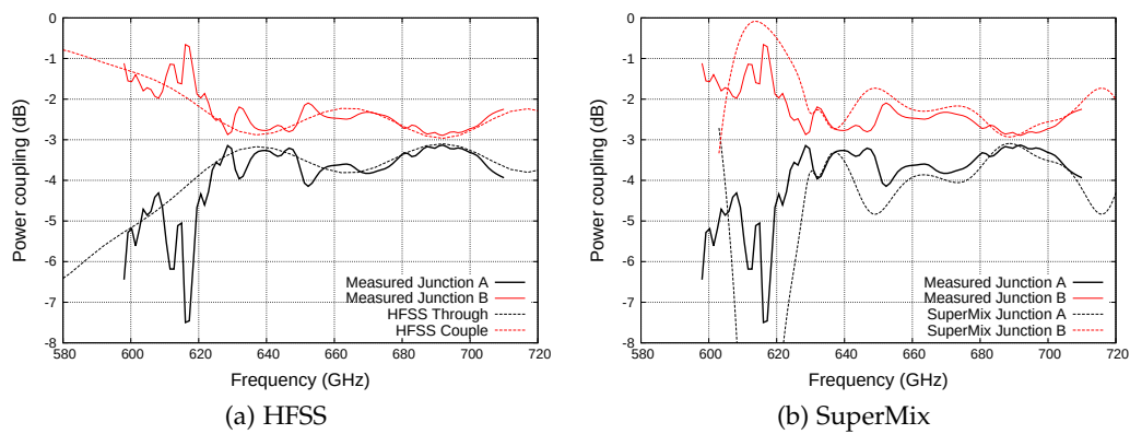
Figure 6.17: (a) Comparison of the measured performance of the hybrid to the HFSS simulations, with junction size corrected to 0.975\times and 1.025\times the designated 1\mu\text{m}^2 area (corresponding to 19.5\ \Omega and 20.5\ \Omega ). (b) Similar simulation performed using SuperMix full chip model.
