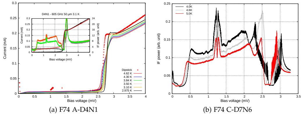
Figure A.3: (a) Slope change near the gap of the IV curve of F74 A-D4N1, which become less prominent when the device was colder. (b) The effect of the instability was only observed when the device was colder.
