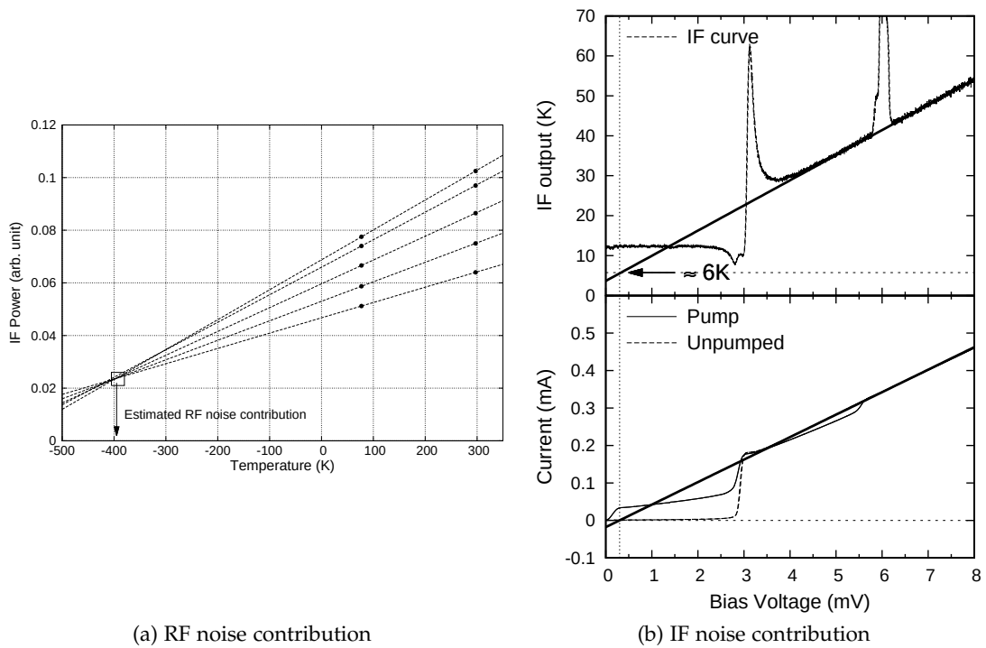
Figure 3.7: Examples showing (a) the intersecting line method for estimating the total contribution of RF losses to the mixer noise temperature, and (b) IF gain calibration method for estimating IF noise.
