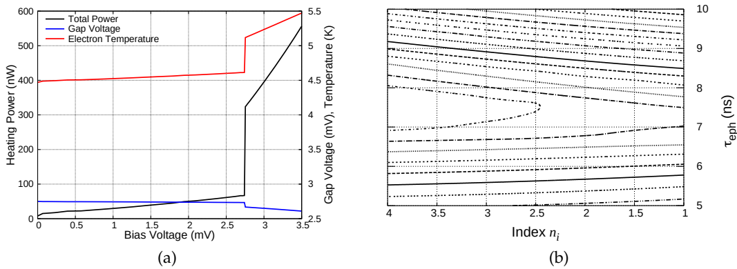
Figure 8.3: (a) The heating power coupled to the junction as a function of bias voltage. Shown together are the junction temperature and the gap voltage change corresponding to the bias voltage. (b) Contour of the error surface with different guess value of \tau_{eph} and index n_i .
