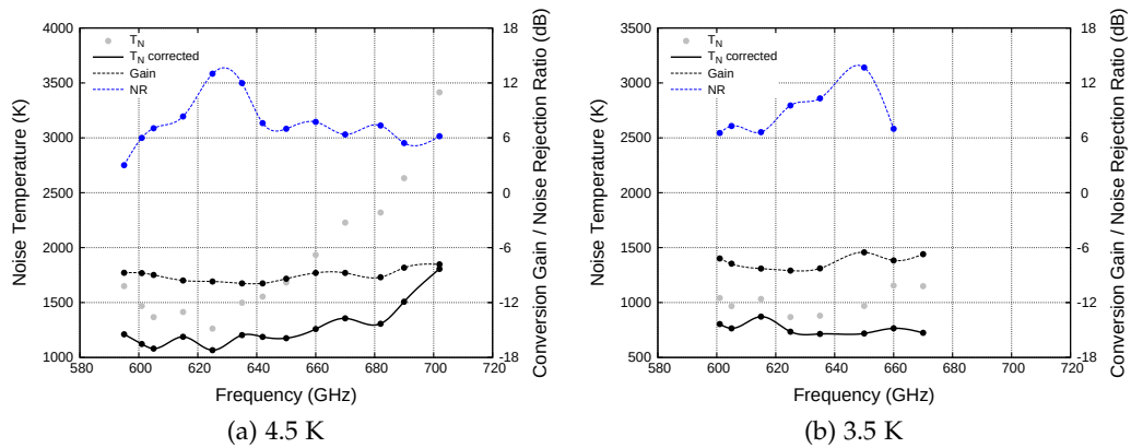
Figure 6.19: Measured noise temperature and DSB gain for FSOI Bal-B04.
