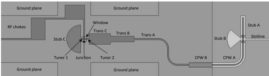
(b) Transition via coplanar waveguide
