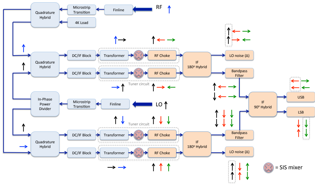
Figure 7.2: Block diagram showing the components needed for a balanced mixer design with sideband separating. The notation for various phasors are: LO in black, RF in blue, USB in red and LSB in green. All phasors are referenced to the upward pointing direction as 0^\circ and clock-wise for positive phase shift.
