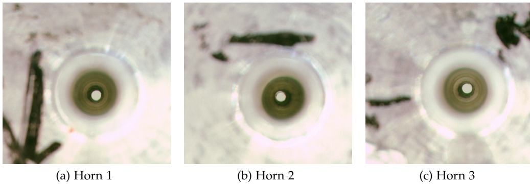
Figure 2.9: Microscope photos show the lateral misalignment between the input circular waveguide and the horn aperture of the first generation horns.
