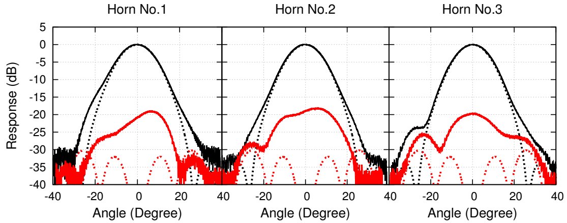
Figure 2.10: Co- and cross-polarization measurements for all three horns from the second fabrication run at 660 GHz.
