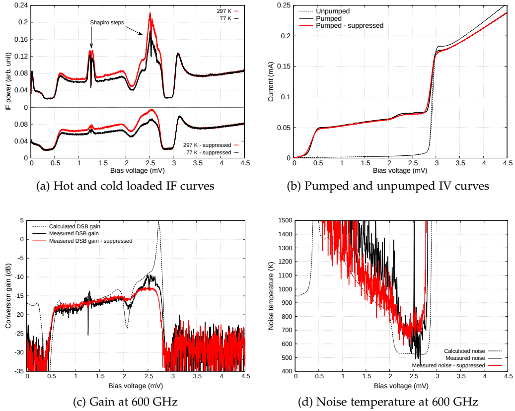
Figure A.5: (a)–(b) IV and IF response of FSOI C-D2N1 at 600 GHz showing the effect of higher magnetic field strength to suppress the Josephson features. The mixer was pumped at \alpha_1 = 0.548 . (c)–(d) Comparison with SuperMix model computed from the recovered impedance.
