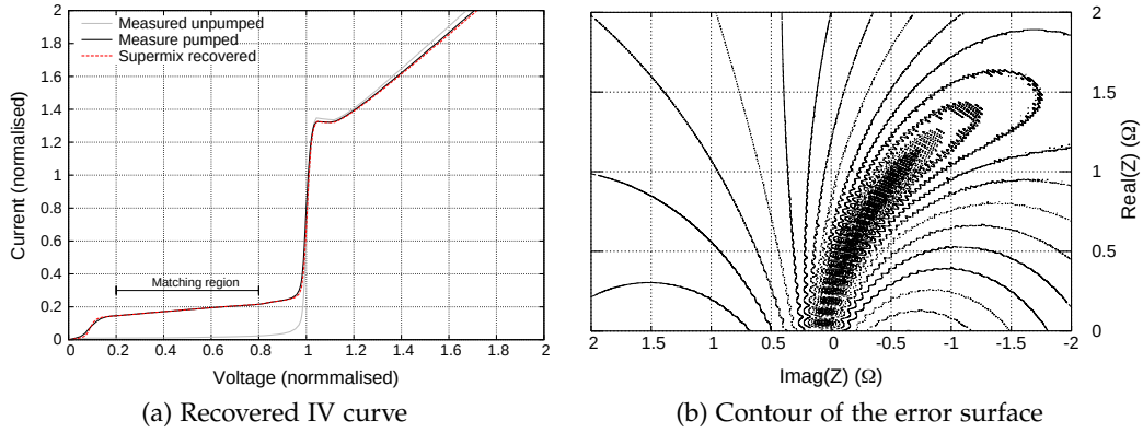
Figure 3.4: Example of embedding impedance recovery using SuperMix of a slightly capacitively tuned device.
