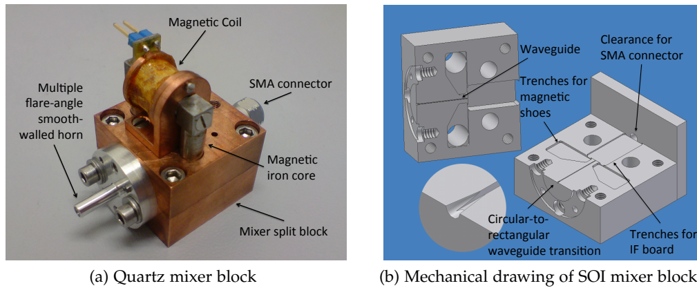
Figure 5.4: Assembly of the 650 GHz mixer block enclosing a unilateral finline mixer, fed by a multiple flare-angle smooth-walled feed horn. The superconducting coil used to suppress the Josephson tunnelling can be clearly seen on top of the block. The butterfly-wing structures are used to hold the magnetic shoes that direct the magnetic field from the coil, fed by the two iron cores on top of the mixer block. The IF output will be tapped from the IF board using standard SMA connector at the back of the mixer block. The IF board is placed in a trench immediately after the rectangular waveguide.
