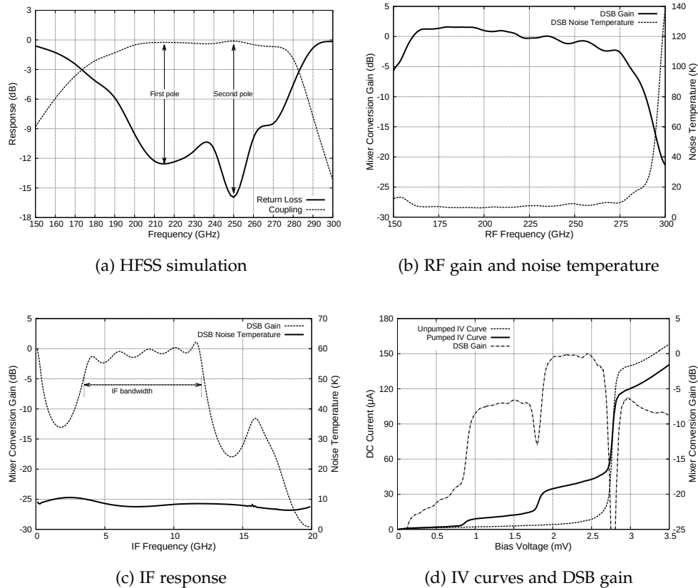
Figure D.2: HFSS and SuperMix simulations showing the predicted behaviour of the complete single-ended mixer chip design, with the following settings: bias voltage at 2.2 mV, IF frequency at 8 GHz, and RF frequency at 230 GHz.
