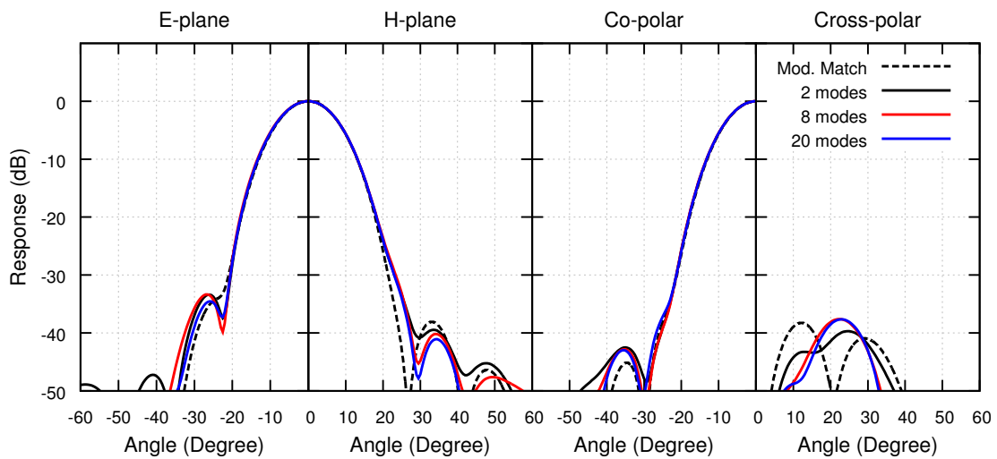
Figure 2.15: Far-field patterns of 230 GHz smooth-walled horn with 2, 8 and 20 modes, compared with the results from HornSynth .
