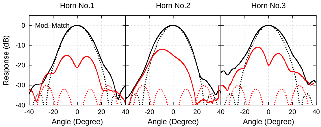
Figure 2.8: Measurements of co-polar and cross-polar pattern for the first generation of horns, compared with modal matching predictions. The solid curves are the measured data while the dotted curves are computed patterns. The black curves represent the co-polar patterns, while the red curves correspond to the cross-polar patterns.
