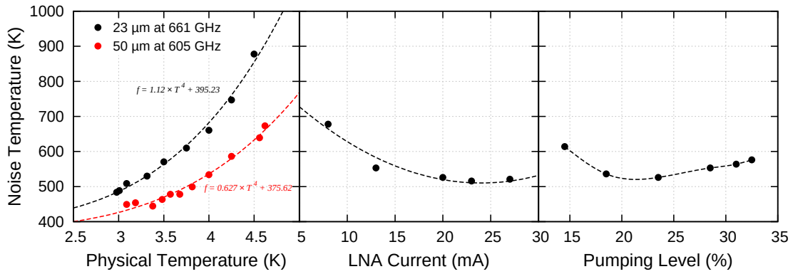
Figure A.1: All the data were taken using the quartz device F74 A-D4N1. (a) The effect of temperature influencing the measured noise temperature at a constant LO pumping level. (b) The effect of current drawn by the cryogenic amplifier influencing the noise temperature performance, at 661 GHz with a 23 \mu\text{m} beam splitter at a constant LO pumping level. (c) The effect of LO pumping level, at 661 GHz with 23 \mu\text{m} beam splitter.
