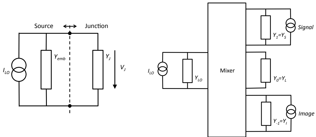
(a) Radiation source coupled to a junction as load admittance
