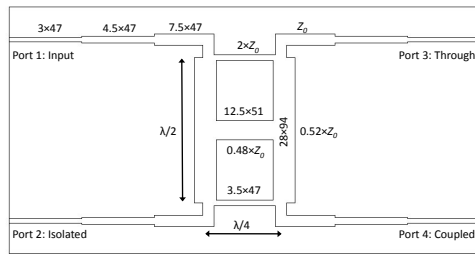
(a) Quadrature hybrid
