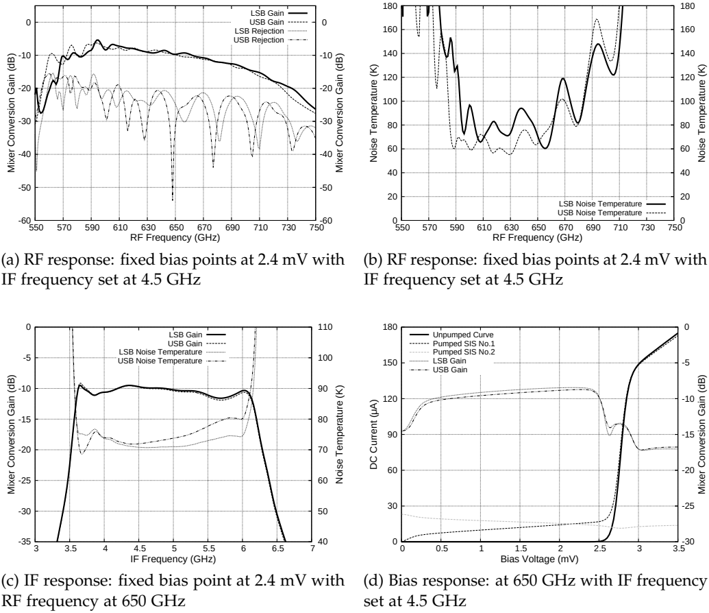
Figure 7.9: SuperMix simulations showing the predicted behaviour of the final design of the balanced with sideband separating mixer chip.
