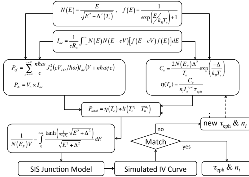
Figure 8.2: Diagram showing the flow of the method used to recover the \tau_{eph} and index n_i .
