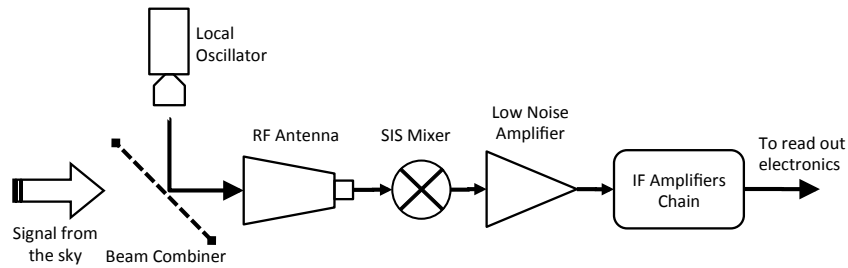
(b) Architecture of a heterodyne receiver
