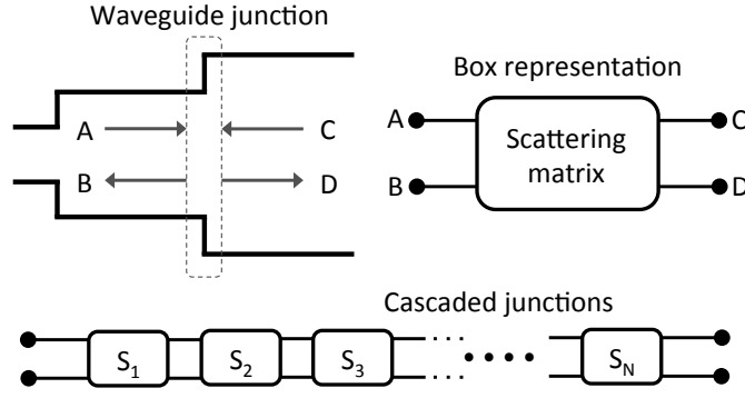
Figure 2.2: Diagram illustrating the scattering matrices used to model a feed horn.
