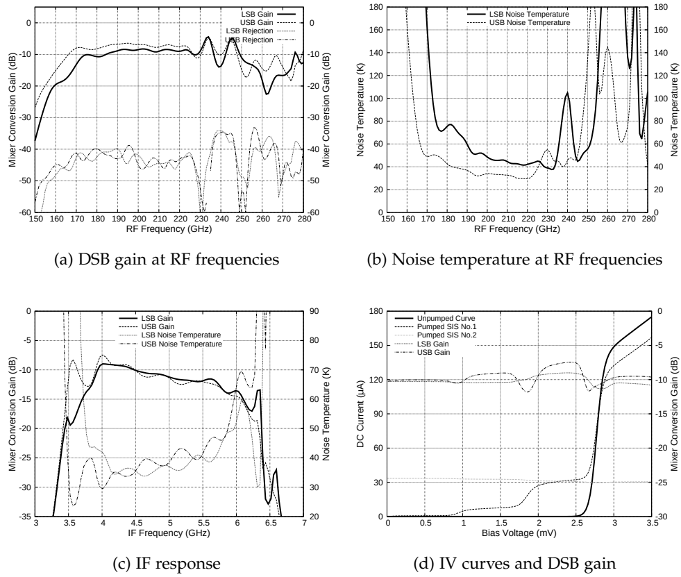
Figure D.6: SuperMix simulations showing the predicted behaviour of the complete sideband separating SIS mixer chip design. The simulation was carried out with the following settings: bias voltage at 2.4 mV, IF frequency at 4 GHz, and RF frequency at 220 GHz.
