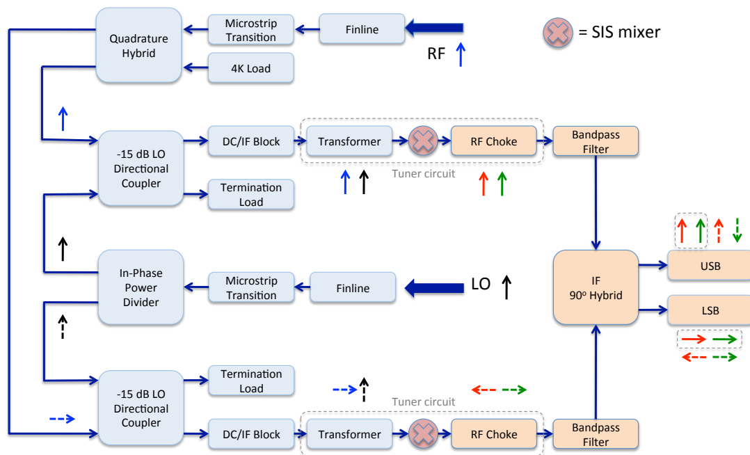
Figure 7.1: Block diagram showing the components needed for a sideband separating mixer. The notation for the various phasors are: LO in black, RF in blue, USB in red, LSB in green, upper branch IF in solid arrow, and lower branch IF in dashed arrow. All phasors are referenced to the upward pointing direction as 0^\circ and clockwise for a positive phase shift.
