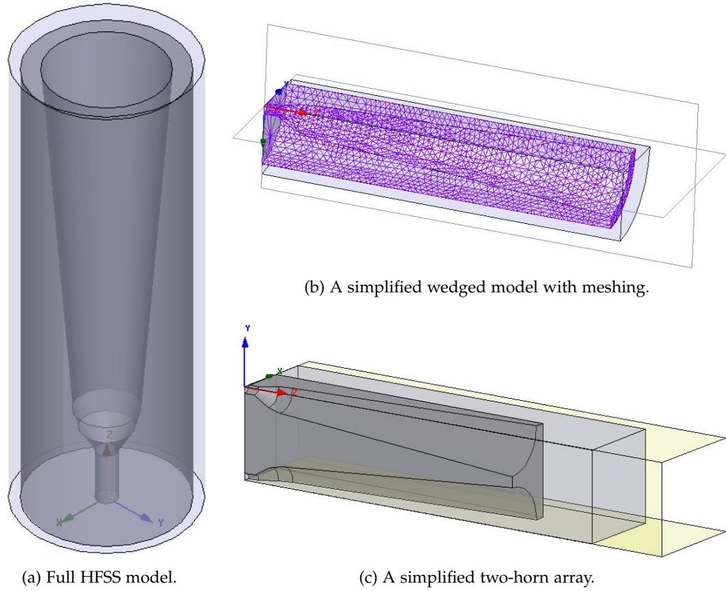
Figure 2.13: Examples of HFSS model of multiple flare-angle smooth-walled horn with the free space boundary one \lambda away from the feed horn.
