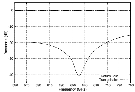
(b) S-parameters at 700 GHz band
