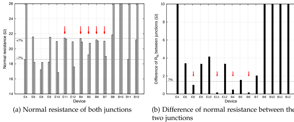
Figure 6.11: Normal resistance of all the surviving SOI balanced mixers that had both junctions fabricated.
