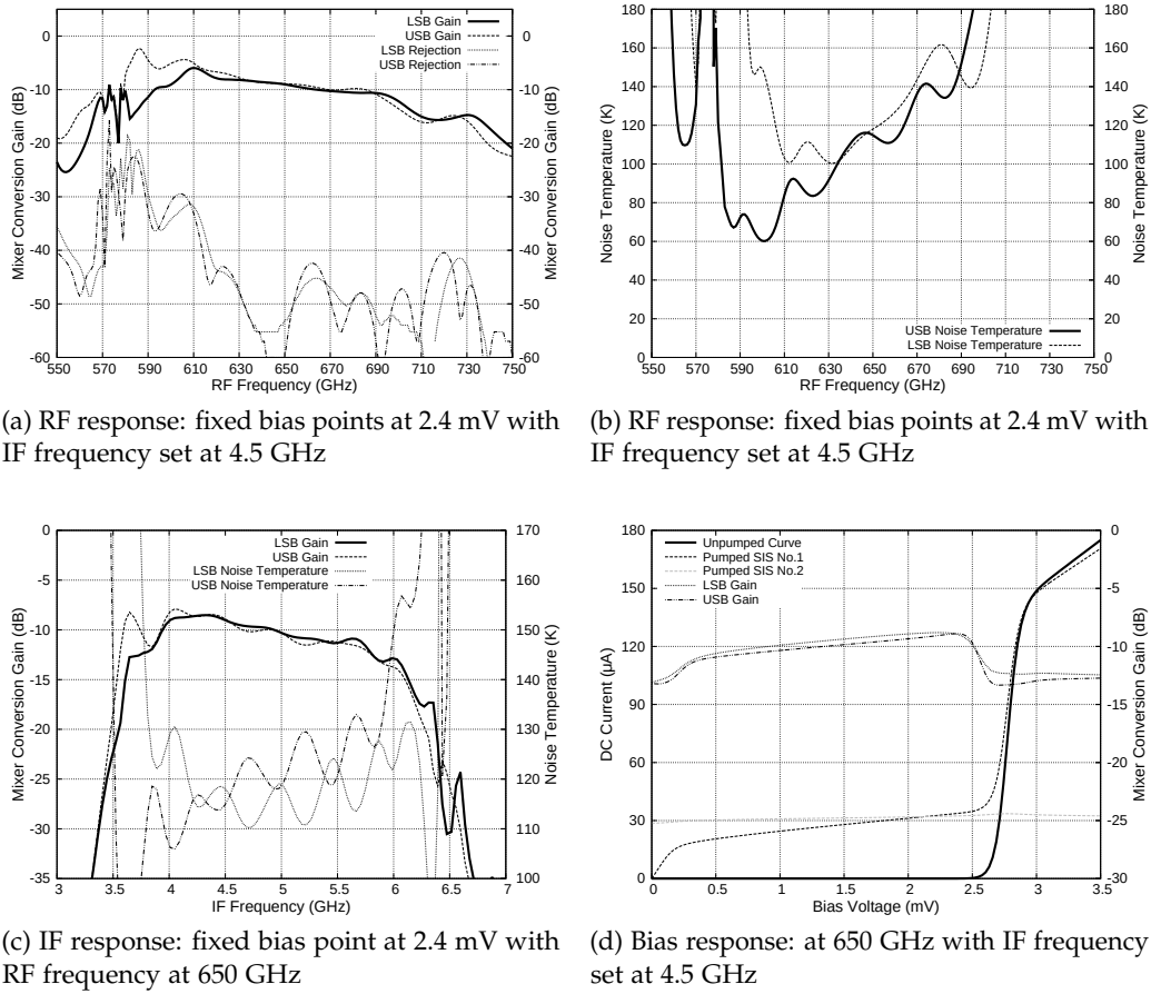
Figure 7.7: SuperMix simulations showing the predicted behaviour of the final design of the sideband separating mixer chip.
