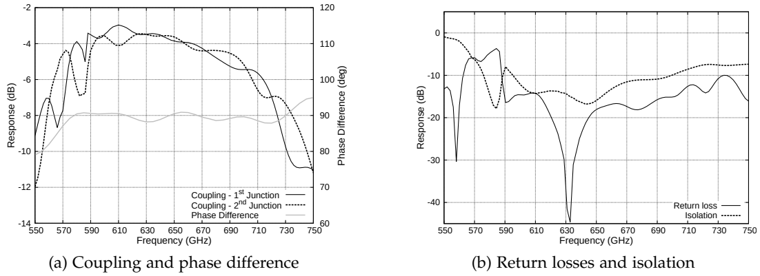
Figure 6.7: Ansoft Designer simulations of the full balanced chip by importing various S-parameters from HFSS. The phase difference is adapted from HFSS simulation with only the quadrature hybrid, DC/IF block and the tuner circuits.
