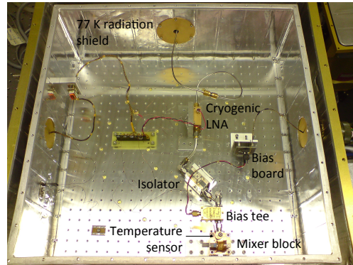
(c) Working area of the Dewar
