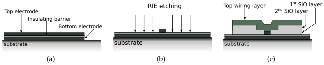
Figure 5.1: Diagrams illustrating the various photolithography steps used in fabrication of the SIS devices.
