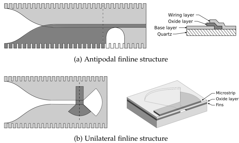
Figure 1.5: Two different types of finline taper. The diagram is not drawn to scale. Image courtesy of Grimes (2006).
