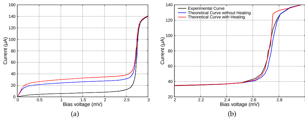
Figure 8.1: (a) The measured IV curve for different LO pump levels. (b) The matching of simulated IV curves with and without the heating effect with the experimental IV curve.
