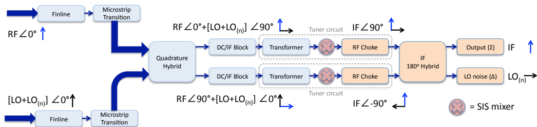
Figure 6.1: Block diagram showing the components needed for a balanced mixer design. The phasors for the LO components are shown in black arrows, while the RF phasors are in blue. The 0^\circ phase is referenced to the upward pointing direction and clockwise for positive phase shift.
