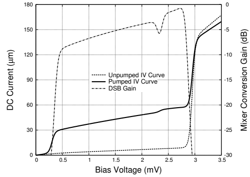
(e) Bias response for direct-mixers (SOI substrate)
