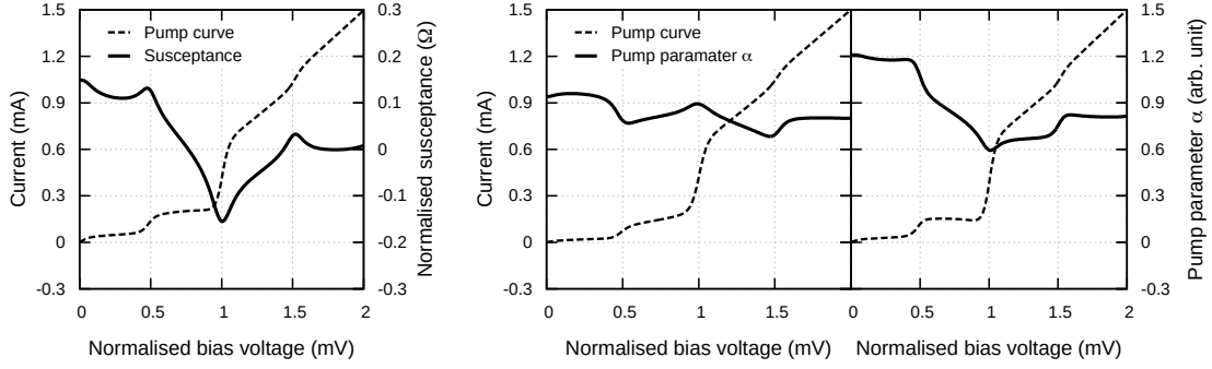
Figure 3.5: (Left panel) Examples showing the pumping level and the normalised susceptance of a tuned SIS mixer pumped at 345 GHz. (Right panel) show the pumped curves and how the pump parameter for a slightly capacitive (left) and a slightly inductive (right) SIS mixer varies against the bias voltages.
