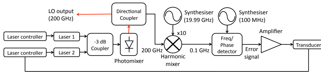
Figure 9.4: Graphical description of phase-locking two lasers.
