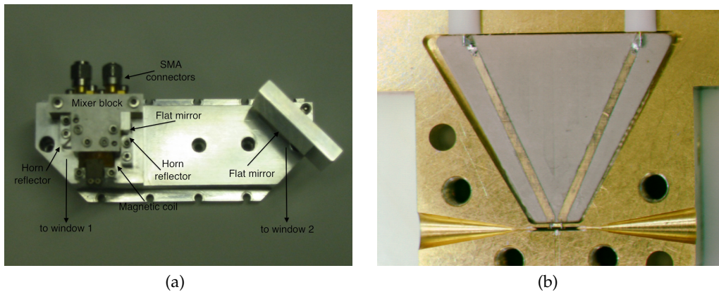
Figure 6.15: (a) Photograph showing the mixer block and the ancillary relay optics affixed on the bracket. (b) Internal view of the mixer block, with two back-to-back Pickett-Potter horn fabricated as part of the mixer block.
