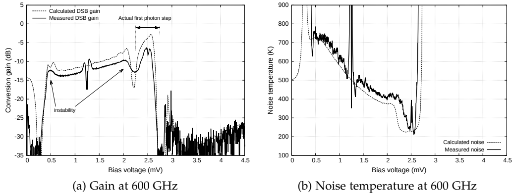
Figure 5.10: Measured gain curve and noise temperature at 600 GHz in comparison with SuperMix model computed from the recovered impedance for F71 C-D7N6.
