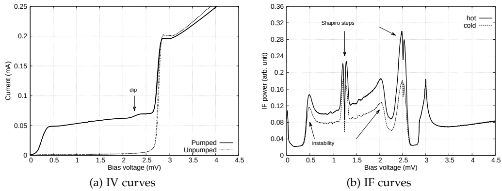
Figure 5.9: IV characteristic of the tested mixer pumped with a 600 GHz RF signal and the measured hot and cold loaded IF responses. The mixer was pumped at \alpha_1 = 0.407 .
