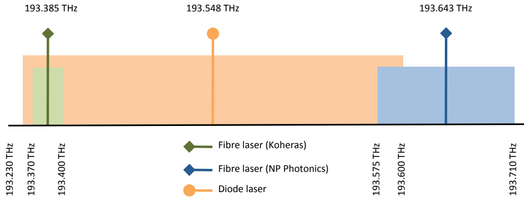
Figure 9.2: Diagram showing the centre frequency and the tuning range of the three lasers.
