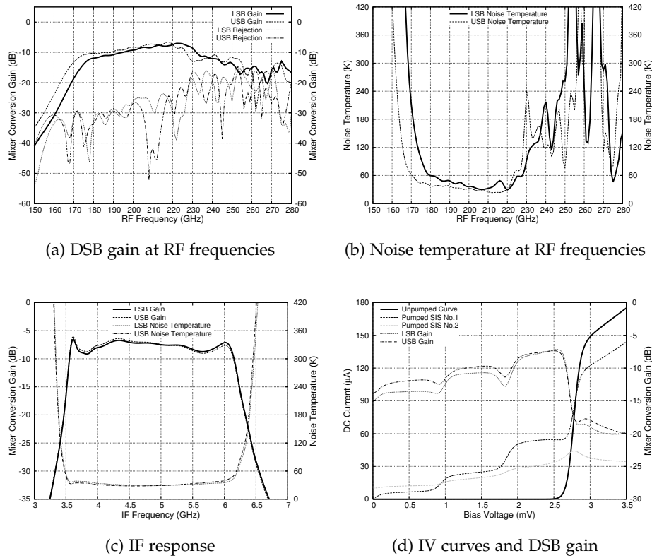
Figure D.8: SuperMix simulations showing the predicted behaviour of the complete balanced with sideband separating mixer chip design. The simulation was carried out with the following settings: bias voltage at 2.4 mV, IF frequency at 5 GHz, and RF frequency at 220 GHz.
