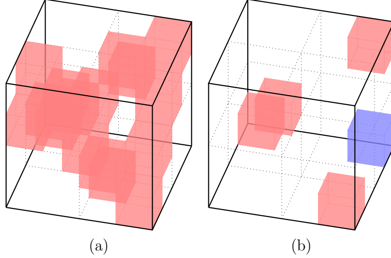
Figure 2.2: (a) The GHZ model. We represent only the red, impossible outcomes; all other entries are possible. (b) Hardy's paradox within the GHZ model; the blue outcome is possible.
