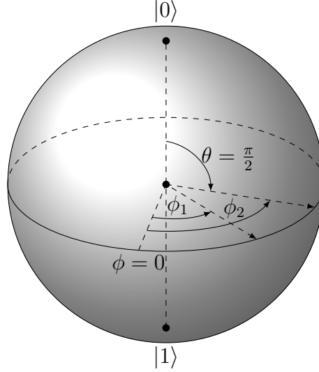
Figure 6.3: Equatorial measurements at \phi_1 and \phi_2 on the Bloch sphere.
