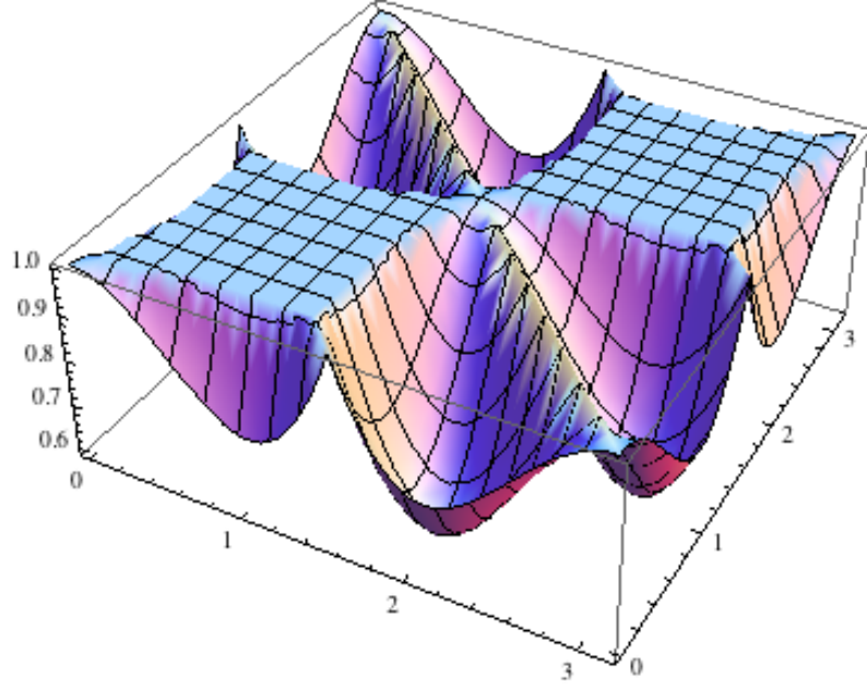
Figure 6.4: Contextuality of empirical models obtained with equatorial measurements at \phi_1 and \phi_2 on each qubit of |\phi^+\rangle .
