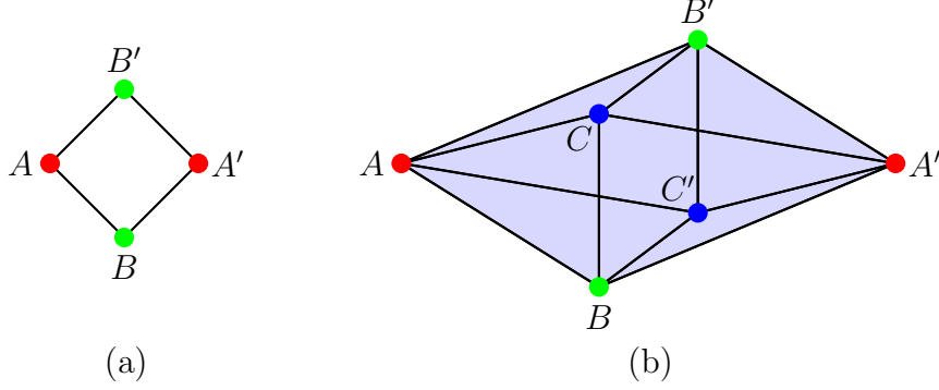
Figure 1.2: (a) The compatibility structure of the Bell-CHSH model (b) A similar tripartite measurement scenario.
