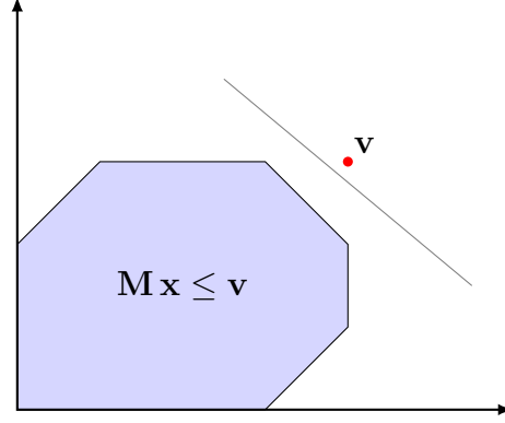
Figure 6.1: A two-dimensional analogue of the linear program for contextuality, with the image of a level set of the objective function in grey.
