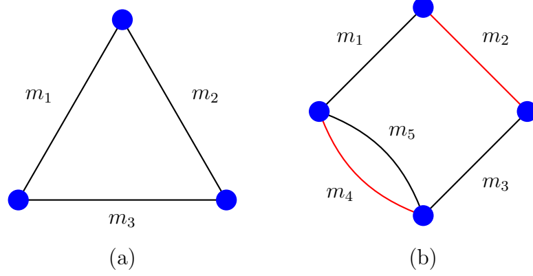
Figure 3.1: Dual (multi)graphs of chain Kochen-Specker models: (a) the contextual triangle; (b) an example with multiple edges which has a perfect matching (red).
