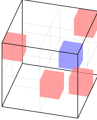
Figure 2.3: A non-Hardy (3, 2, 2) paradox. We assume that all unspecified entries are possible. This model does not contain a Hardy paradox, but is logically non-local since the blue entry cannot be completed to a deterministic grid.
