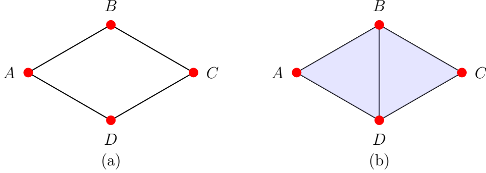
Figure 4.2: The measurement covers of example 4.3.7: (a) \mathcal{M} = \{AB, BC, CD, DA\} (b) \mathcal{M}' = \{ABD, BCD\} .
