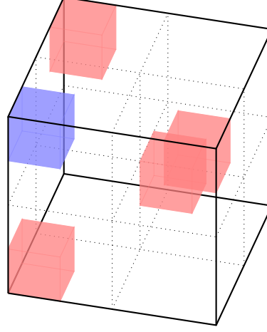
Figure 2.1: The n = 3 Hardy paradox. The blue entry corresponds to Boolean ‘1’ or ‘possible’, and the red entries to ‘0’ or ‘impossible’. The blank entries are unspecified.
