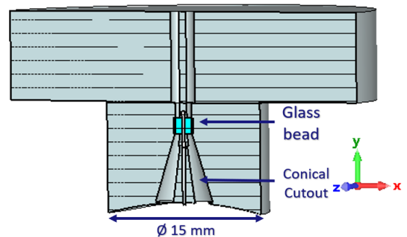
Figure 3: A simplified design of the HF BPM in CST, the button material is modelled with Aluminium, the beampipe as a perfect vacuum, and the metallic conical pickup as a perfect electrical conductor (PEC).
