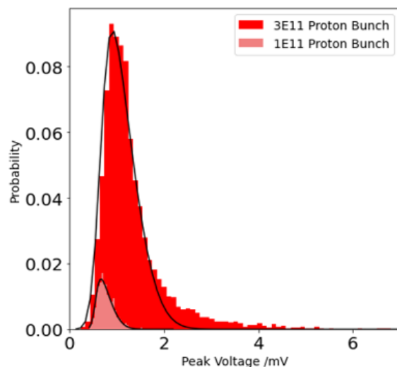
Figure 6: The distribution of the peak voltages recorded at the oscilloscope over a large number of proton shots represented with a histogram for low and high intensity proton bunches. Black curves represent a fitted probability density function to the distribution.
