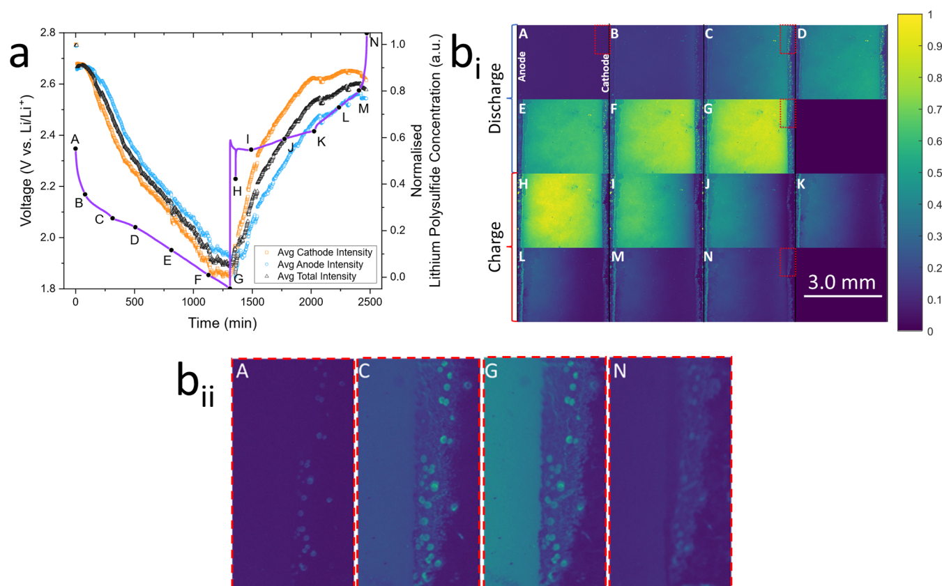
Figure 4. Cycling data (a) and optical fluorescence images ( b_i , b_{ii} ) taken during operando study of the electrolyte of a standard Li–S cell, omitting the SEI protective \text{LiNO}_3 additive, with 20\ \mu\text{M} polysulfide-sensitive PS- \text{Li}_2\text{S}_x fluorescent dye for the first cycle. ( b_{ii} ) Enlarged fluorescence images of pores within the cathode and nearby electrolyte during the first cycle at (A) open-circuit potential, (C) first discharge plateau, (G) end of discharge, and (N) end of charge.
