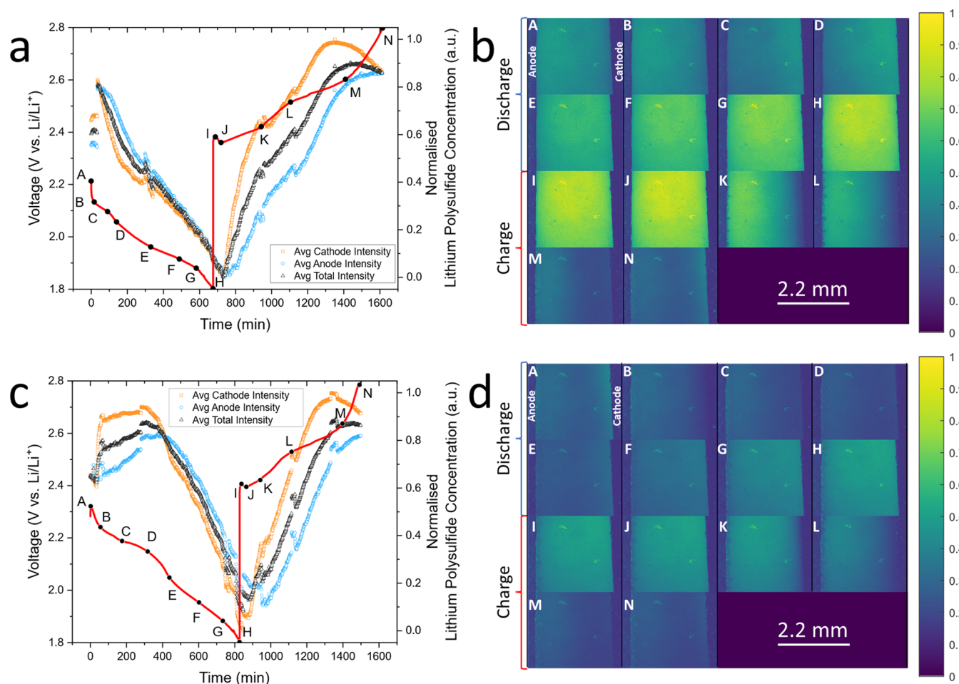
Figure 3. Cycling data (a, c) and optical fluorescence imaging (b, d) taken during operando study of the electrolyte of a standard Li–S cell, with 20 \mu\text{M} polysulfide-sensitive PS- \text{Li}_2\text{S}_x fluorescent dye for the first cycle (a, b) and the second cycle (c, d).
