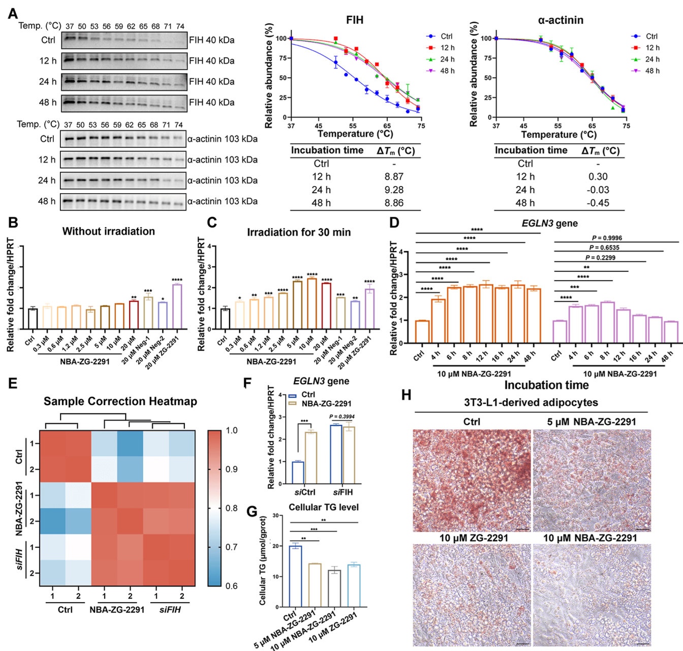
Figure 5. NBA-ZG-2291 sustainably engages with FIH and regulates the expression of FIH-dependent HIF target gene EGLN3 in Hep3B cells. (A) The CETSA assay was carried out with Hep3B cells grown in the presence of NBA-ZG-2291 (50 \mu M) for 12–48 h after 30 min of light activation (365 nm, 16 W). The intensity of the bands for grayscale analysis was referenced to the starting temperature (37 ^{\circ} C). \alpha -Actinin was the sample loading control. n = 2 ; mean \pm SD. The uncropped blot is shown in Figure S14. (B) NBA-ZG-2291 showed weak upregulation to the expression of EGLN3 without irradiation. (C) NBA-ZG-2291 showed significant and dose-dependent upregulation of the expression of EGLN3 with irradiation. (D) NBA-ZG-2291 showed long-term regulation of expression of the FIH-dependent HIF target gene after 30 min of irradiation. (E) Correlation heatmap of the NBA-ZG-2291-treated group and the siFIH group by RNA-sequencing analysis. (F) NBA-ZG-2291 showed no significant effect on EGLN3 expression when FIH was knocked down. The relative fold change with respect to DMSO treated sample is shown (with normalization to HPRT gene levels). Mean \pm SEM; n = 3 . (G) TG level of NBA-ZG-2291-treated 3T3-L1-derived adipocytes. Mean \pm SEM; n = 3 . (H) Representative Oil Red O-stained images of the control, ZG-2291-treated, and NBA-ZG-2291-treated 3T3-L1-derived adipocytes. Scale Bar, 30 \mu m. P values were analyzed by two-way ANOVA comparing with the vehicle/control group (*, P < 0.05 ; **, P < 0.01 ; ***, P < 0.001 ; ****, P < 0.0001 ). See Methods (Quantitative PCR Analysis of Gene Expression) for assay details.
