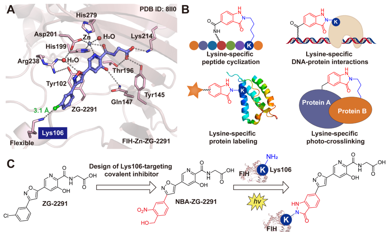
Figure 1. (A) View from a crystal structure of FIH in complex with the FIH inhibitor ZG-2291 (PDB ID: 8II0 18 ). Note that the interaction between the ZG-2291 meta -chloro group and Lys106 enables electron density for the Lys106 side chain to be clearly observed, which has been rarely observed in reported FIH structures. 18,20,31–33 (B) Previous applications of light-induced primary amines and the o -NBAs click cyclization reaction; the reaction proceeds via a nitroso intermediate (Figure S3). (C) Design of the light-induced, Lys106-targeting irreversible FIH covalent inhibitor, NBA-ZG-2291.
