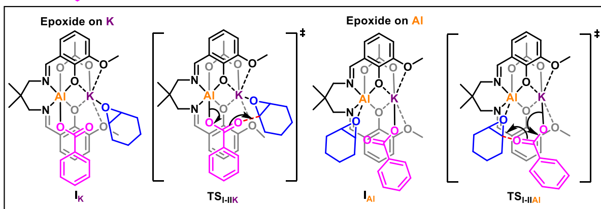
Figure S55. Computed Pathways for lowest free enthalpy TS. Reaction profile showing key intermediates and transition states computed with temperature corrections and accounting for catalyst concentration.
