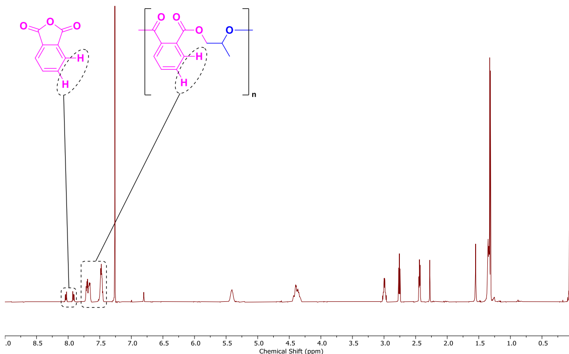
Figure S45. ^1\text{H} NMR spectrum (400 MHz, \text{CDCl}_3 , 298 K) of reaction mixture of PO and PA. Conversion of PA (%) = (\int_{7.75-7.40 \text{ ppm}} / \int_{8.10-7.40 \text{ ppm}}) * 100 . \text{TON}_{\text{Epoxide}} = \text{TON}_{\text{Anhydride}} = \text{Conv.} (\%) * 400 . Spectroscopic data is consistent with prior literature reports. 14
