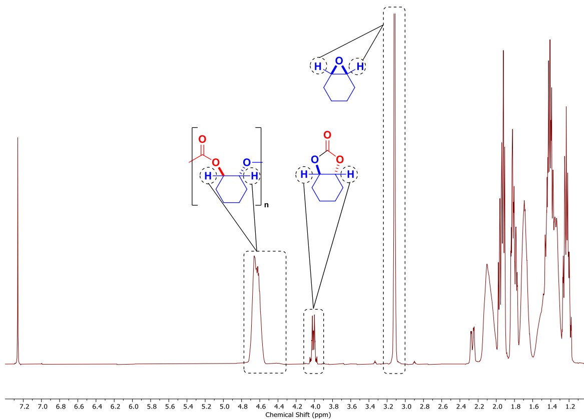
Figure S49. ^1\text{H} NMR spectrum (400 MHz, \text{CDCl}_3 , 298 K) of reaction mixture of CHO and \text{CO}_2 (20 bar). Conversion of CHO to PCHC (%) = (\int_{4.90-4.35} \text{ppm} / (\int_{4.90-4.35} \text{ppm} + \int_{3.25-3.00} \text{ppm})) * 100 . \text{TON}_{\text{PCHC}} = \text{Conv.}(\%) * 2000 . Selectivity _{\text{PCHC}} (%) = (\int_{4.90-4.35} \text{ppm} / (\int_{4.90-4.35} \text{ppm} + \int_{4.10-3.90} \text{ppm})) * 100 . Spectroscopic data is consistent with prior literature reports. 12
