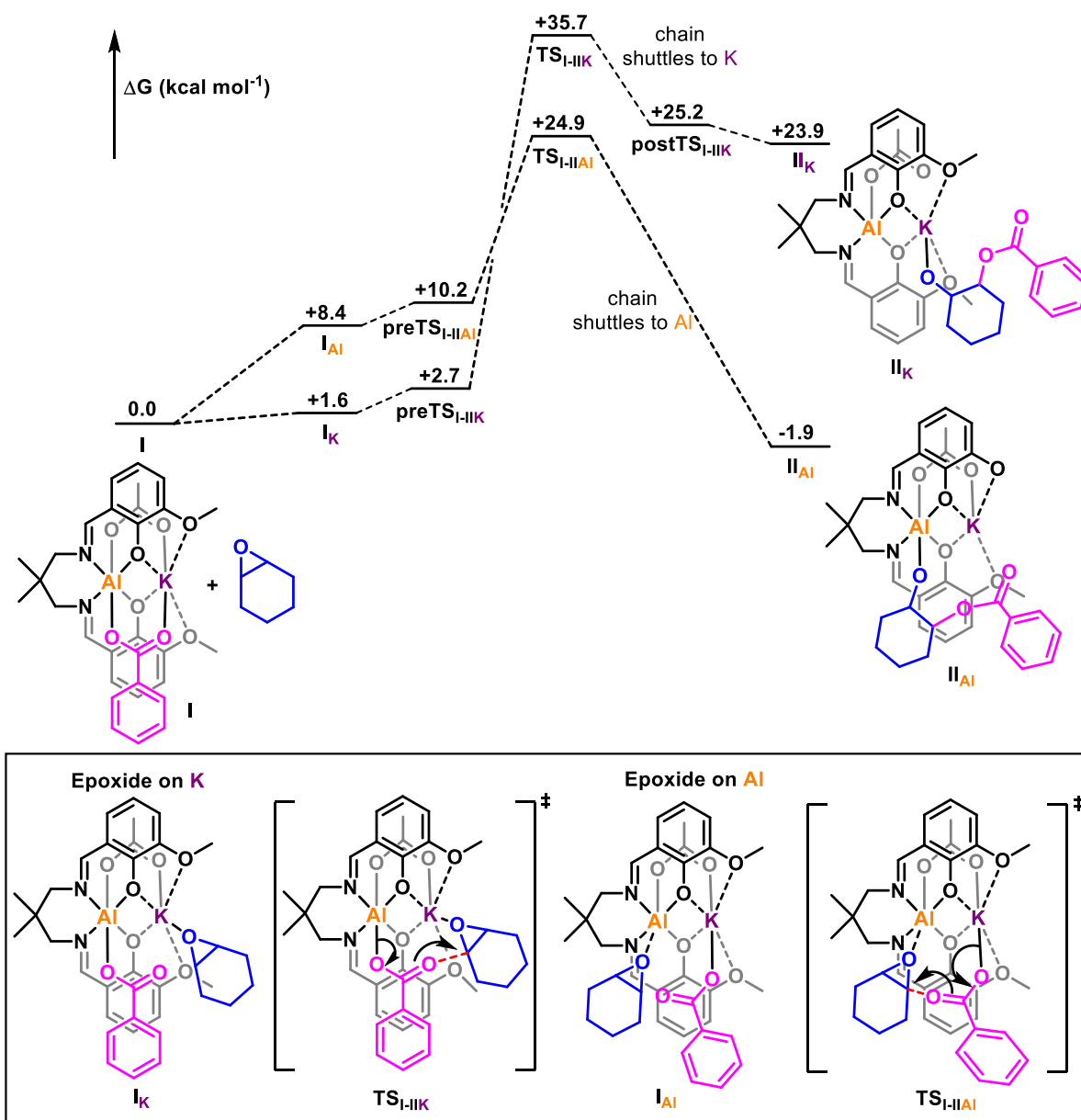
Figure S56. Computed Pathways for lowest free enthalpy TS. Reaction profile showing key intermediates and transition states computed with temperature corrections and accounting for excess epoxide.
