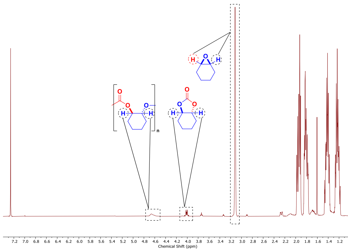
Figure S48. ^1\text{H} NMR spectrum (400 MHz, \text{CDCl}_3 , 298 K) of reaction mixture of CHO and \text{CO}_2 (1 bar). Conversion of CHO to PCHC (%) = (\int_{4.90-4.35 \text{ ppm}} / (\int_{4.90-4.35 \text{ ppm}} + \int_{3.25-3.00 \text{ ppm}})) * 100 . \text{TON}_{\text{PCHC}} = \text{Conv.}(\%) * 2000 . Selectivity _{\text{PCHC}} (%) = (\int_{4.90-4.35 \text{ ppm}} / (\int_{4.90-4.35 \text{ ppm}} + \int_{4.10-3.90 \text{ ppm}})) * 100 . Spectroscopic data is consistent with prior literature reports. 12
