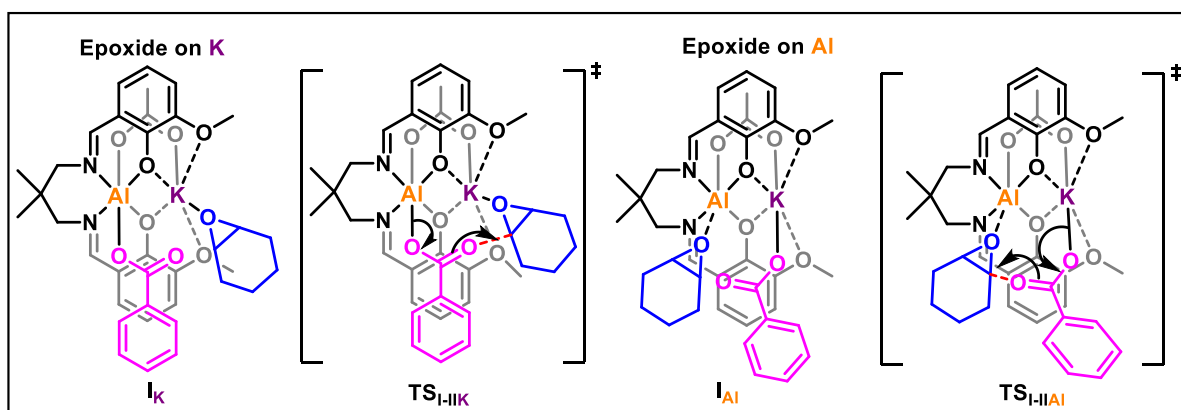
Figure S52. Computed Reaction Profile for epoxide ring-opening. \omega b97xD/C H O= 6-31+g(d,p)/K AI = 6-311+g(d)/solvent = modified THF eps=16 epsinf=1.867 (cpcm).
