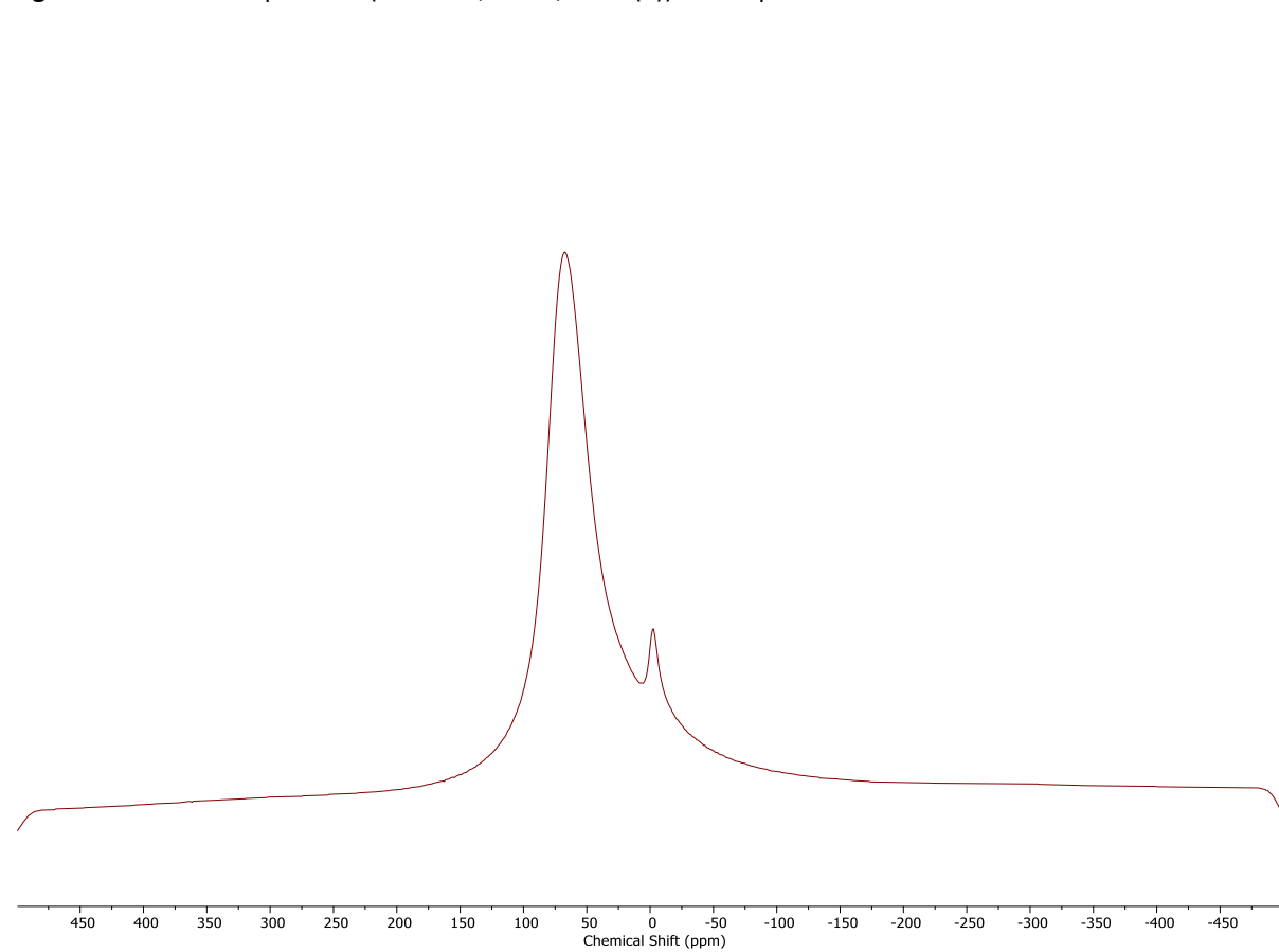
Figure S20. ^{13}\text{C} NMR Spectrum (126 MHz, 298 K, \text{CDCl}_3 (*)) of complex 4.
