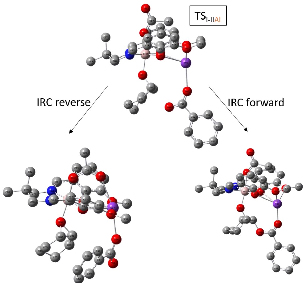
Figure S54. IRC for TS_{I-IIAI} showing connected intermediates either side. Maxpoints=50, maxcycle=40, stepsize=20
