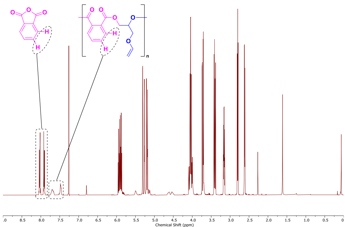
Figure S47. ^1\text{H} NMR spectrum (400 MHz, \text{CDCl}_3 , 298 K) of reaction mixture of AGE and PA. Conversion of PA (%) = (\int_{7.80-7.40} \text{ppm} / \int_{8.10-7.40} \text{ppm}) * 100 . \text{TON}_{\text{epoxide}} = \text{TON}_{\text{anhydride}} = \text{Conv. (\%)} * 400 . Spectroscopic data is consistent with prior literature reports. 14
