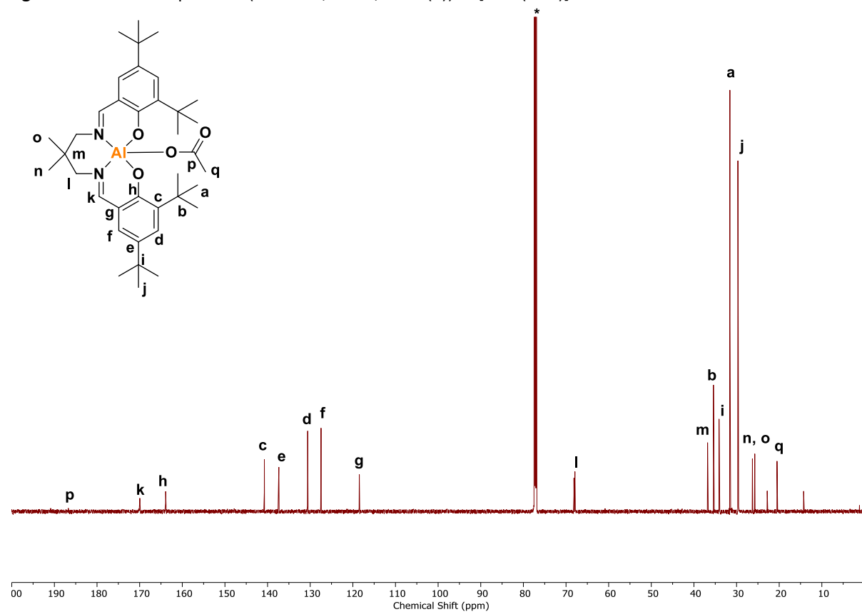
Figure S26. ^{13}\text{C} NMR Spectrum (176 MHz, 298 K, \text{CDCl}_3 (*)) of [\text{L}_{\text{sal}}\text{Al}(\text{OAc})] .
