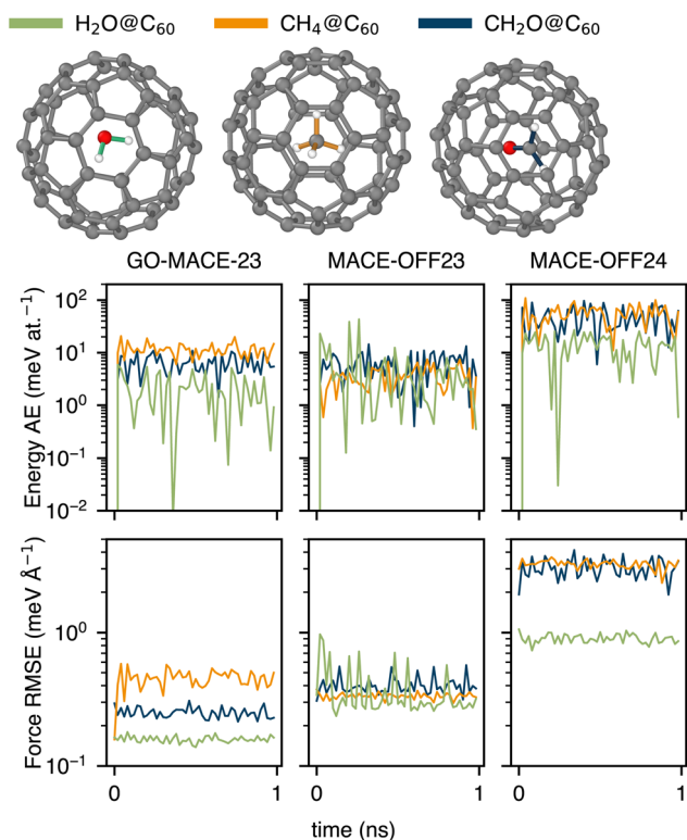
Fig. 7 Evolution of energy and force RMSE between GO-MACE-23 predictions and the corresponding DFT level of theory (left column), as well as between both MACE-OFF variants and their respective DFT levels of theory (middle and right columns). The errors are calculated from 1 ns trajectories at 500 K for H_2O , CH_4 , and CH_2O enclosed in a C_{60} fullerene. The trajectories are driven by GO-MACE-23.
