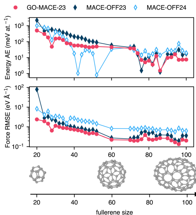
Fig. 6 Evolution of the prediction errors of the per-atom energy and forces of fullerenes, obtained from ref. 53, of sizes between 20 and 100 atoms computed with GO-MACE-23 and their corresponding DFT level of theory (red), and MACE-OFF and their corresponding DFT level of theory (dark and light blue). Similar to Fig. 5, lines represent the ML predictions, and the dashed lines represent the QM reference calculations. The rendered images show three fullerenes: C_{20} , C_{60} , and C_{100} .
