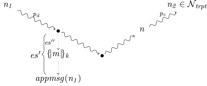
Figure 5.8: An illustration of Lemma 5.30.
