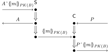
(e) A Hijack subpath for A \in \mathcal{T}_{names}^{reg} , P \in \mathcal{T}_{names}^{pen} .
