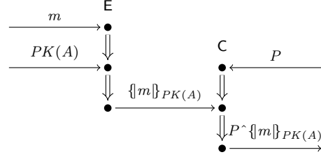
(b) A Send subpath for A \in \mathcal{T}_{names}^{reg} , P \in \mathcal{T}_{names}^{pen} .
