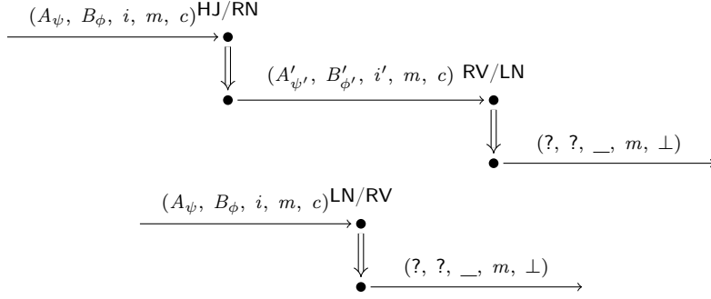
Figure 3.5: An illustration of one of the transformations of Lemma 3.13. This also illustrates Assumption 3.12 (2).
