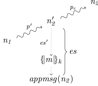
Figure 5.5: An illustration of Lemma 5.25.
