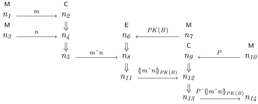
(b) A bundle containing a low-level Send penetrator subpath.
