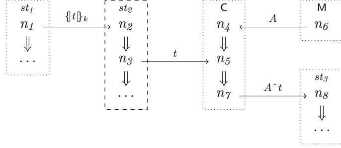
Figure 5.2: A bundle that does not satisfy Assumption 5.9 (4).
