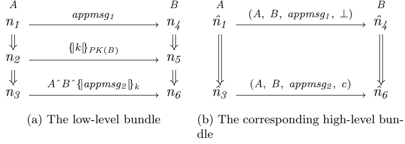
Figure 4.2: A low-level bundle that sends application-layer messages, one over the unprotected channel and another using a simple transport-layer protocol. The corresponding high-level bundle is also given.
