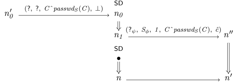
Figure 8.7: An illustration of the second case of Lemma 8.39 (where n is a penetrator node). In the above, \hat{c} = \widehat{\text{transport}(\mathcal{UP}^{C \rightarrow S})} .
