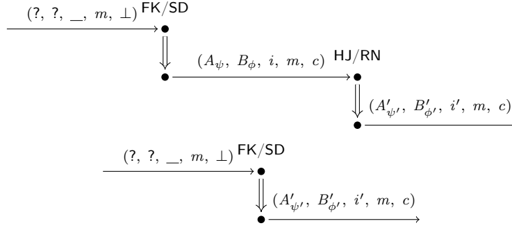
Figure 3.6: An illustration of one of the transformations of Lemma 3.13. This also illustrates Assumption 3.12 (3).
