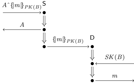
(c) A Learn subpath for A, B \in \mathcal{T}_{names}^{reg} , assuming that the penetrator obtains SK(B) somehow.
