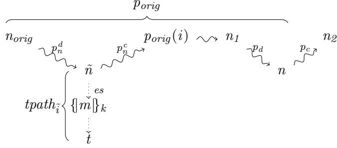
(b) The penetrator paths for Case (2).
