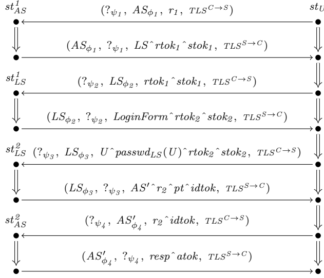
Figure 3.8: A graphical illustration of Proposition 3.23.
