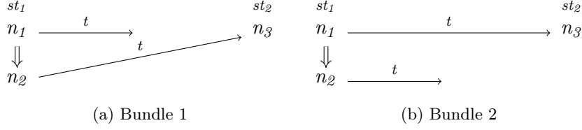
Figure 5.1: A bundle illustrating the problem with bundle equivalence.
