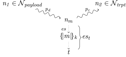
Figure 5.3: An illustration of Lemma 5.22. In the figure above dotted arrows indicate extraction paths, whilst wiggly lines arrows indicate, as usual, penetrator paths.
