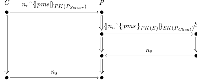
Figure 7.1: A example of a session where the penetrator causes a unilateral TLS session between C and P_{Server} to use the same encryption key as the bilateral TLS session between P_{Client} and S . The above uses a simplified version of TLS, rather than the full version.
