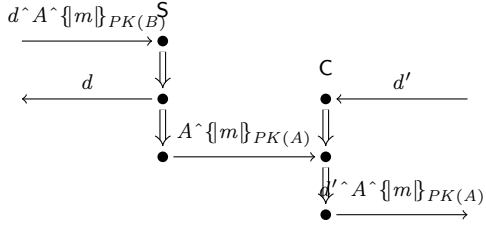
(f) A Transmit subpath, assuming that the running example has been augmented with nonces.
