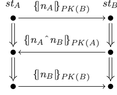
Figure 2.1: A graphical representation of a bundle containing one complete run of the Needham-Schroeder protocol.
