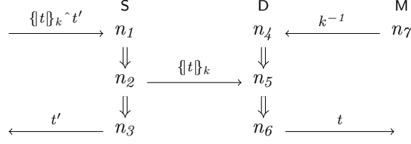
(a) A bundle containing a destructive penetrator path \langle n_1, n_2, n_5, n_6 \rangle .
