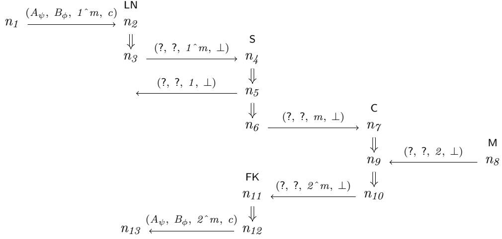
Figure 8.3: The penetrator path \langle n_1, n_2, n_3, n_4, n_6, n_7, n_{10}, n_{11}, n_{12}, n_{13} \rangle is a high-level penetrator renumber subpath for the running example. In the above, c is the bottom-transport-layer and it is assumed that it permits FK and LN strands (thus, it is not an \mathcal{AC} channel, in particular).
