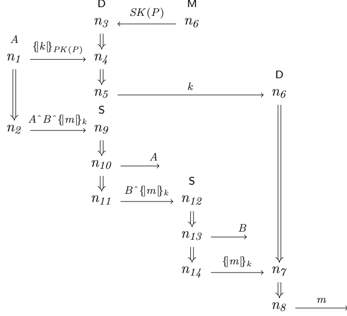
(a) A bundle containing a path that extracts the application-message from n_1 .
