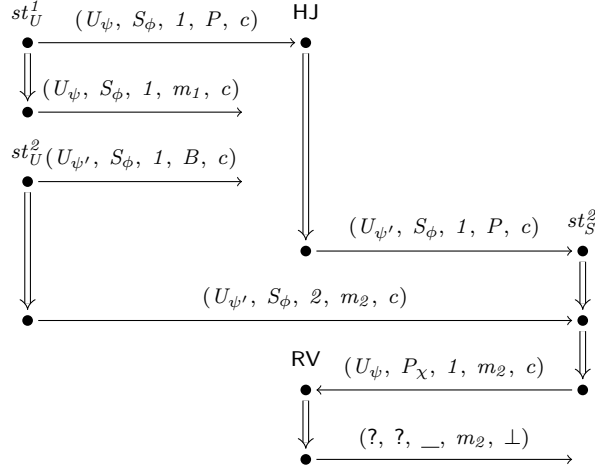
Figure 3.3: A graphical representation of a re-ascribe hijack attack by the penetrator, assuming that P \in \mathcal{T}_{names}^{pen} but B \in \mathcal{T}_{names}^{reg} . The above RV strand should not be allowed as the intended recipient was B , who is honest.
