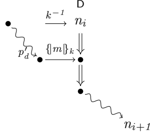
Figure 5.6: An illustration of Lemma 5.27.
