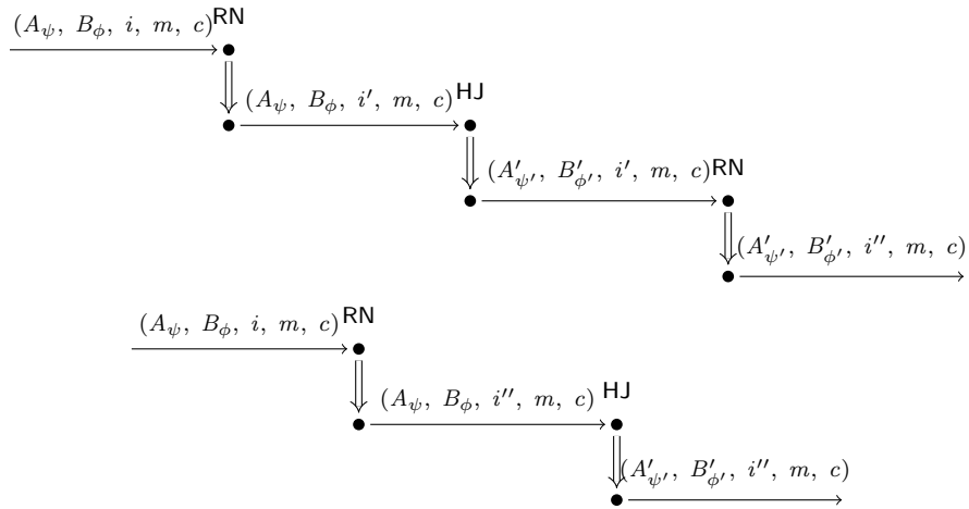
Figure 3.7: An illustration of one of the transformations of Lemma 3.13.
