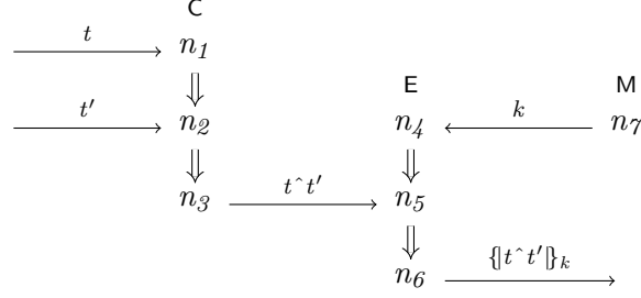
(b) A bundle containing a constructive penetrator path \langle n_1, n_3, n_5, n_6 \rangle .
