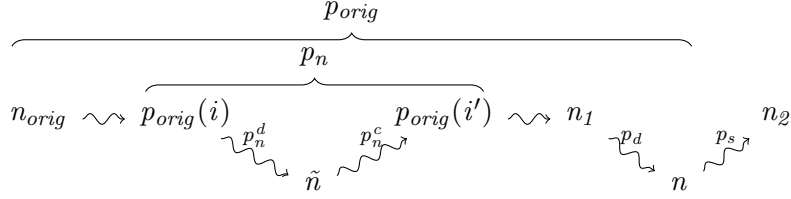
(a) The penetrator paths for Case (1).
