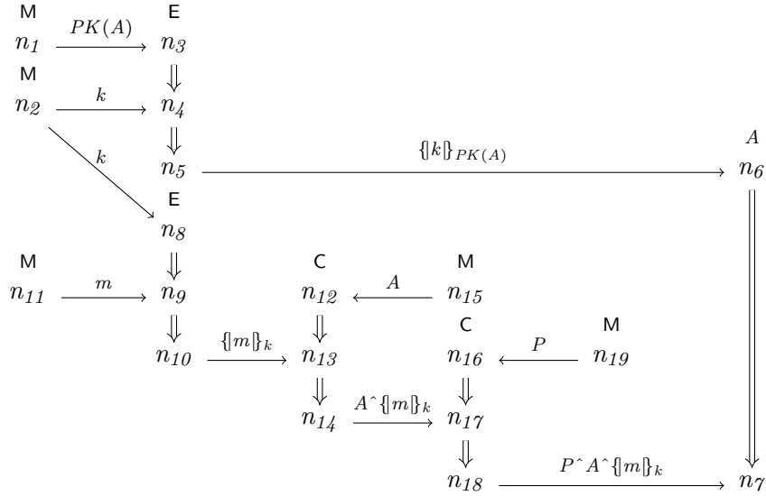
(b) A bundle containing a path that packages the application-message of n_1 .
