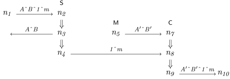
Figure 8.4: The penetrator path \langle n_1, n_2, n_4, n_9, n_{10} \rangle is a v_{B \rightarrow T} -Hijack subpath for the running example layered on a bottom transport-layer protocol that encodes (A?, B?, \_, am, c) as A^B^am (in the above am = 1^m ). Note that the subpath is also a v_{B \rightarrow M} -Hijack subpath and hence will be abstracted to a HJ strand in the middle strand space.
