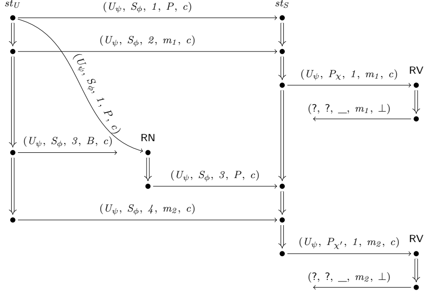
Figure 3.4: A graphical representation of a renumbering attack by the penetrator, assuming that P \in \mathcal{T}_{names}^{pen} but B \in \mathcal{T}_{names}^{reg} . The second RV strand should not be allowed as the intended recipient was B , who is honest.
