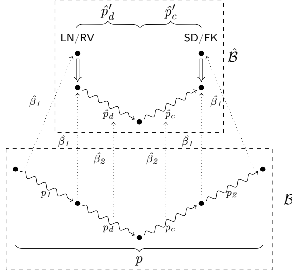
Figure 8.6: An illustration of the case of Proposition 8.20 where p is normal, and is not a normal v_{B \rightarrow M} -transport-layer penetrator subpath.
