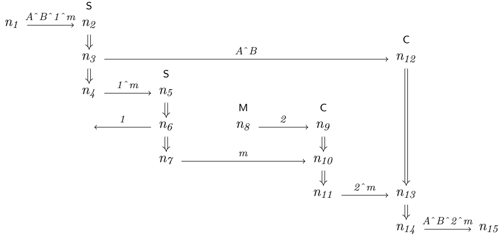
Figure 8.1: The penetrator path \langle n_1, n_2, n_4, n_4, n_5, n_7, n_{10}, n_{11}, n_{13}, n_{14}, n_{15} \rangle is a v_{B \rightarrow T} -Renumber subpath for the running example layered on a bottom transport-layer protocol that encodes (A?, B?, \_, m, c) as A^B m . The above bundle is a low-level version of the HL-Renumber penetrator subpath of Figure 8.3.
