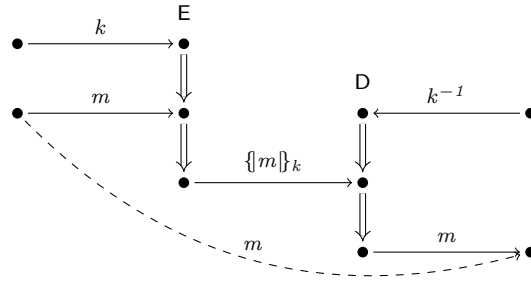
(a) Eliminating E-D redundancies.
