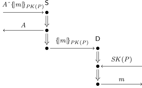
(a) A Receive subpath for A \in \mathcal{T}_{names}^{reg} , P \in \mathcal{T}_{names}^{pen} .
