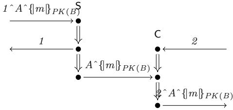
(g) A Renumber subpath, assuming that the running example has been augmented with sequence numbers.
