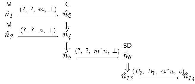
(a) The corresponding high-level bundle, including the high-level SD strand.
