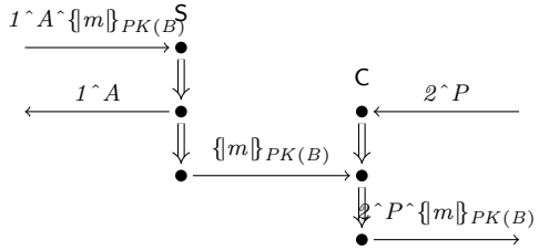
(h) A Hijack-Renumber subpath, assuming that the running example has been augmented with sequence numbers.
