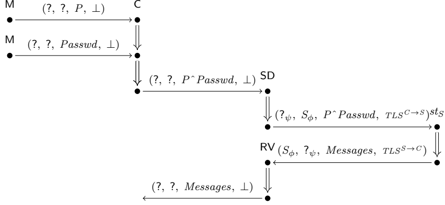
Figure 3.2: A figure illustrating how the penetrator can check his email, using the same protocol as Figure 3.1.
