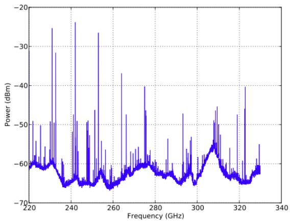
Fig. 8 Frequency spectrum with 220 – 330 GHz mixer. LO set to 198 GHz with the tripler in place. It can be seen that there are other significant harmonics present at frequencies well above 198 GHz.
