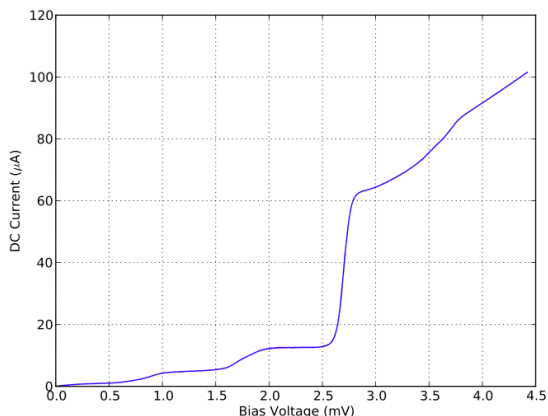
Fig. 2 A 252 GHz pumped I-V curve with a clean photon step structure.
