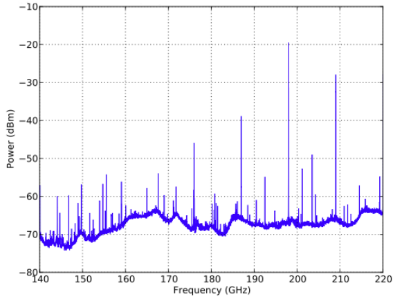
Fig. 7 Frequency spectrum with 140 – 220 GHz mixer. LO set to 198 GHz with the tripler in place. It can be seen that as well as the main tone at 198 GHz, there are other significant harmonics present which are separated by 11 GHz from the main tone.
