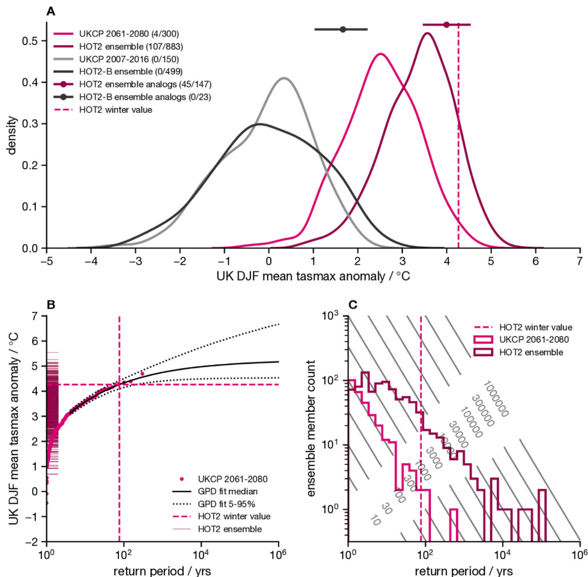
Fig. 4. As Fig. 3, but for the HOT2 winter.
