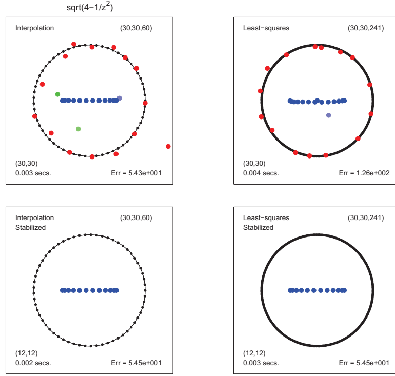
FIG. 6.8. Type (30,30) approximation of \sqrt{4-z^{-2}} , which has a branch cut [-1/2, 1/2] . Poles are placed along the branch cut. In the upper row the poles are far from symmetric, but the lower row shows the expected symmetries enforced by ratdisk . If |f(z) - r(z)| is measured just at grid points with |\text{Im}z| > 0.25 , the Err values shrink to 1.27\text{e}-5 , 2.51\text{e}-5 , 1.36\text{e}-5 , and 1.38\text{e}-5 .
