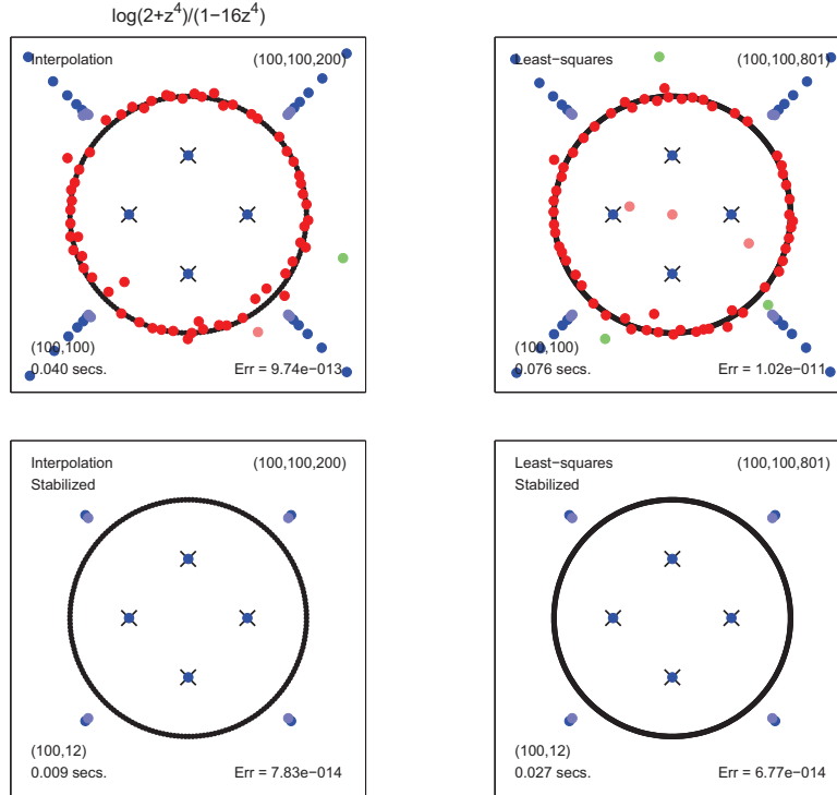
FIG. 6.3. For type (100,100) approximation of \log(2+z^4)/(1-16z^4) , there are many spurious poles in addition to the useful poles tracking the fourfold symmetric branch cuts. Note that as in Figs. 4.1 and 6.1, the spurious poles are not symmetric, even though the function is even. In the lower plots the symmetries are enforced and the type is reduced, with both \mu and \nu being divisible by 4 because of the fourfold symmetry.
