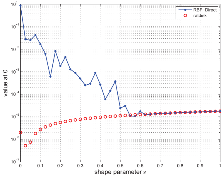
FIG. 8.1. Evaluation of an RBF interpolant through 80 data points by direct linear algebra (blue) and ratdisk (red circles). Rational least-squares approximation circumvents the ill-conditioning of the matrices in the linear algebra formulation.
