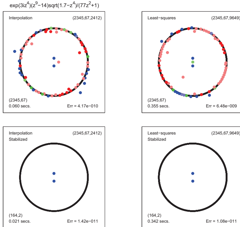
FIG. 6.7. Approximation of type (2345,67) to a complex function with two poles and four branch cuts. The polynomial degree is so high that the robust algorithm does not use the denominator at all except to capture the poles.
