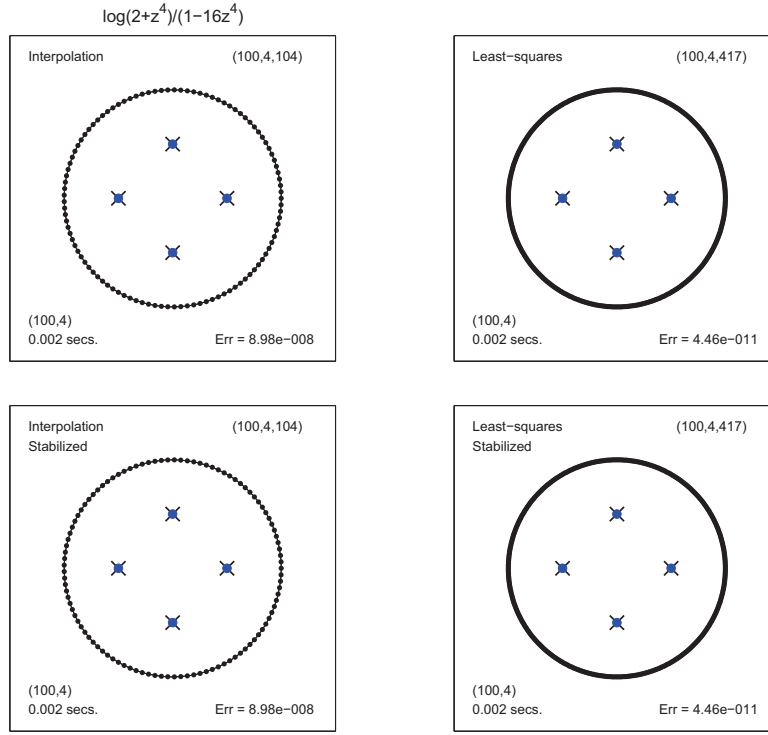
FIG. 6.2. Type (100,4) approximation of the even function \log(2+z^4)/(1-16z^4) . Here, since n has been specified as low as 4, the robustness features make no significant difference. The next figure shows what happens if n is increased.
