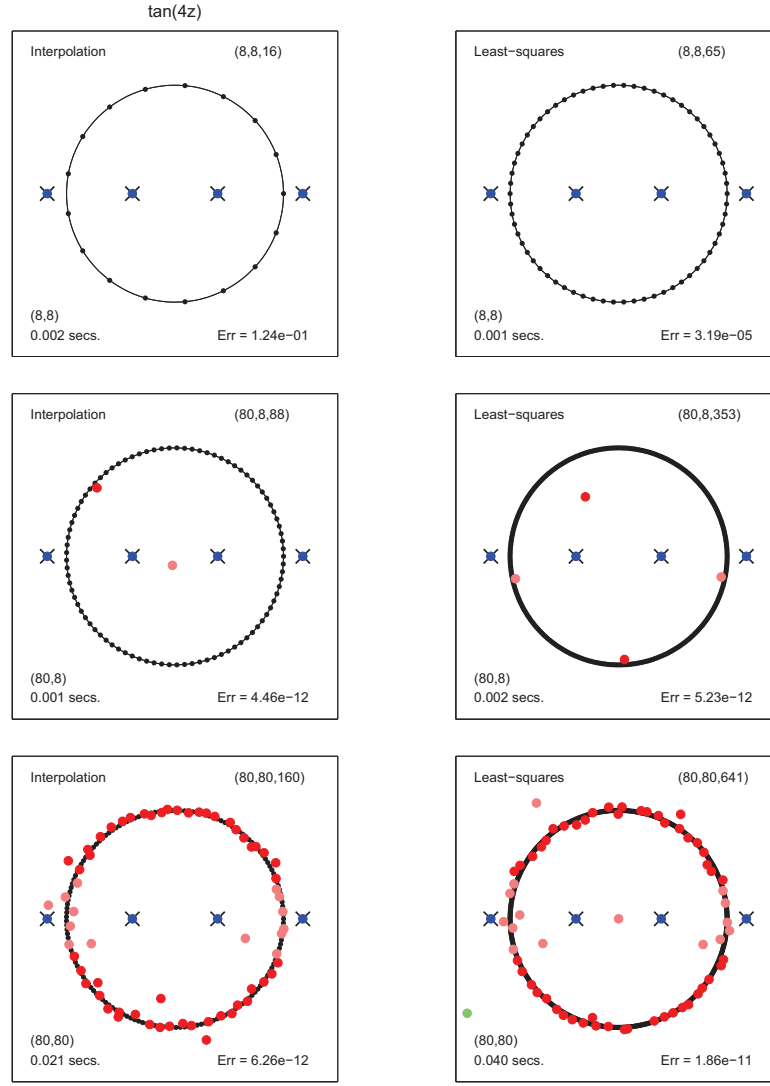
FIG. 4.1. Approximations to \tan(4z) by the algorithm of §3. For the type (8,8) approximations of the top row, both approximations successfully place four poles where one would expect them, and least-squares improves the quality of the fit by orders of magnitude. For type (80,8), in the second row, some spurious poles have appeared, and least-squares no longer makes much difference. With type (80,80), there are dozens of spurious poles clustering along the unit circle. In both the second and third rows, the spurious poles would make the Err measure infinite if the grid on which |f(z) - r(z)| was measured were infinitely fine, but the grid has just 7860 points and poles at arbitrary points with residues below 10^{-12} usually slip through undetected.
