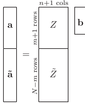
FIG. 3.1. Structure of the Toeplitz matrix equation \hat{\mathbf{a}} = \hat{Z}\mathbf{b} of (3.1), summarizing the notation of §3. In terms of function values rather than coefficients, this corresponds to equation (3.4), \hat{p}(z_j) = f_j q(z_j) for 0 \leq j \leq N . The least-squares problem is to minimize \|\hat{\mathbf{a}}\| subject to the constraint \|\mathbf{b}\| = 1 . The minimum value of \|\hat{\mathbf{a}}\| is \sigma_{\min} , the smallest singular value of \hat{Z} .
