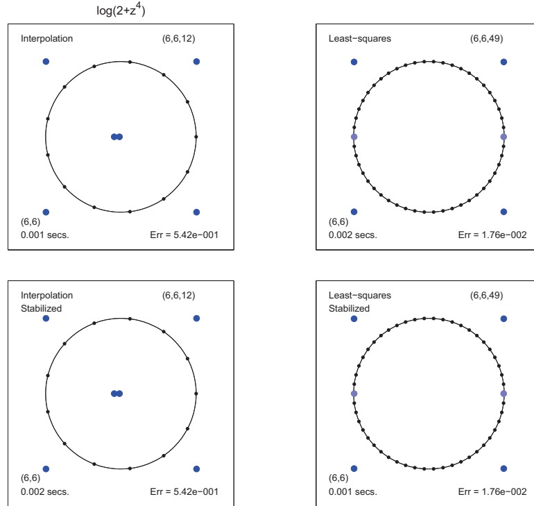
FIG. 6.9. Type (6,6) approximation of \log(2+z^4) . Notice that although f has four-fold symmetry, the exact type (\mu, \nu) is not divisible by 4, even in the least-squares computation of the bottom-right. This is because N = 49 is fairly small. For larger N one gets the expected symmetry, as shown in the final panel of Fig. 7.1.
