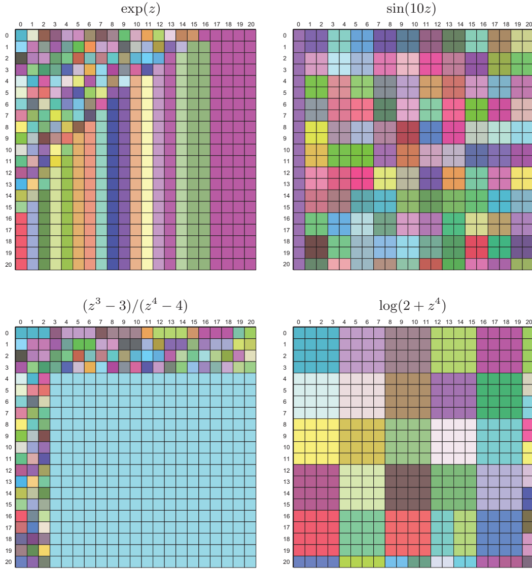
FIG. 7.1. Tables of linearized least-squares approximants to four functions, with m on the horizontal axis and n on the vertical axis. Each color corresponds to the exact type (\mu, \nu) of a ratdisk approximation computed with \text{tol} = 10^{-14} and N = 1023 , so that colors reveal blocks of identical entries or at least entries of identical exact types. For \exp(z) all the blocks are distinct until the function is resolved to machine precision, after which the denominator degrees are systematically reduced as far as possible. For the odd function \sin(10z) , 2 \times 2 square blocks appear in the table; because of the factor 10, this function is never resolved with m, n \leq 20 to machine precision, so no further degeneracies appear in the table. For (z^3 - 3)/(z^4 - 4) we get an infinite square block since the function is rational and thus resolved exactly for m \geq 3 and n \geq 4 . Finally, for \log(2 + z^4) we get 4 \times 4 blocks until m and n get large enough for the approximations to have accuracy close to machine precision; these anomalies go away if \text{tol} is increased to 10^{-12} .
