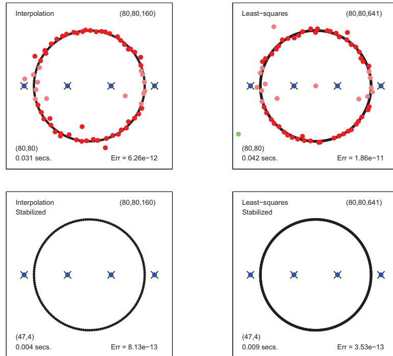
FIG. 6.1. Type (80,80) approximation of \tan(4z) again, now including robust ratdisk approximation in the second row. The spurious poles are gone. Note that the exact type has shrunk to (47,4), which is of the (odd,even) form appropriate in approximation of an odd function.
