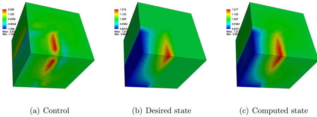
Figure 8.5: Control, desired state and state for time-dependent boundary control example with \beta = 10^{-6} , at the final time-step.
