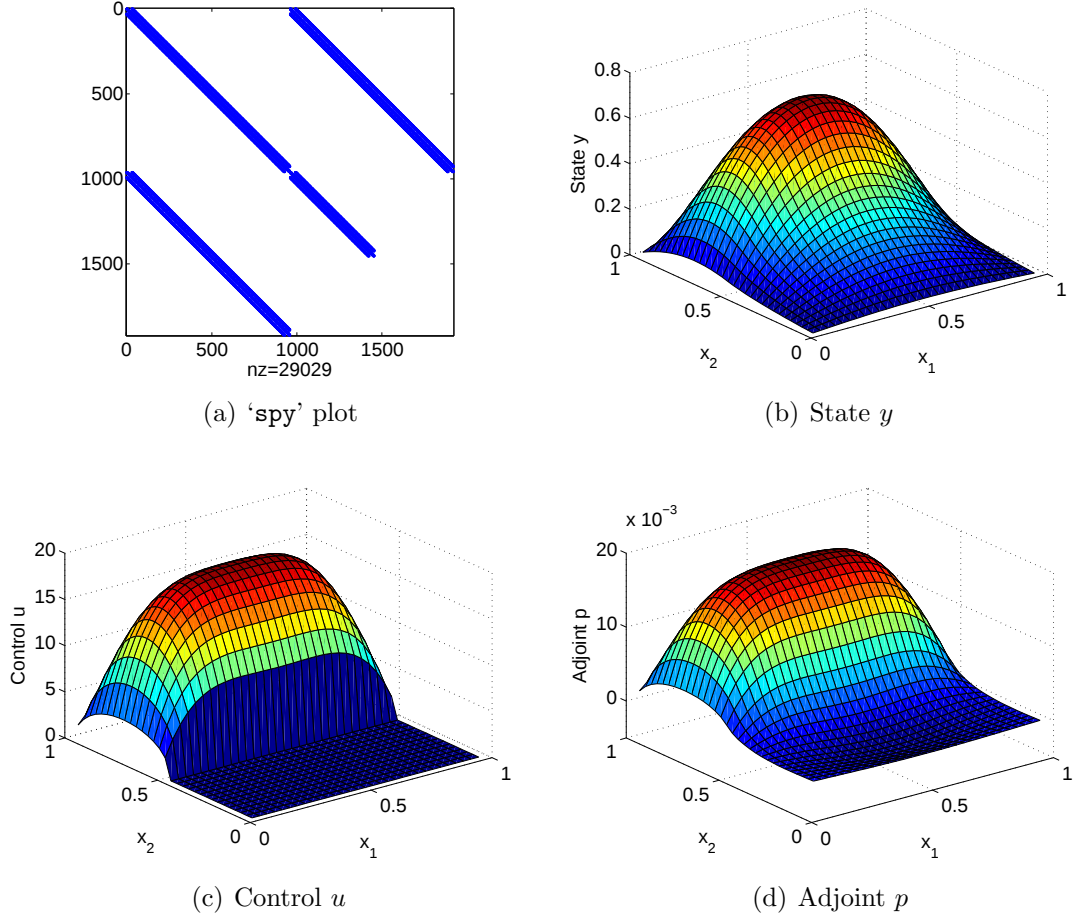
Figure 4.2: Plots of state, control and adjoint variables for the subdomain control test problem, with h = 2^{-5} and \beta = 10^{-3} , as well as a MATLAB 'spy' plot of the matrix within the system being solved.
