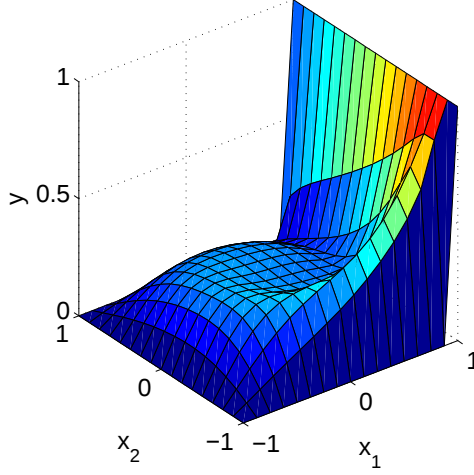
Figure 5.1: Finite element solution plot of (5.1)–(5.2), with \Omega = [-1, 1]^2 , h = 2^{-3} , \nu = \frac{1}{200} , f = 0 , g = 1 on x_1 = 1 and 0 otherwise, and \mathbf{w} = [\frac{1}{2}x_2(1-x_1^2), -\frac{1}{2}x_1(1-x_2^2)]^T , where \mathbf{x} = [x_1, x_2]^T denotes the spatial coordinates.
