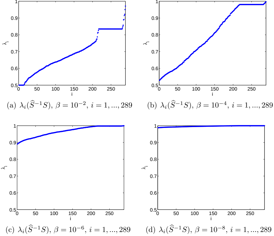
Figure 5.3: Spectra of \hat{S}^{-1}S for \beta = 10^{-2} , \beta = 10^{-4} , \beta = 10^{-6} and \beta = 10^{-8} , for an evenly spaced grid on \Omega = [-1, 1]^2 with h = 2^{-3} , \nu = \frac{1}{100} and \mathbf{w} = [\sin \frac{\pi}{6}, \cos \frac{\pi}{6}]^T .
