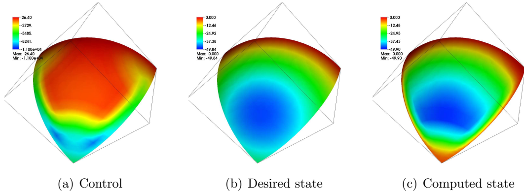
Figure 8.3: Control, desired state and state for the final-time case example with \beta = 10^{-4} , at the final time-step.
