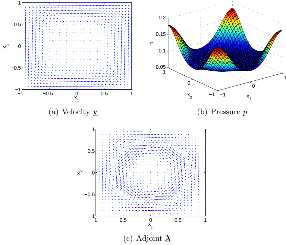
Figure 7.3: Solution plots for velocity \underline{v} , pressure p and adjoint \underline{\lambda} for Problem 2, with \beta = 1 and \text{Re} = 200 .
