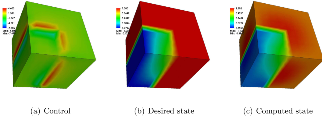
Figure 8.4: Control, desired state and state for time-dependent boundary control example with \beta = 10^{-6} , at the 10-th time-step.
