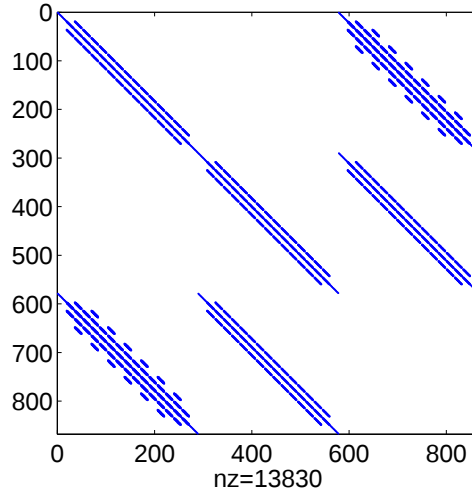
Figure 5.2: Sparsity pattern of the system (5.7) for Problem 1 as stated in Section 5.4, with h = 2^{-3} , \beta = 10^{-2} and \nu = \frac{1}{200} .
