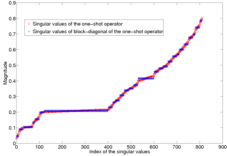
Figure 8.1: Singular values of the matrices \mathcal{K} and \bar{\mathcal{L}} for a small example.
