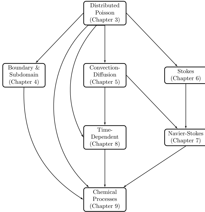
Figure 1.1: Flow chart outlining the problems of which we seek the numerical solution in this thesis, and their links to each other from a preconditioning point-of-view.
