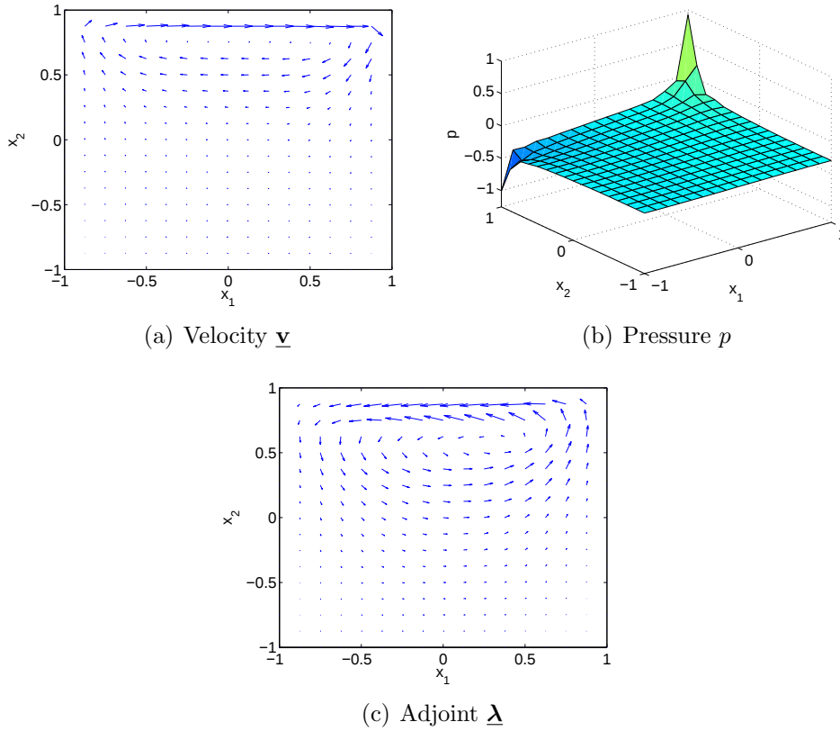
Figure 7.2: Solution plots for velocity \underline{\mathbf{v}} , pressure p and adjoint \underline{\lambda} for Problem 1, with \beta = 1 and \text{Re} = 100 .
