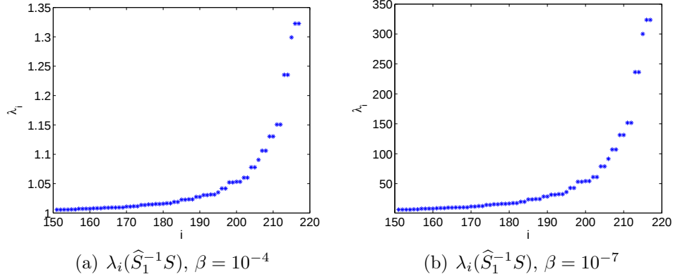
Figure 3.2: Illustrations of the intermediate eigenvalues of \hat{S}_1^{-1}S for \beta = 10^{-4} and \beta = 10^{-7} , for an evenly spaced grid on \Omega = [0, 1]^2 with h = 2^{-4} .
