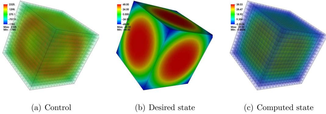
Figure 8.2: Control, desired state and state for the all-times case example with \beta = 10^{-4} , at the 15-th time-step.
