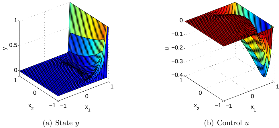
Figure 5.5: Solutions of state and control for Problem 2 using Q1 basis functions with \nu = \frac{1}{100} and \beta = 1 .
