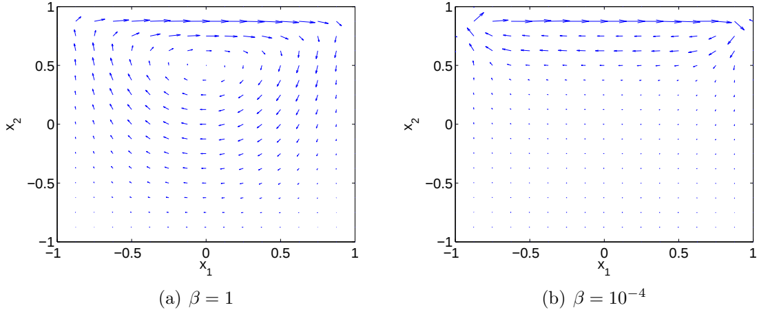
Figure 6.1: Plots of computed velocity solution to the test problem for different \beta . The value of h used here is 2^{-3} .
