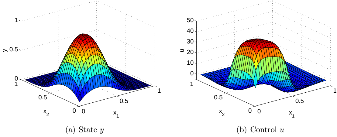
Figure 3.3: State and control solution to the numerical example in 2D, within \Omega \setminus \partial\Omega with axes x_1 and x_2 , with h = 2^{-5} and \beta = 10^{-4} .
