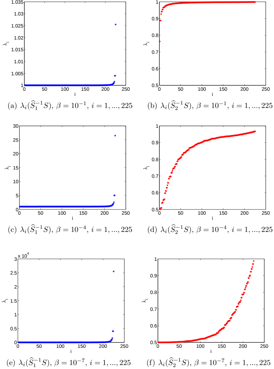
Figure 3.1: Spectra of \hat{S}_1^{-1}S [(a), (c), (e)] and \hat{S}_2^{-1}S [(b), (d), (f)] for \beta = 10^{-1} , \beta = 10^{-4} and \beta = 10^{-7} , for an evenly spaced grid on \Omega = [0, 1]^2 with h = 2^{-4} .
