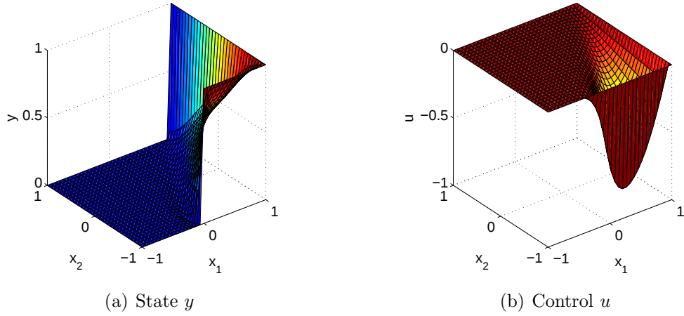
Figure 5.4: Solutions of state and control for Problem 1 using Q1 basis functions with \nu = \frac{1}{100} and \beta = 1 .
