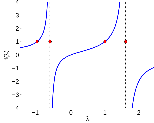
Figure 2.1: Plot of the function f(\lambda) = \frac{-\lambda}{\lambda^2 - \lambda - 1} . Marked are the values \lambda = -1, 1, \frac{1}{2}(1 \pm \sqrt{5}) .
