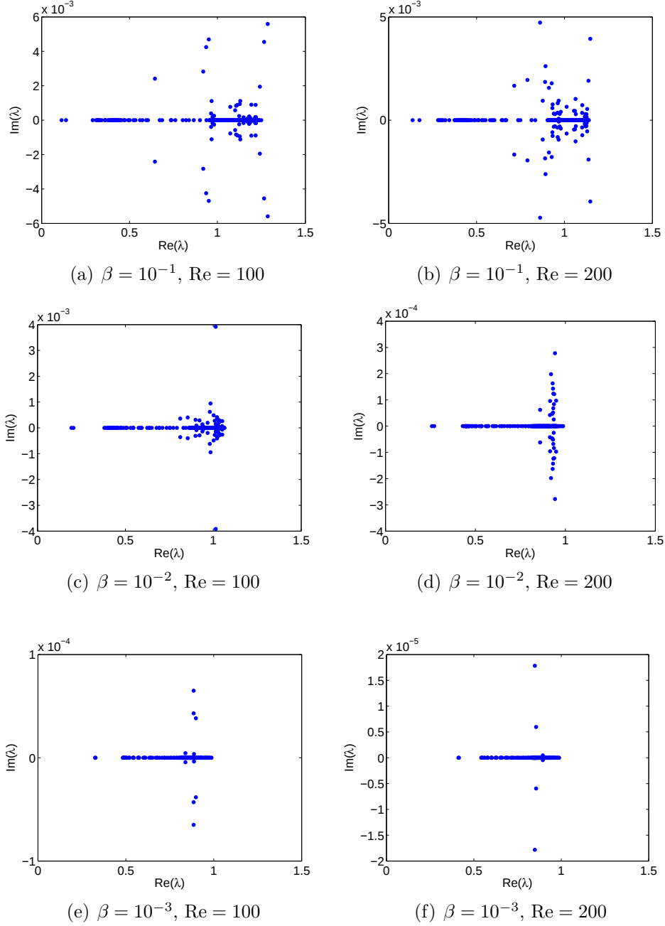
Figure 7.1: Spectra of \left(M_p^{-1}F_pM_p^{-1}F_p^TK_p^{-1} + \frac{1}{\beta}K_p^{-1}\right) \left[B\left(\mathbf{F}M^{-1}\mathbf{F}^T + \frac{1}{\beta}\mathbf{M}\right)^{-1}B^T\right] for \beta = 10^{-1}, 10^{-2}, 10^{-3} and \text{Re} = \frac{2}{\nu} = 100 and 200 , for the final Oseen step in the solution of Problem 1, on an evenly spaced grid on \Omega = [-1, 1]^2 with h = 2^{-4} .
