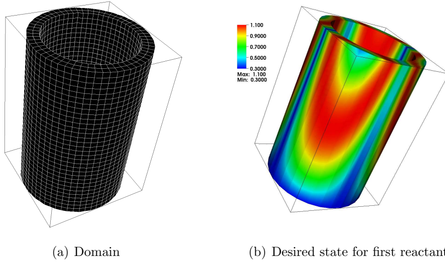
Figure 9.1: Cylindrical domain on which the first example was solved, and the desired state for the first reactant.
