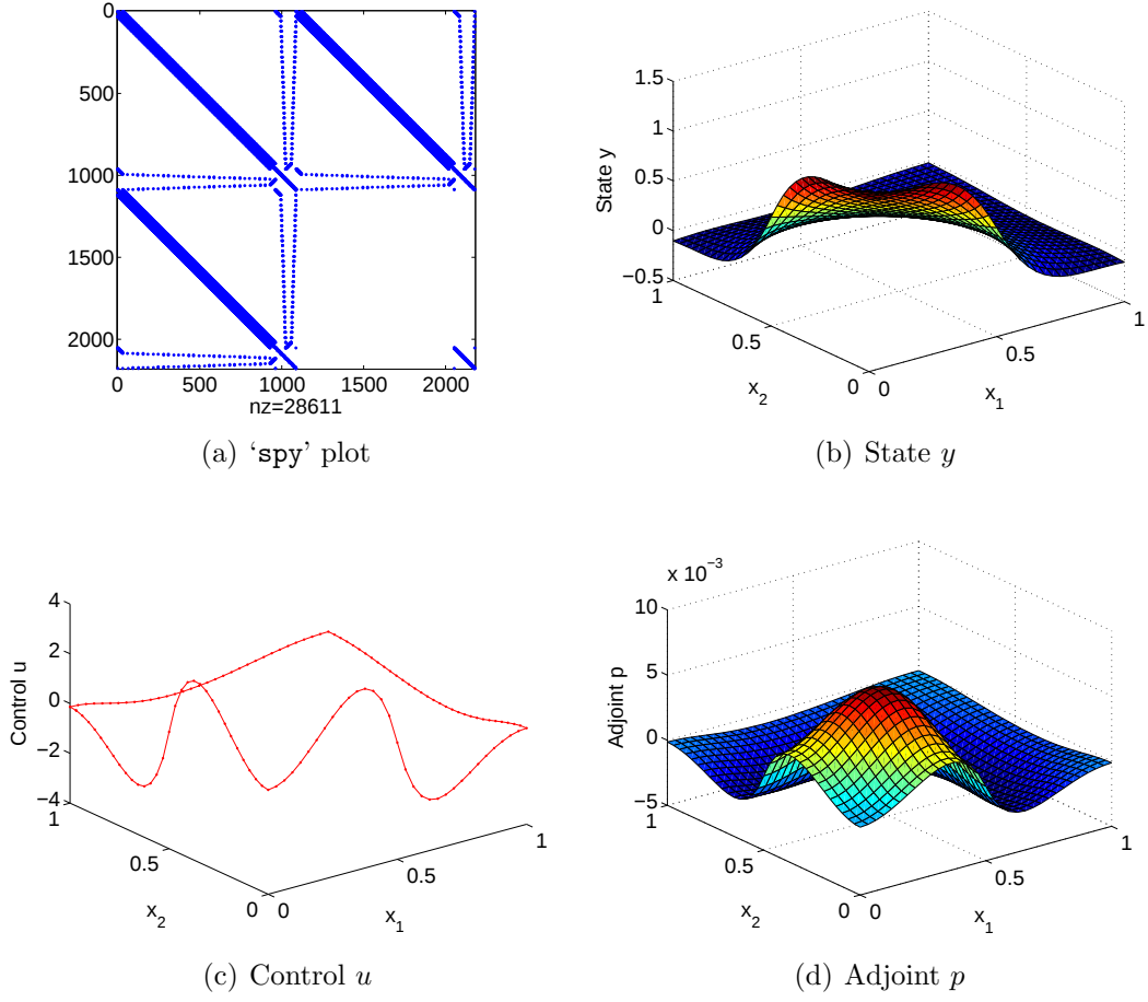
Figure 4.1: Plots of state, control and adjoint variables for the Neumann boundary control test problem, with h = 2^{-5} and \beta = 10^{-3} , as well as a MATLAB 'spy' plot of the matrix within the system being solved.
