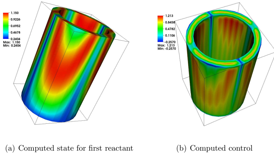
Figure 9.2: Computed state for the first reactant and computed control, at the 8-th time-step, with \alpha_u = \alpha_v = 1 and \alpha_c = 10^{-5} .
