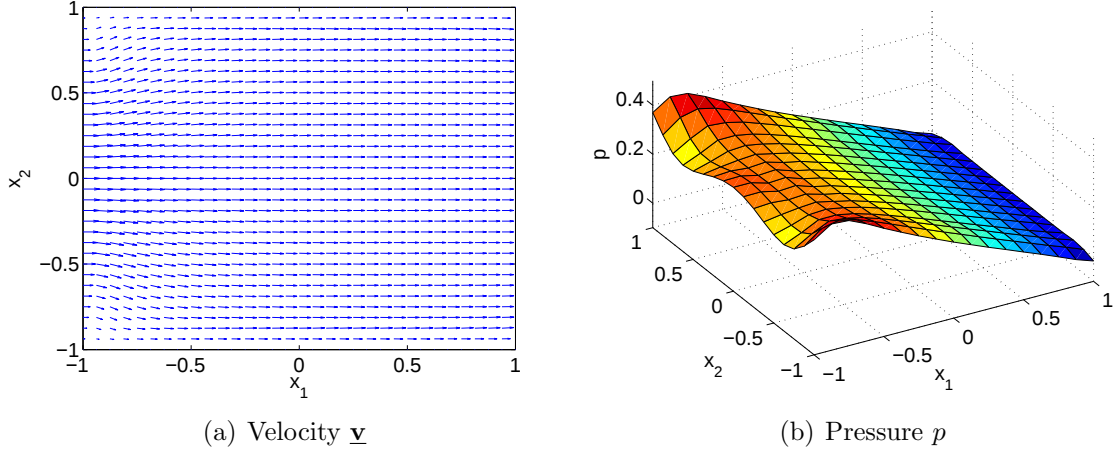
Figure 7.4: Solution plots for velocity \underline{v} and pressure p for Problem 3, with \beta = 10^{-2} and \text{Re} = 100 .
