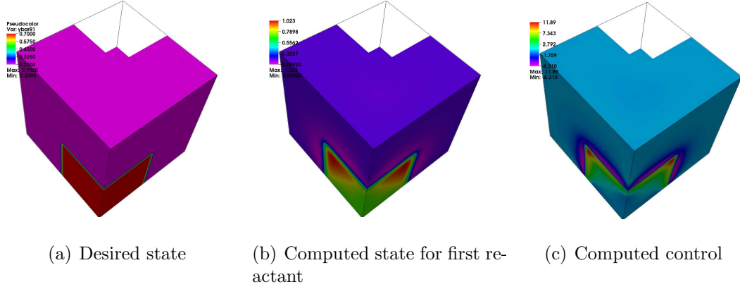
Figure 9.3: Desired and computed states for the first reactant and computed control, at the 8-th time-step, with \alpha_u = \alpha_v = 1 and \alpha_c = 10^{-5} .
