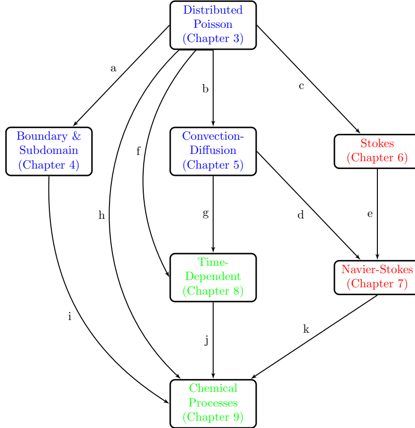
Figure 10.1: Flow chart outlining the problems of which we have sought the numerical solution in this thesis, and their links to each other from a preconditioning point-of-view.
