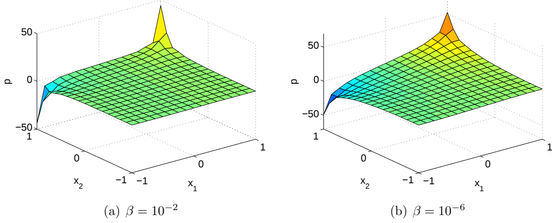
Figure 6.2: Plots of computed pressure solution to the test problem for different \beta . The value of h used here is 2^{-4} .
