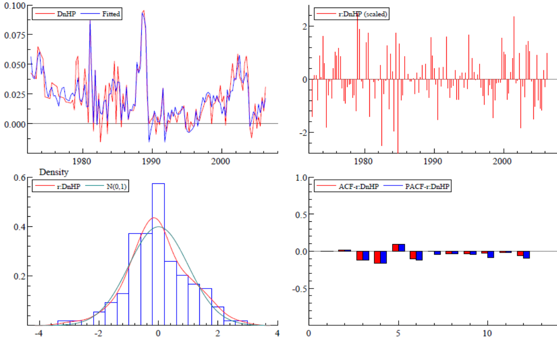
Chart panel 5 : Residual analysis of Model B
